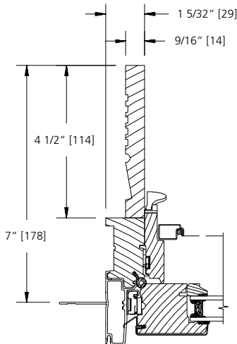
7" WALL
