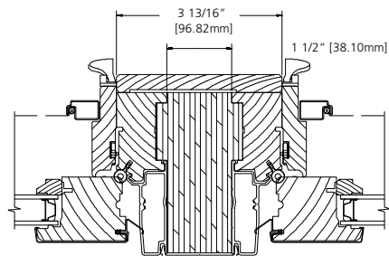
1 1/2" WOOD SPREAD MULLION
