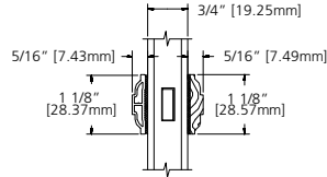
1 1/8" SDL
