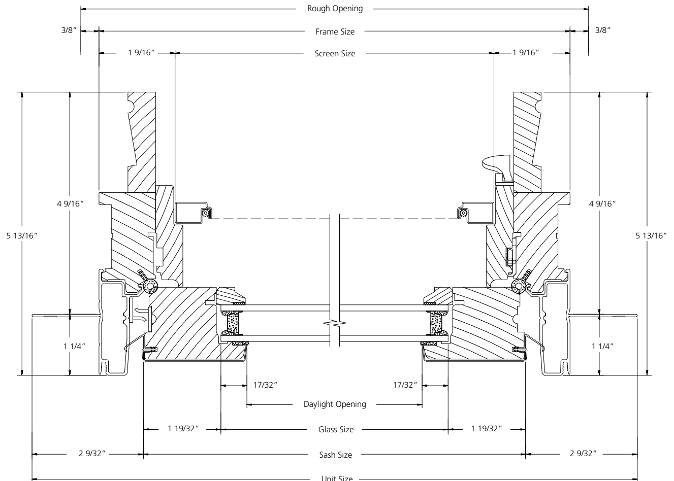
HORIZONTAL SECTION
