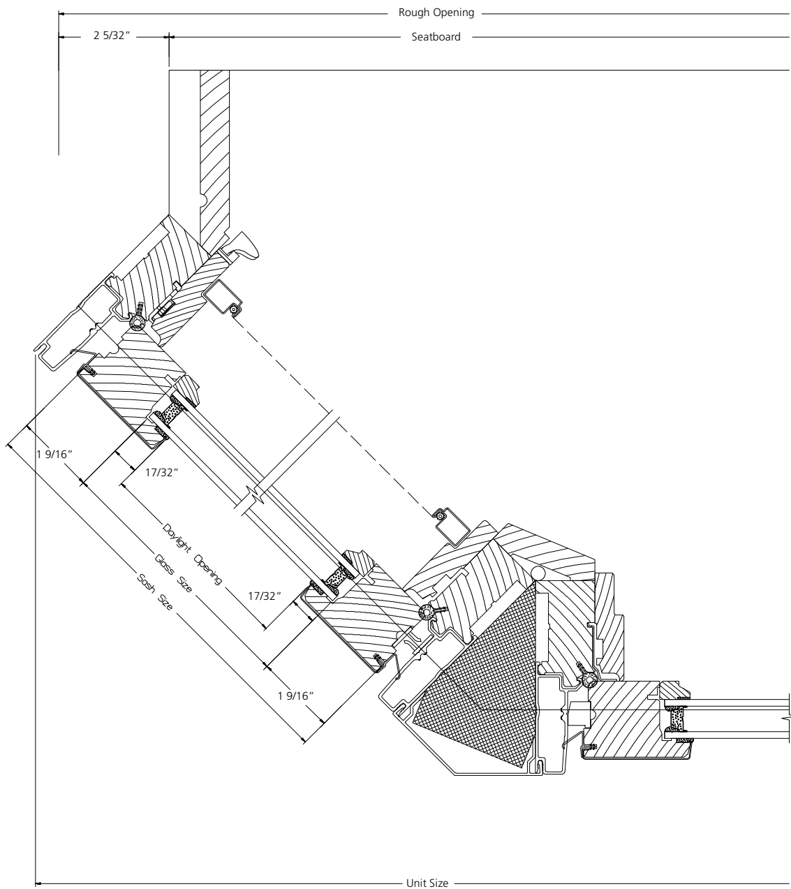
HORIZONTAL SECTION
