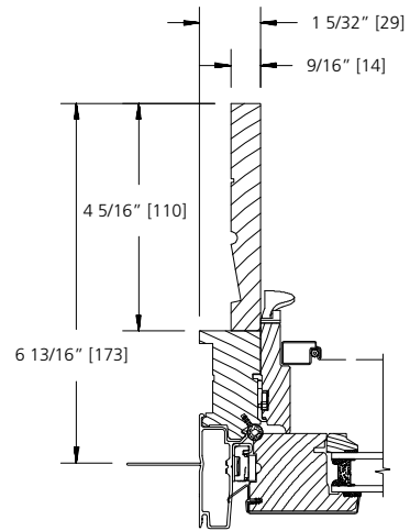
6 13/16" WALL
