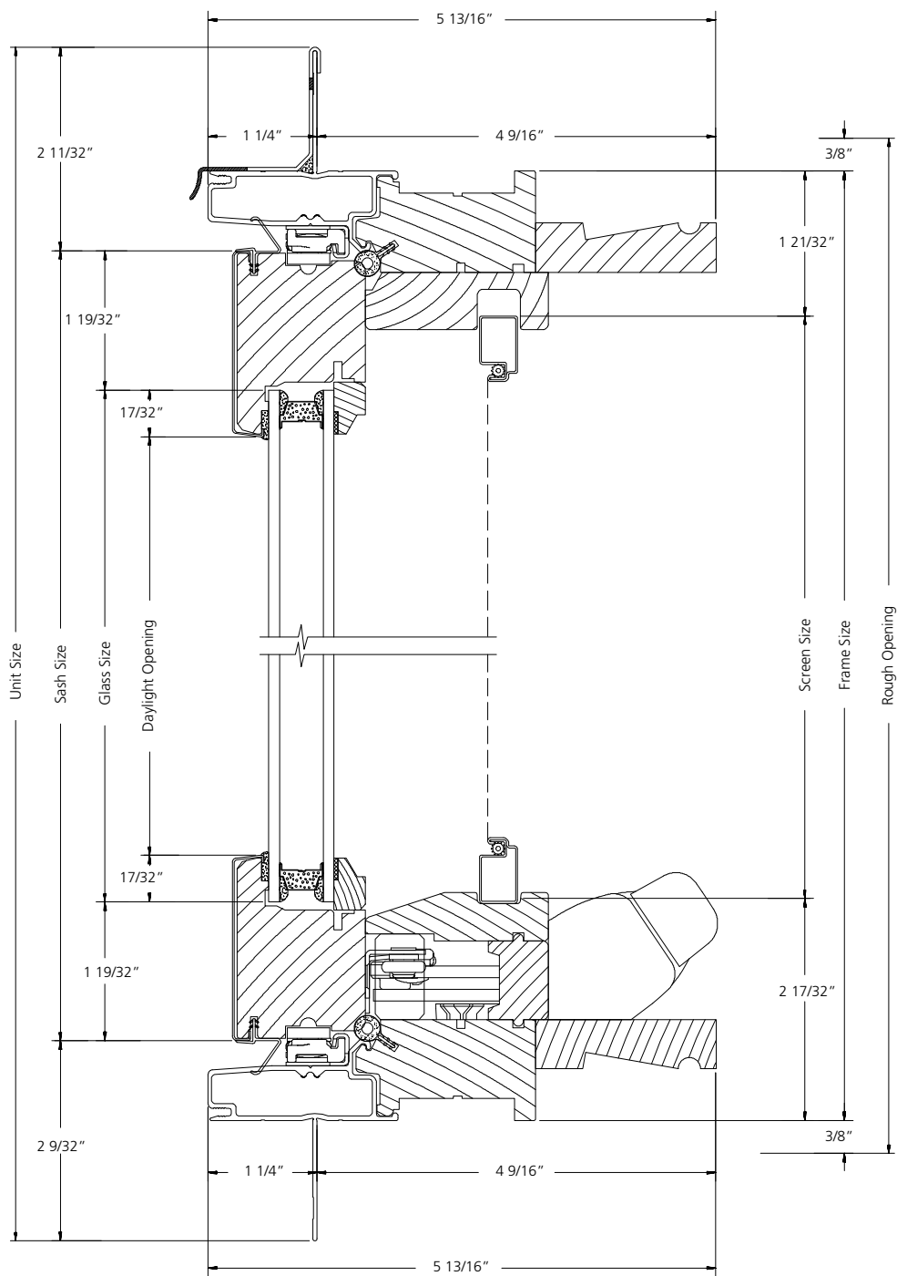
VERTICAL SECTION
