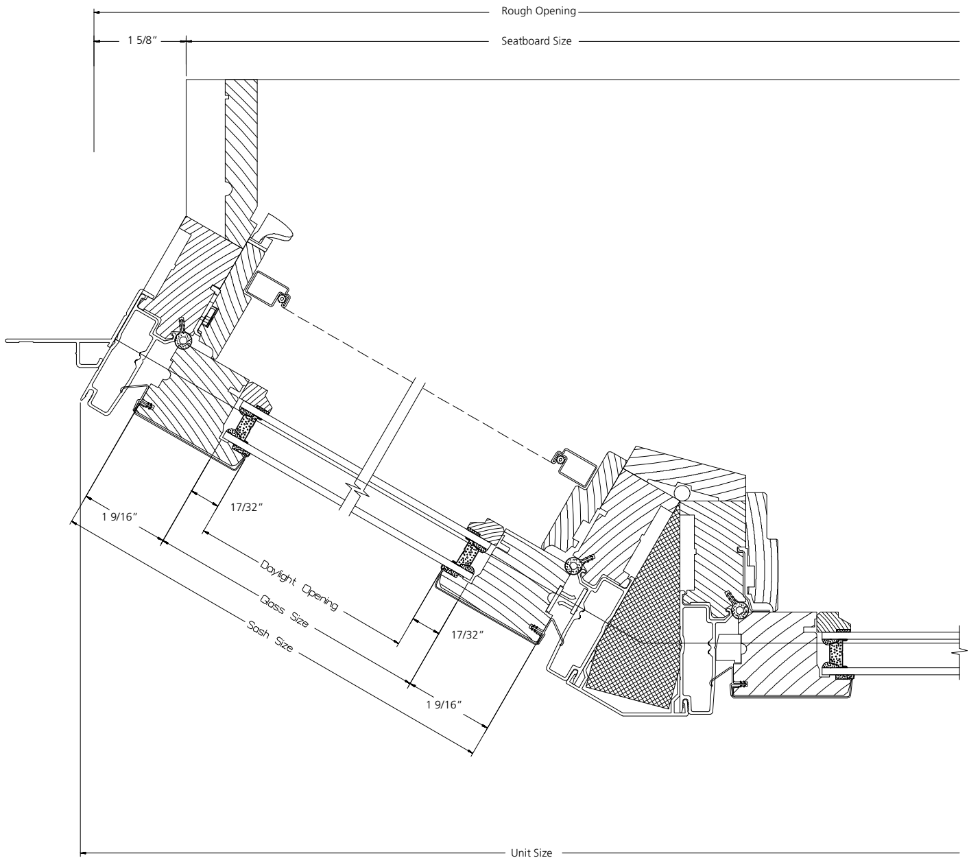
HORIZONTAL SECTION
