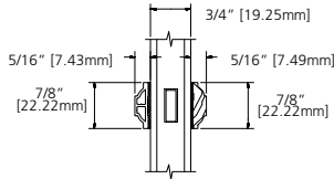
7/8" SDL
