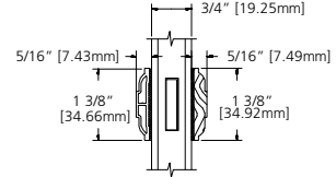
1 3/8" SDL
