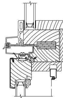
DIRECT SET RADIUS OVER CASEMENT
