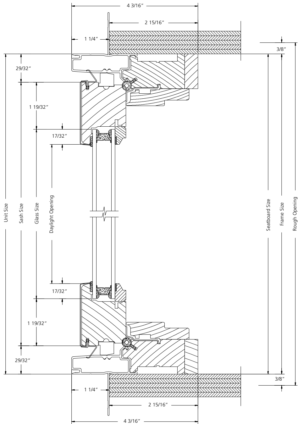
VERTICAL SECTION
