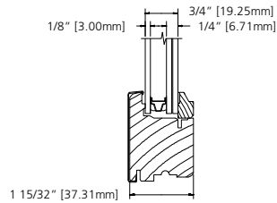
LAMINATED INSULATED CLEAR OR LOW-E 3.0mm//6.7mm LAMINATE
