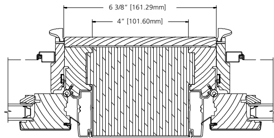
4" WOOD SPREAD MULLION
