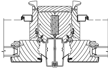
TWIN OPERATING CASEMENT
