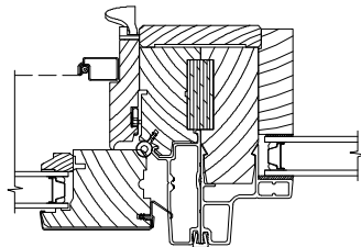
CASEMENT NEXT TO DIRECT SET
