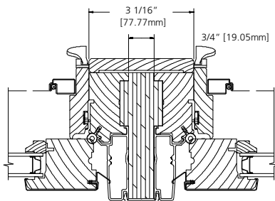
3/4" WOOD SPREAD MULLION
