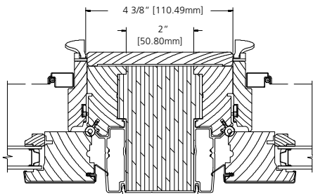
2" WOOD SPREAD MULLION
