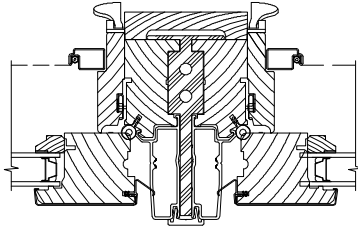
1/4" ALUMINUM REINFORCEMENT
