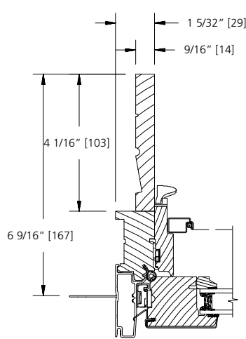
6 9/16" WALL
