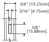
5/8" GRILLE
