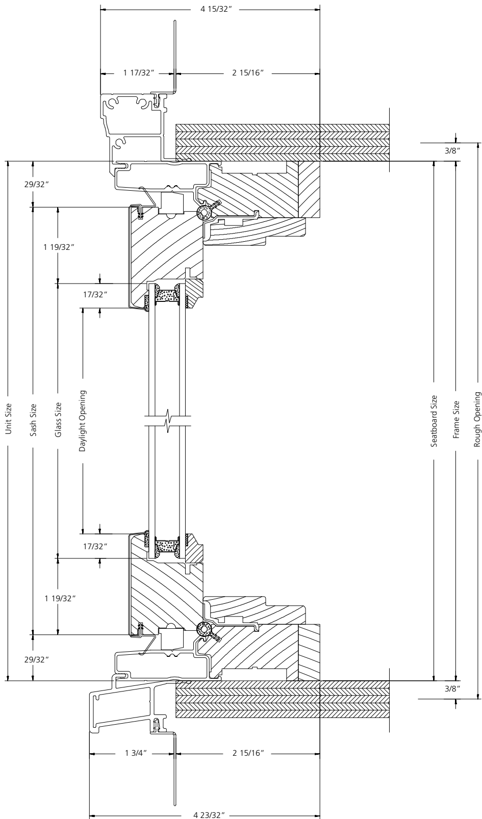
VERTICAL SECTION
