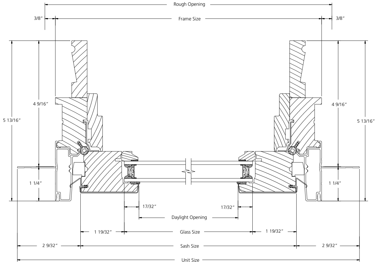
HORIZONTAL SECTION
