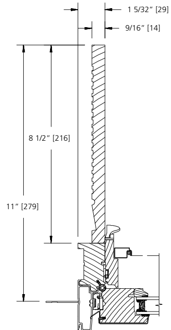
11" WALL
