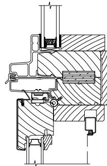
DIRECT SET GEOMETRIC OVER CASEMENT
