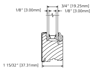
INSULATED GLASS
