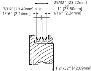
TRIPLE GLAZE INSULATED
