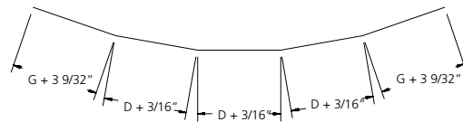
EXTREME PERIMETER
