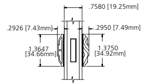
1 3/8" SDL
