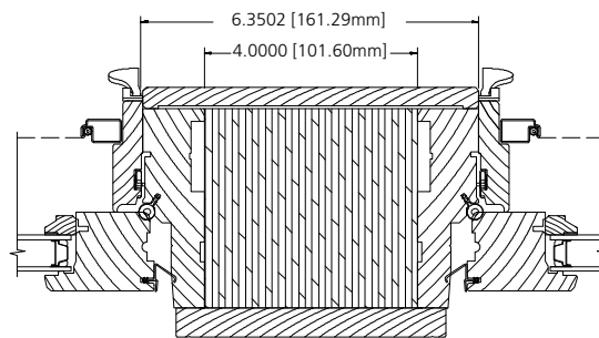
4" WOOD SPREAD MULL
