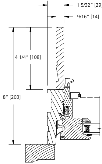
8" WALL
