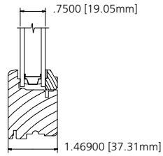
INSULATED GLASS
