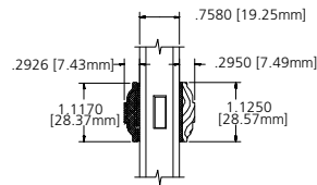
1 1/8" SDL
