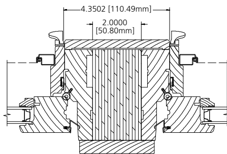
2" WOOD SPREAD MULL
