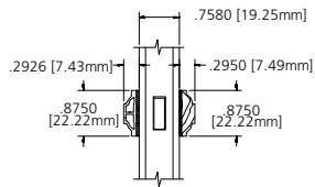
7/8" SDL
