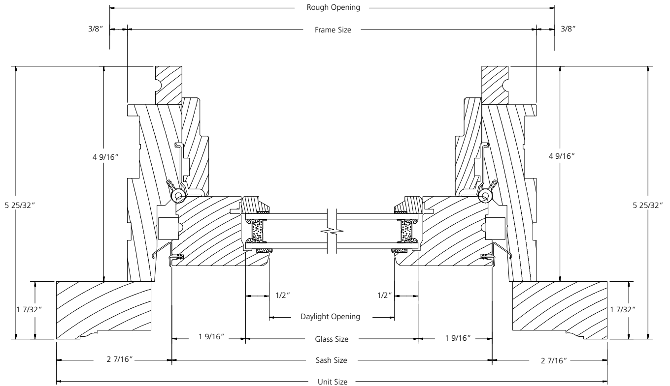
HORIZONTAL SECTION
