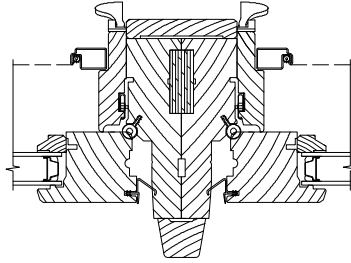
TWIN OPERATING CASEMENT
