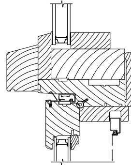
DIRECT SET RADIUS OVER CASEMENT
