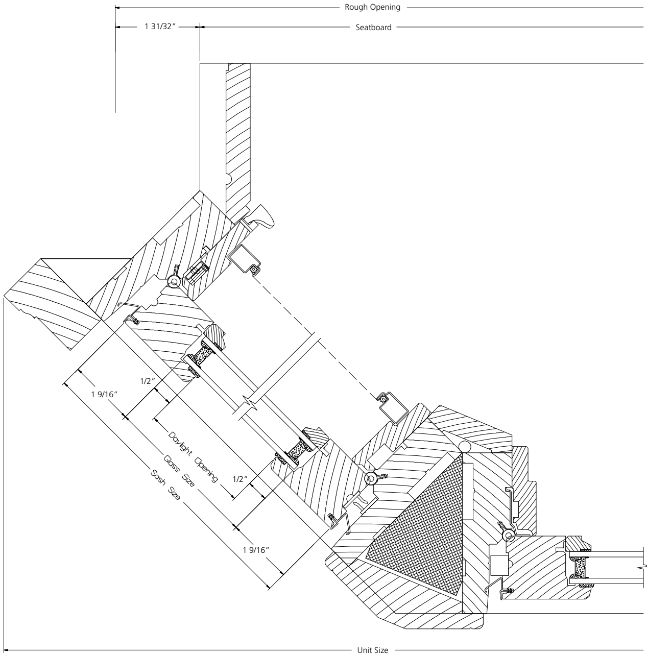
HORIZONTAL SECTION
