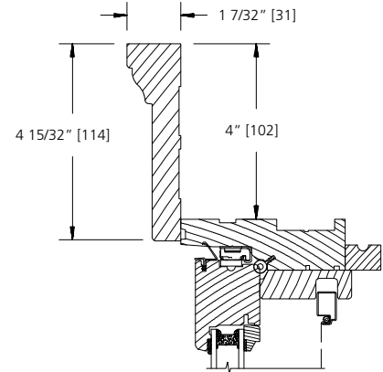
1 X 4 BACK BAND
