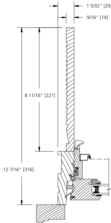
12 7/16" WALL
