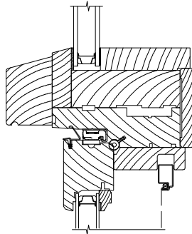
DIRECT SET GEOMETRIC OVER CASEMENT
