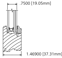
LAMINATED INSULATED CLEAR OR LOW-E
