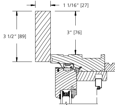
FLAT CASING
