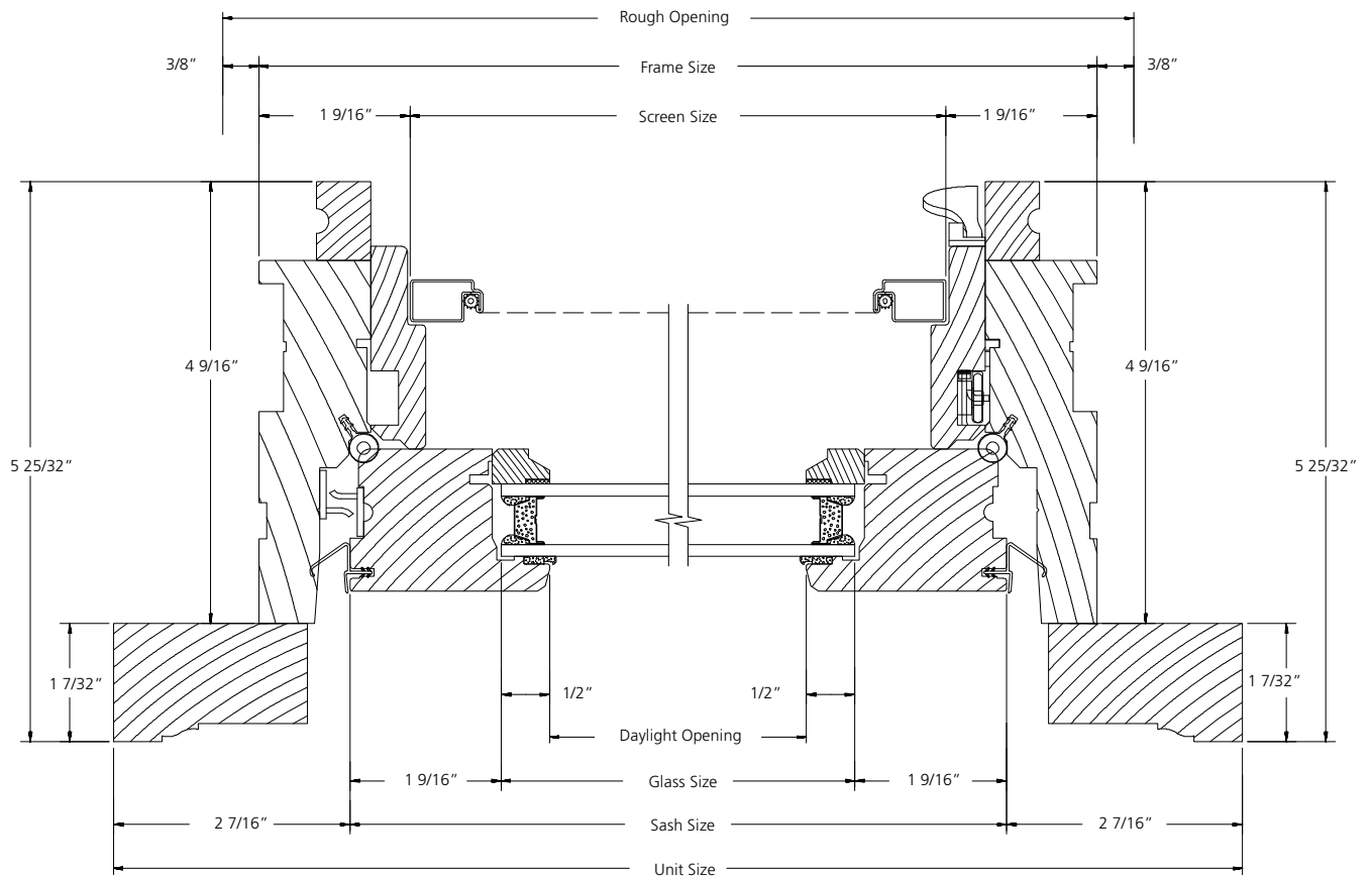
HORIZONTAL SECTION
