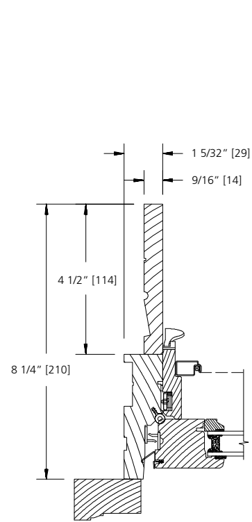
8 1/4" WALL
