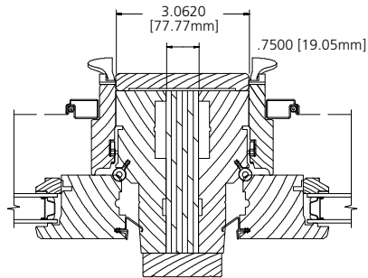
3/4" WOOD SPREAD MULL
