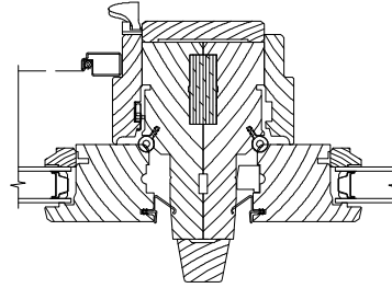
OPERATING CASEMENT NEXT TO CASEMENT PICTURE
