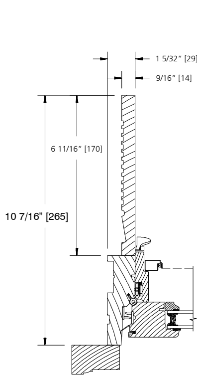
10 7/16" WALL
