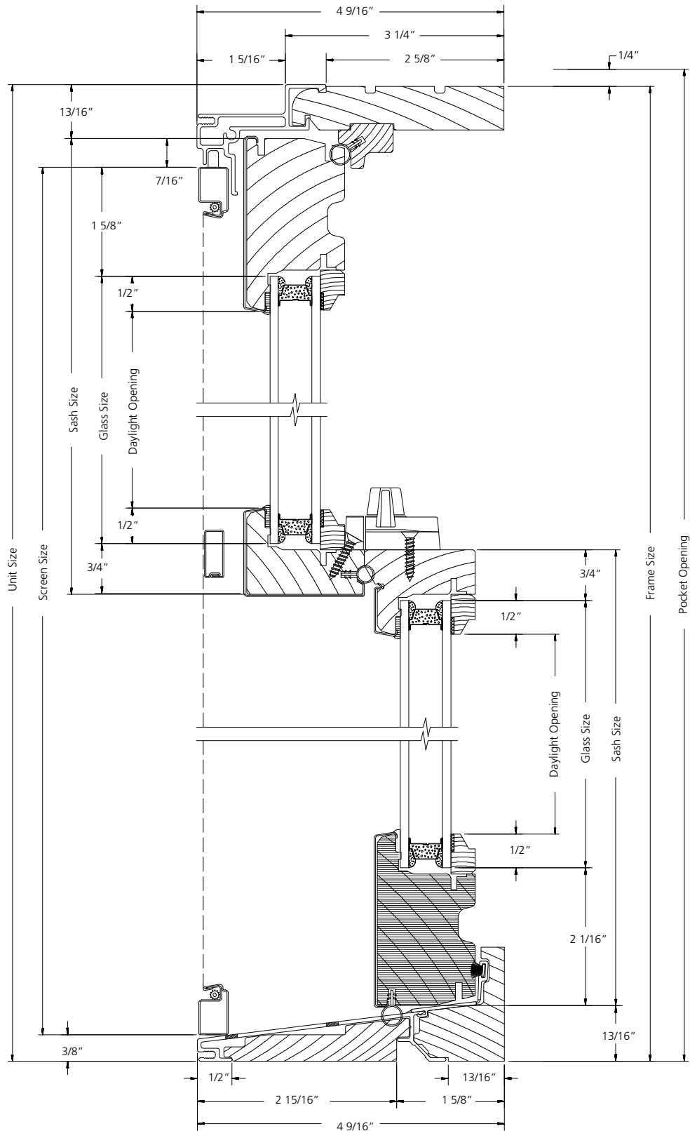
VERTICAL SECTION
