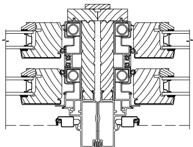
TWIN OPERATING DOUBLE HUNG
