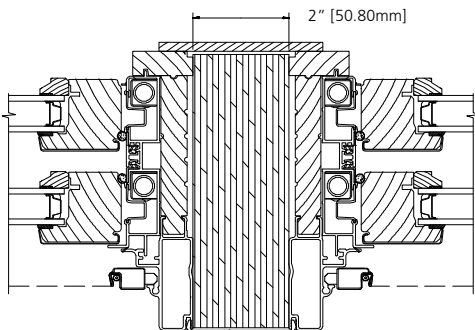
2" WOOD SPREAD MULL
