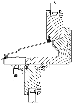
DOUBLE HUNG TRANSOM OVER DOUBLE HUNG
