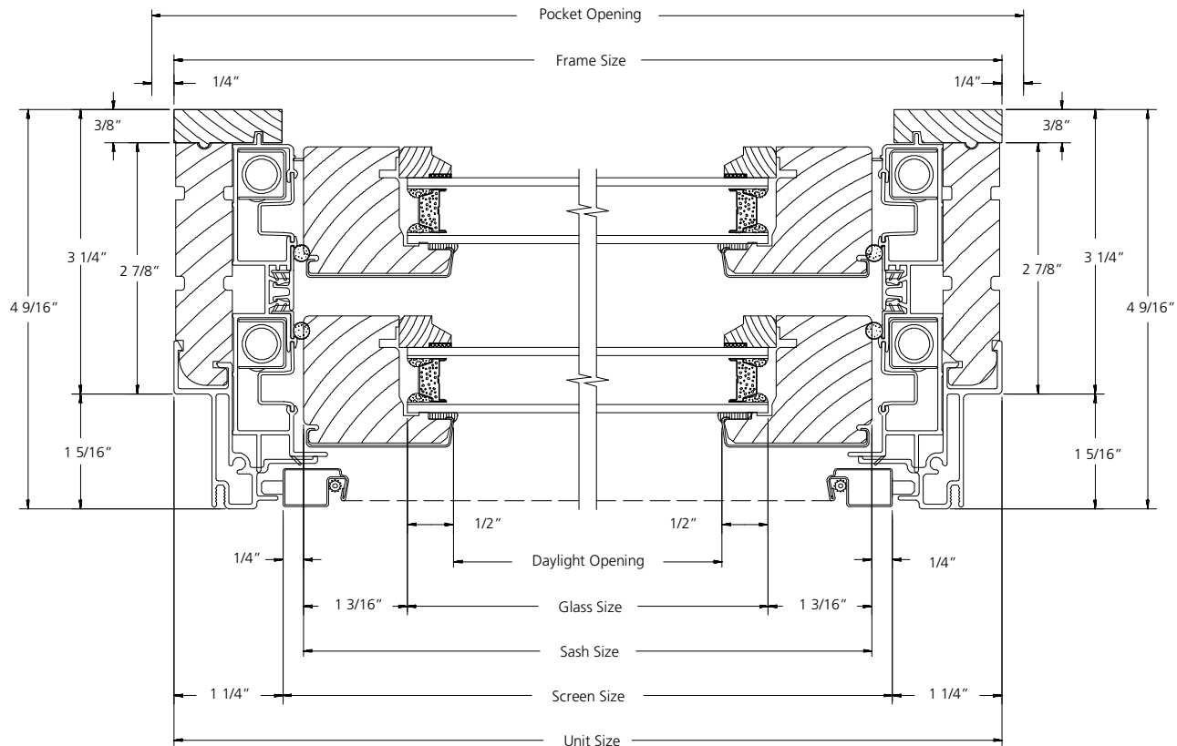
HORIZONTAL SECTION
