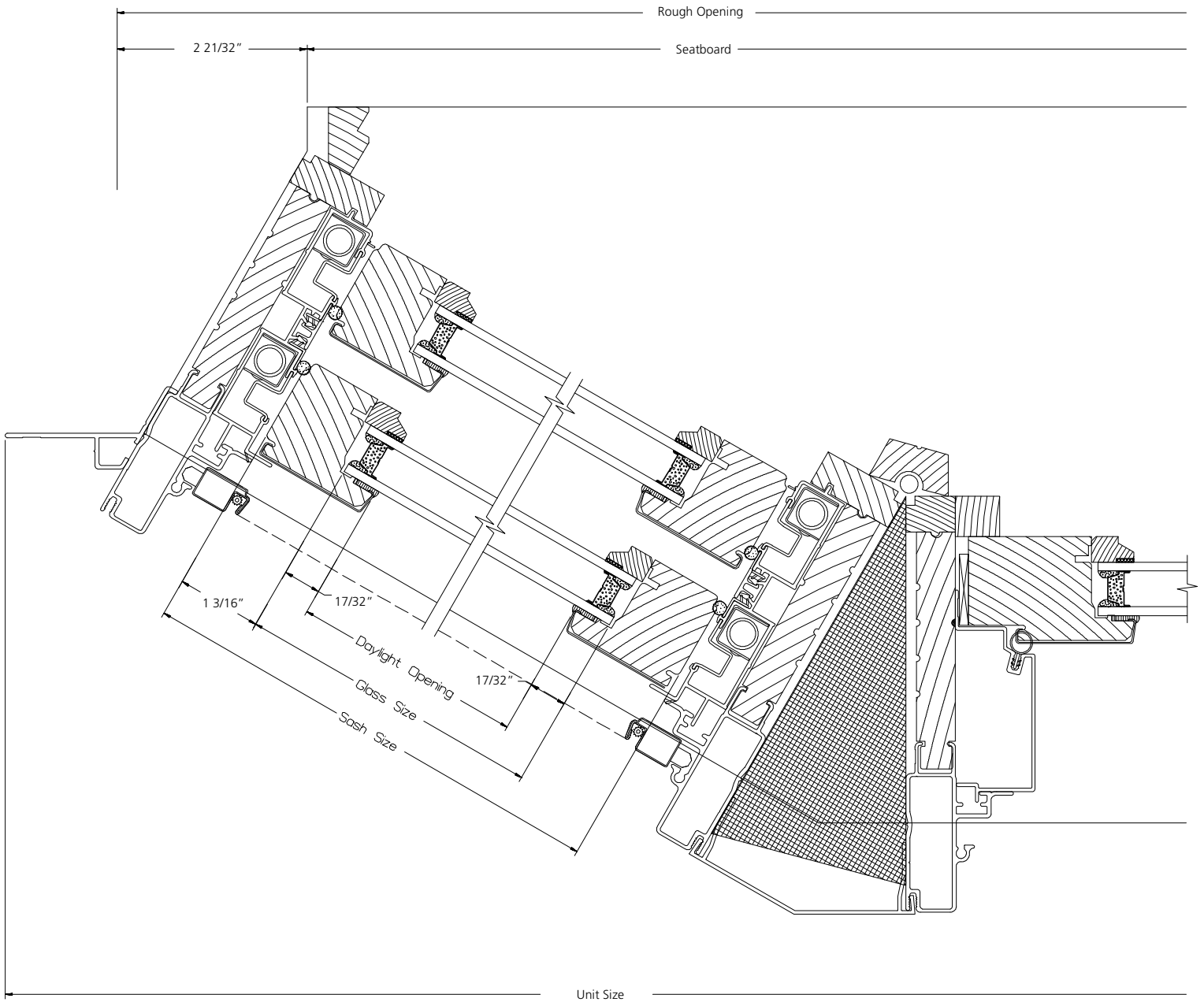
HORIZONTAL SECTION
