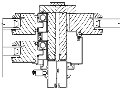
OPERATING DOUBLE HUNG NEXT TO DOUBLE HUNG PICTURE
