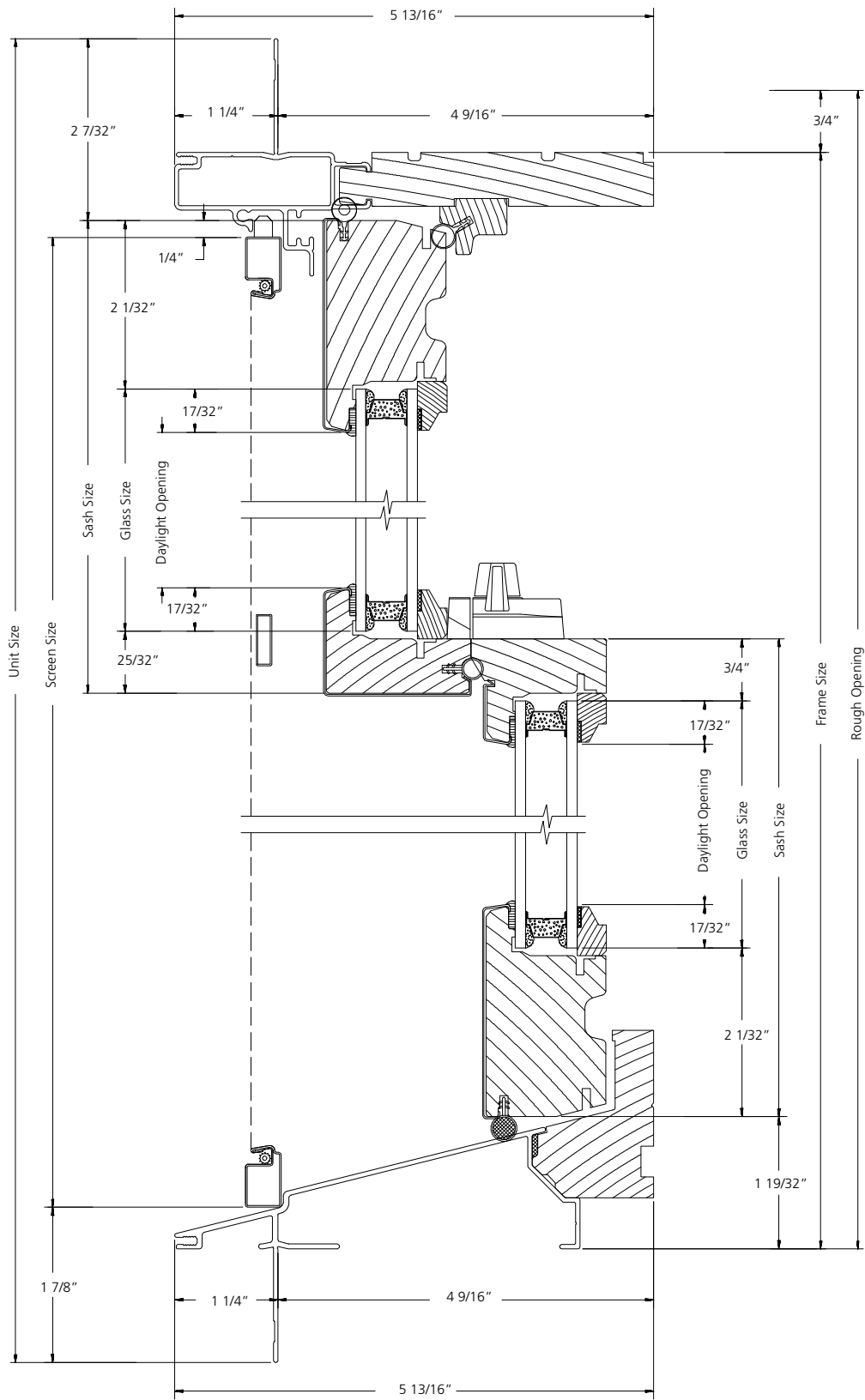
VERTICAL SECTION
