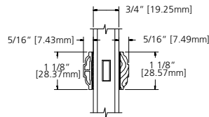
1 1/8" SDL
