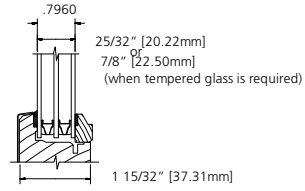
TRIPLE GLAZE INSULATED
