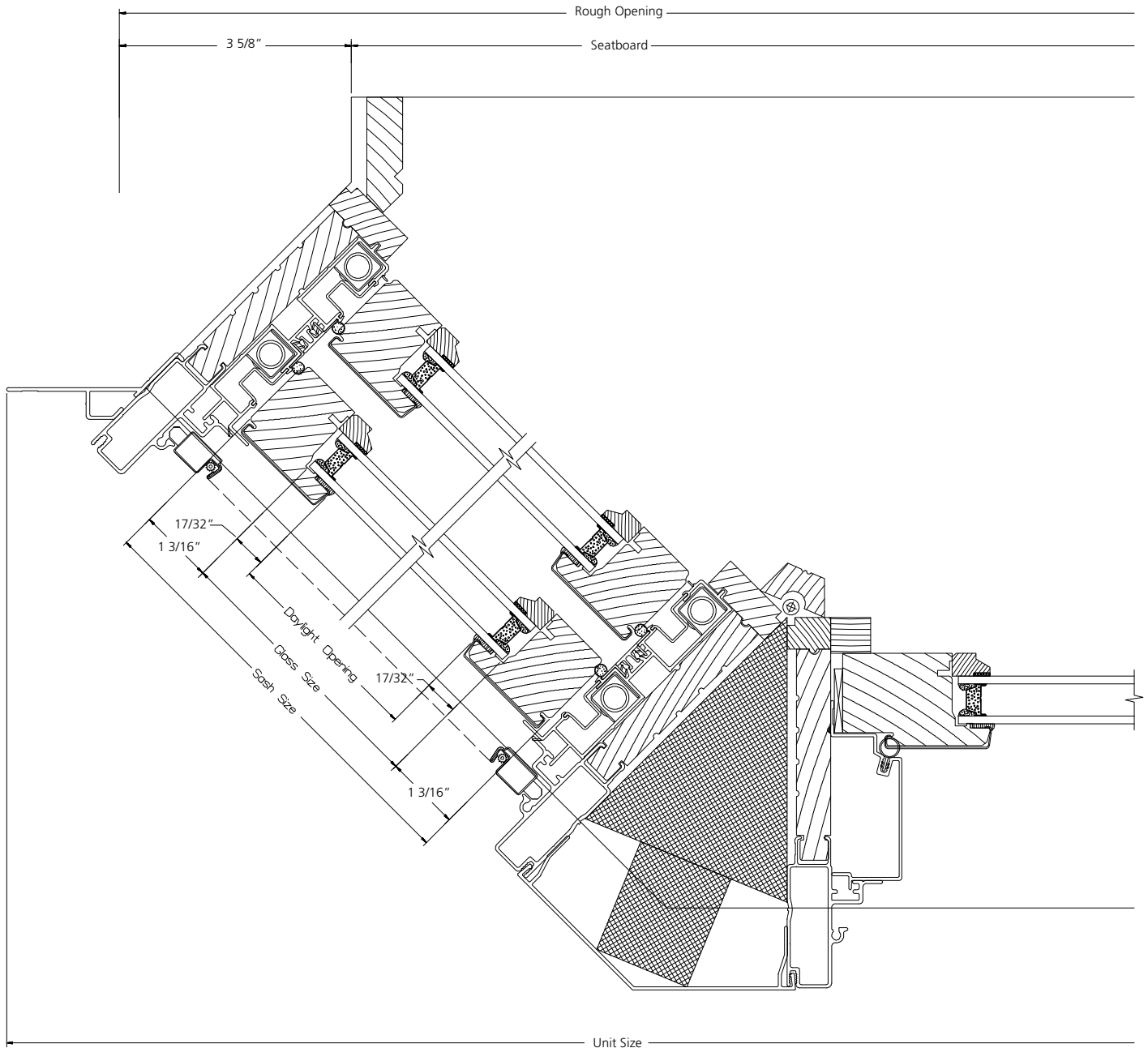
HORIZONTAL SECTION
