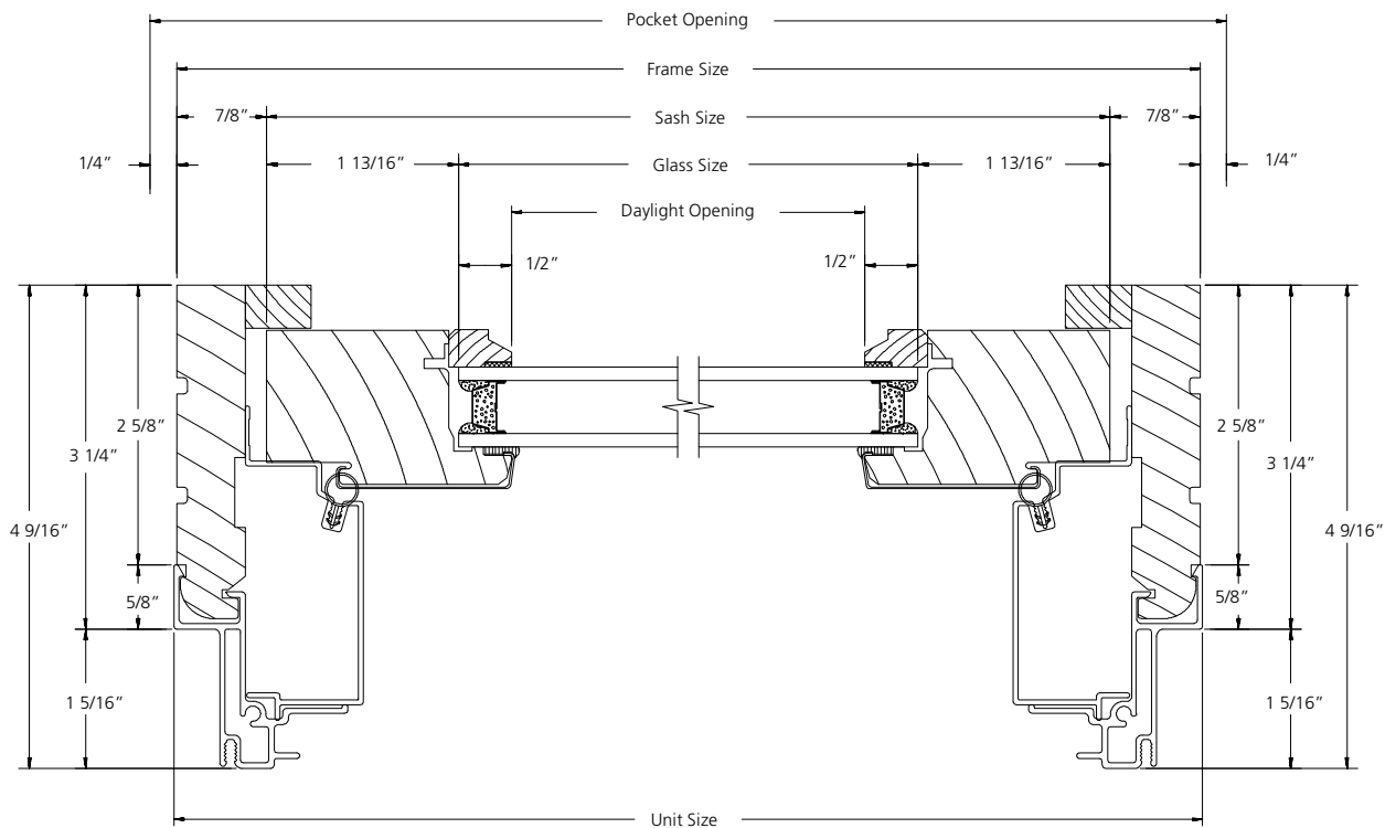
HORIZONTAL SECTION
