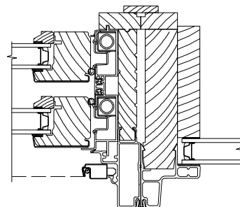
OPERATING DOUBLE HUNG NEXT TO DIRECT SET
