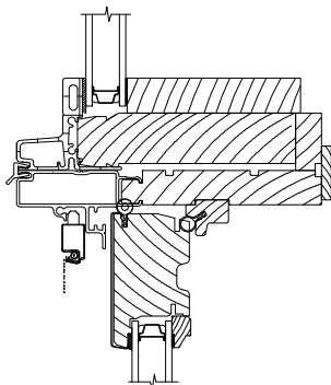
DIRECT SET EXTENDED RADIUS OVER DOUBLE HUNG
