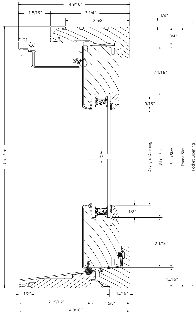
VERTICAL SECTION
