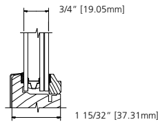
LAMINATED INSULATED CLEAR OR LOW-E 3.0mm//6.7mm LAMINATE
