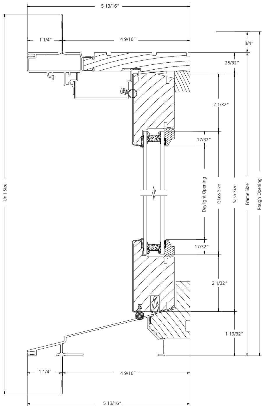
VERTICAL SECTION
