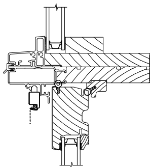
DIRECT SET RADIUS OVER DOUBLE HUNG
