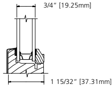
INSULATED GLASS
