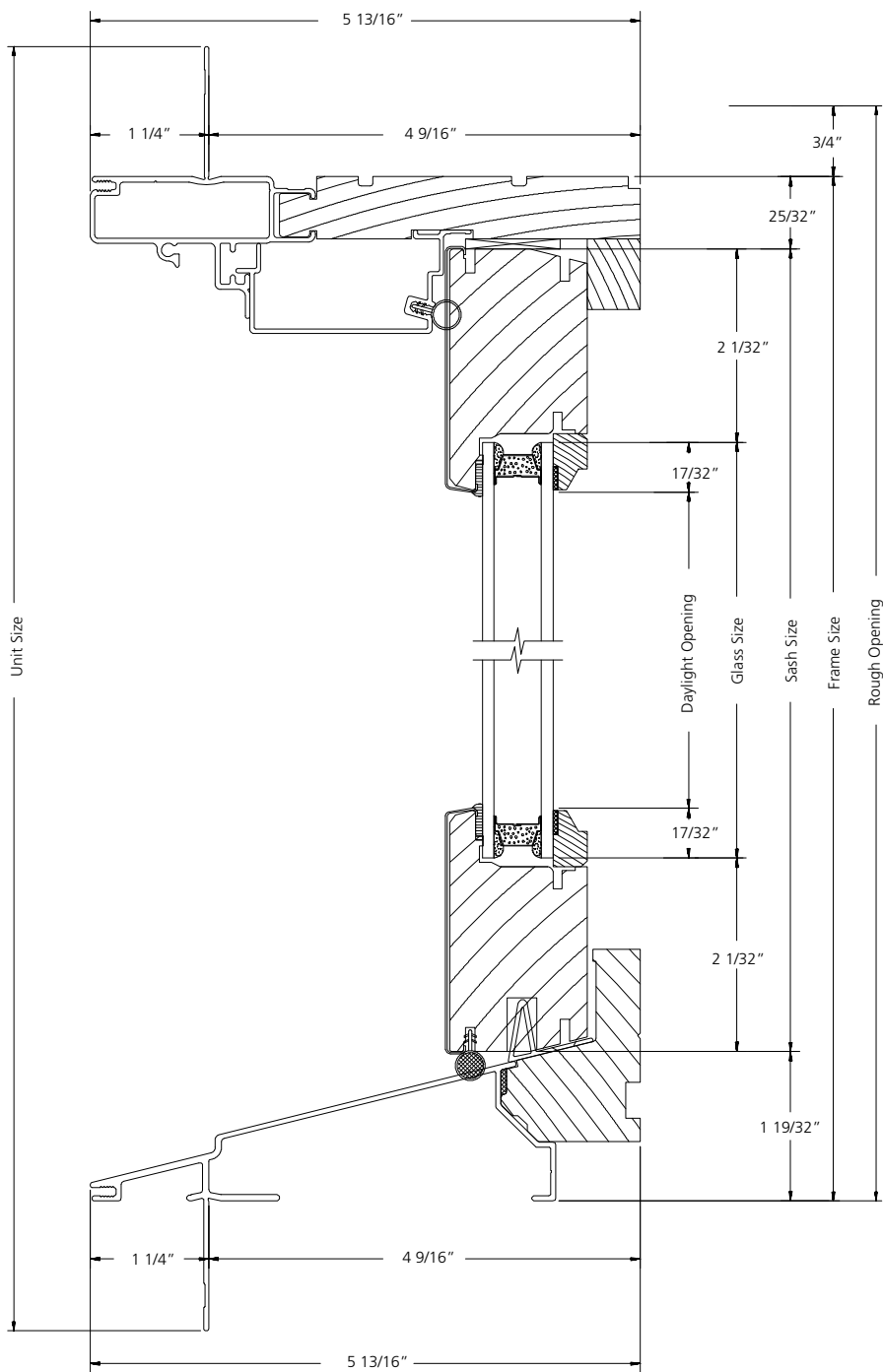
VERTICAL SECTION
