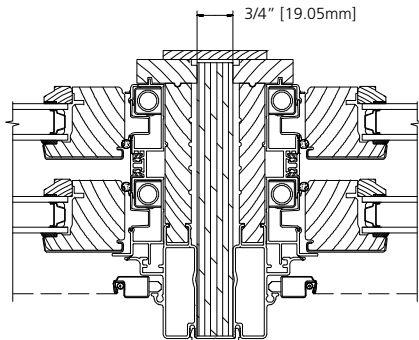
3/4" WOOD SPREAD MULL
