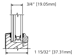
LAMINATED INSULATED TINTED 6.7mm LAMINATE//3.0mm
