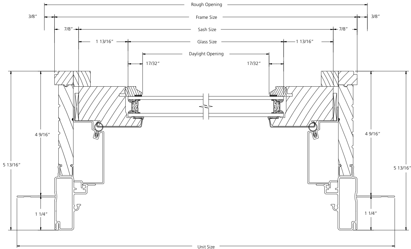
HORIZONTAL SECTION
