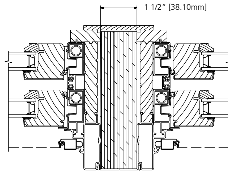
1 1/2" WOOD SPREAD MULL
