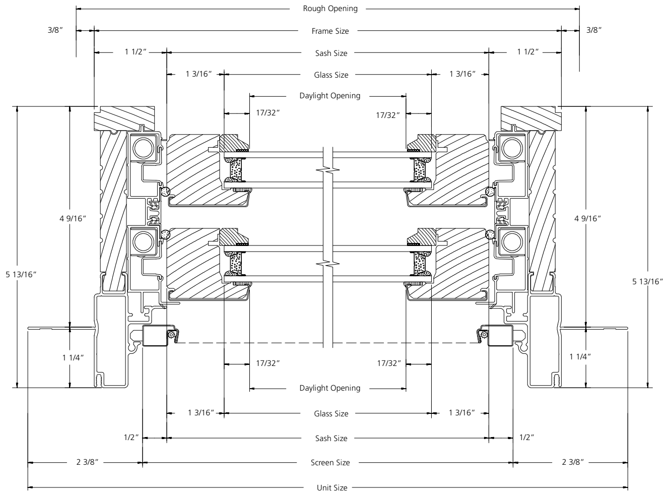
HORIZONTAL SECTION
