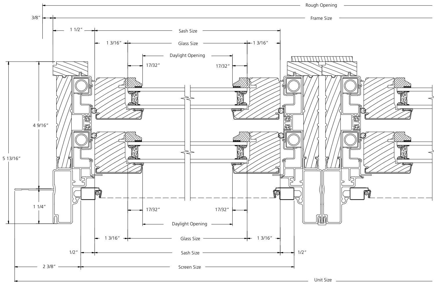
HORIZONTAL SECTION
