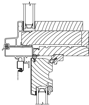
DIRECT SET GEOMETRIC OVER DOUBLE HUNG
