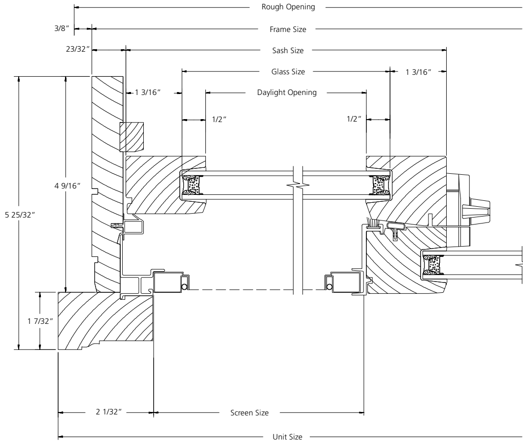
HORIZONTAL SECTION
