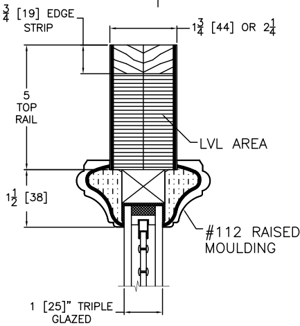
VERTICAL GLAZED CROSS SECTION 1-LITE SIDELIGHT ONLY Triple Glazed
