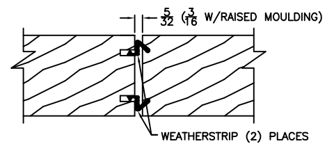
PANEL-TO-PANEL GAP
