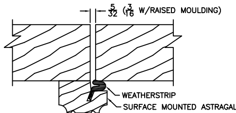
PANEL-TO-PANEL GAP AT ASTRAGAL
