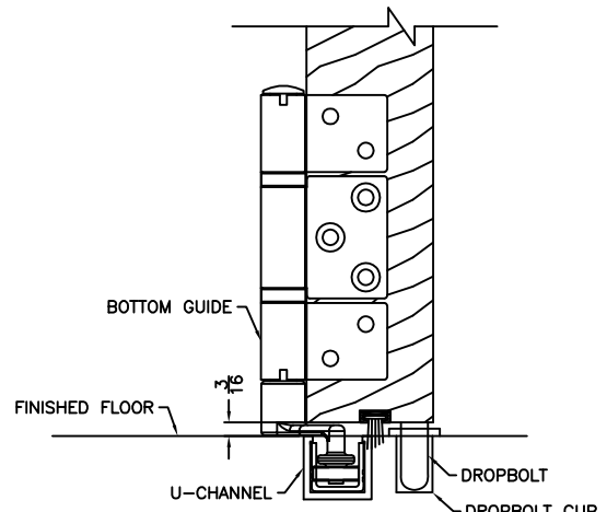
U-CHANNEL (Available Upon Request)
