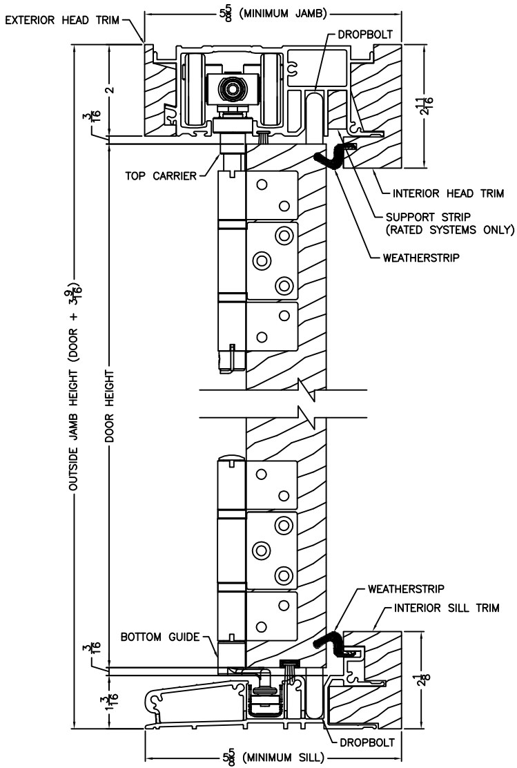
STANDARD SILL & HEAD
