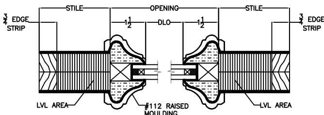
HORIZONTAL CROSS SECTION
