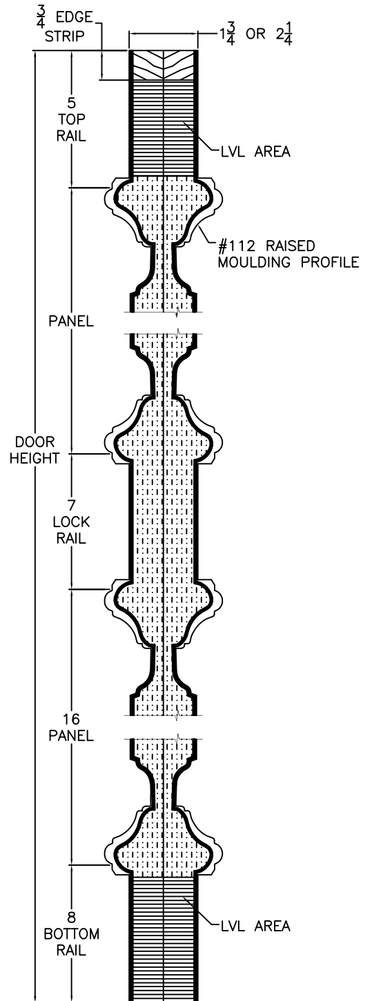
VERTICAL PANEL CROSS SECTION
