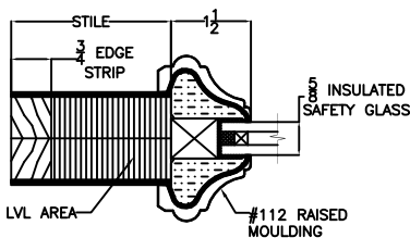
HORIZONTAL CROSS SECTION
