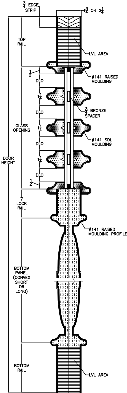
VERTICAL CROSS SECTION 4-LITE SDL SIDELIGHT ONLY
