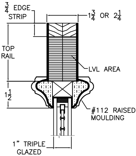
VERTICAL GLAZED CROSS SECTION Triple Glazed
