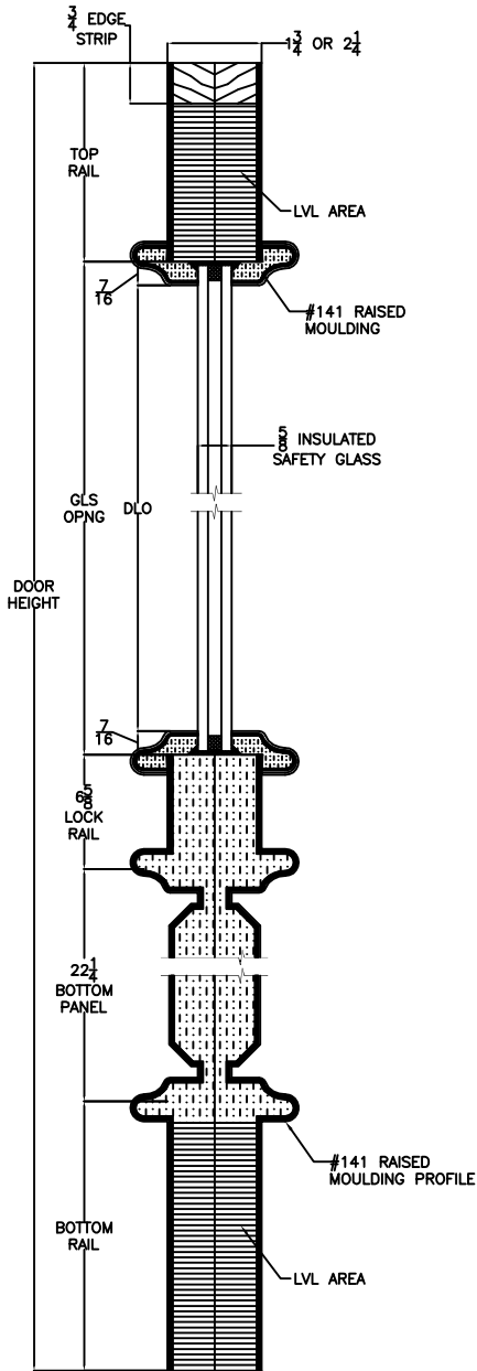
VERTICAL CROSS SECTION
