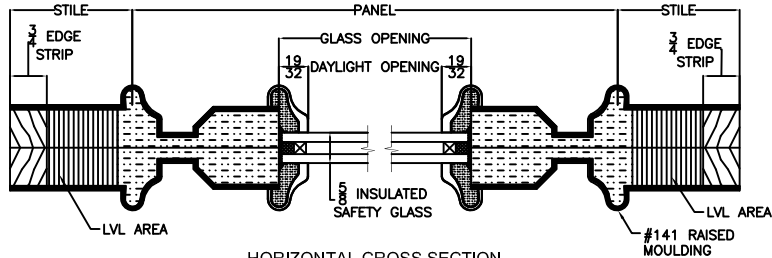
HORIZONTAL CROSS SECTION
