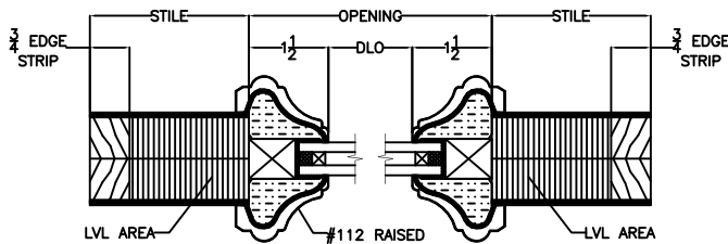
HORIZONTAL CROSS SECTION
