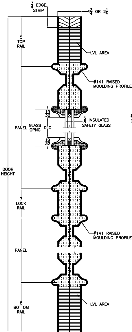
VERTICAL CROSS SECTION
