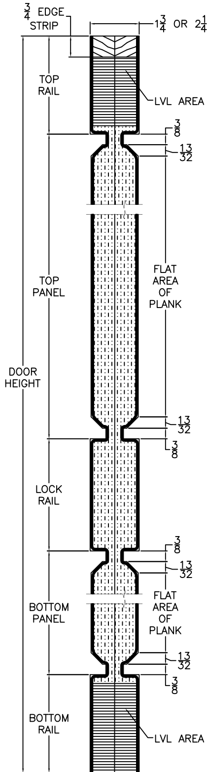
VERTICAL PANEL CROSS SECTION
