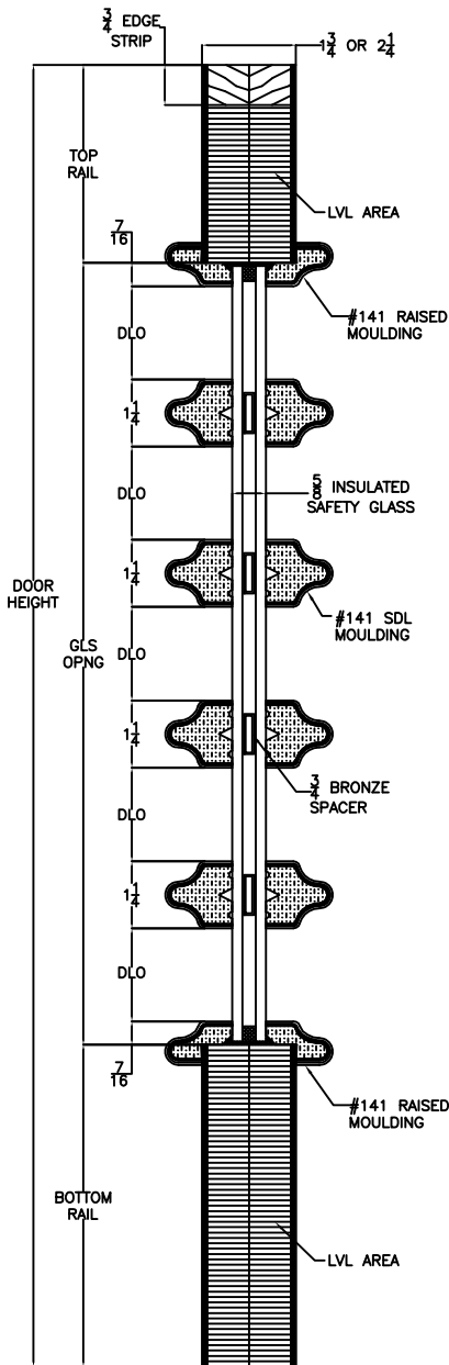
VERTICAL CROSS SECTION
