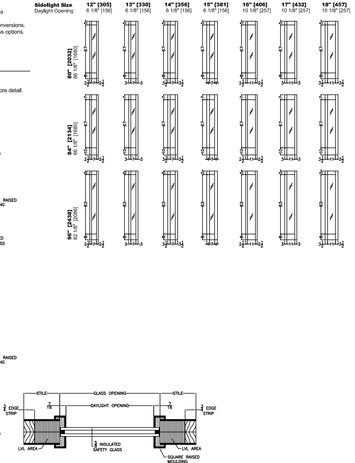
HORIZONTAL CROSS SECTION
