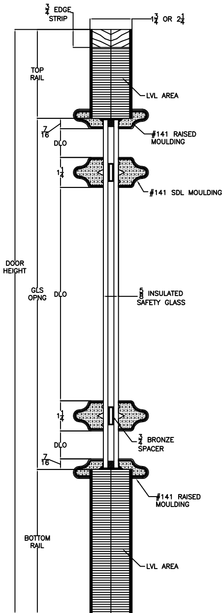
VERTICAL DOOR CROSS SECTION Insulated Glass
