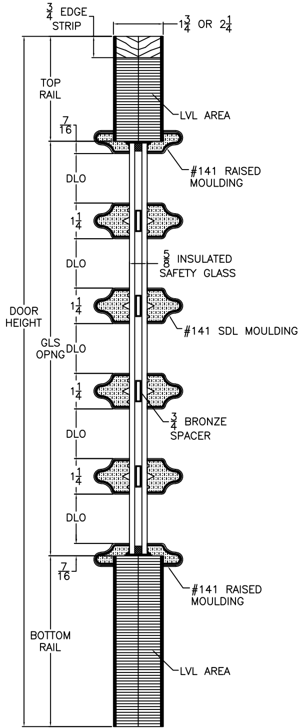
VERTICAL SIDELIGHT CROSS SECTION Insulated Glass
