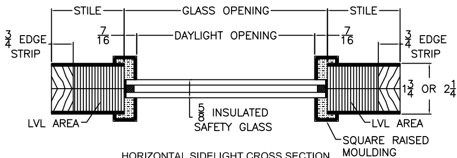
HORIZONTAL SIDELIGHT CROSS SECTION Insulated Glass
