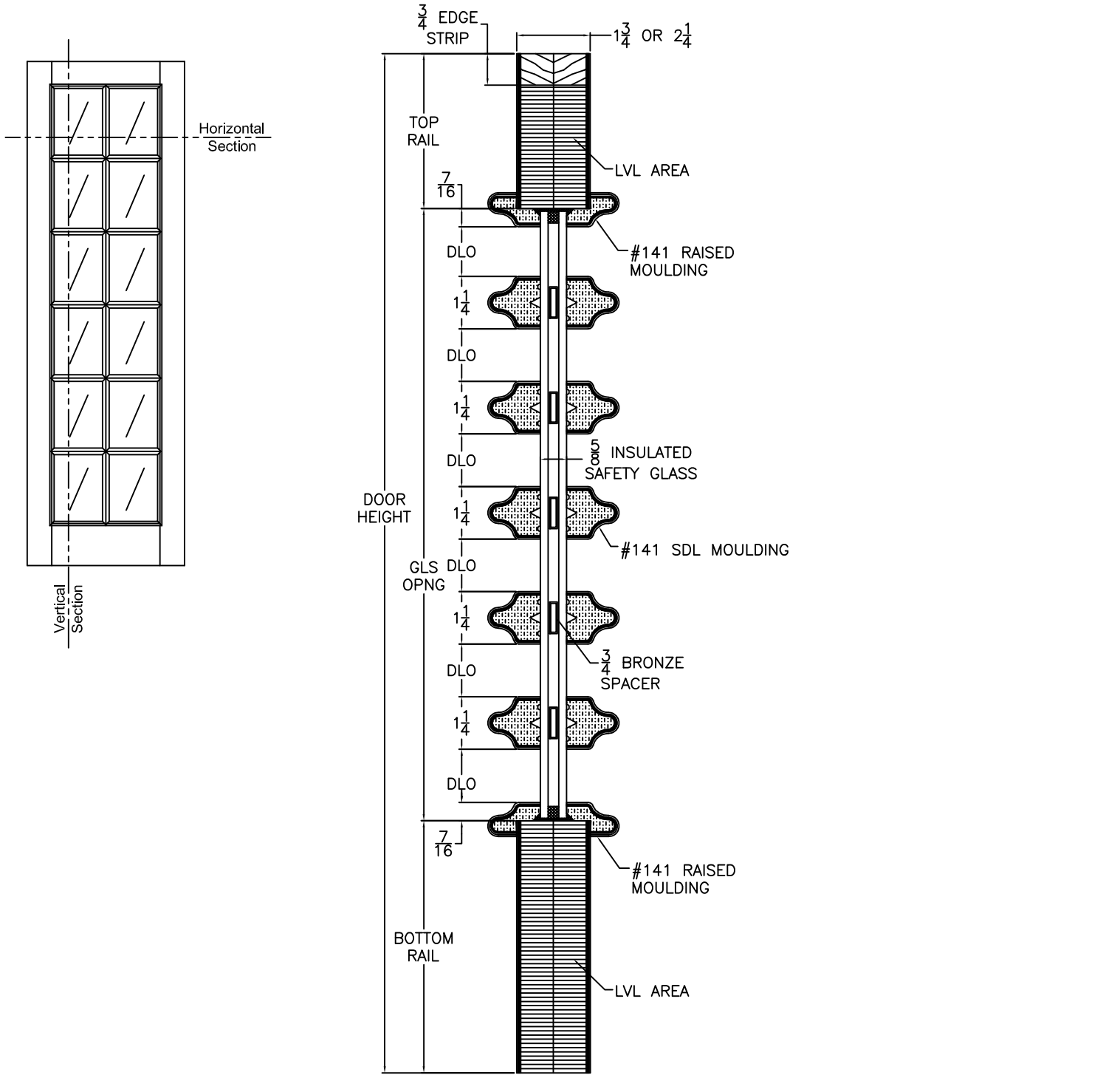
VERTICAL DOOR CROSS SECTION Insulated Glass
