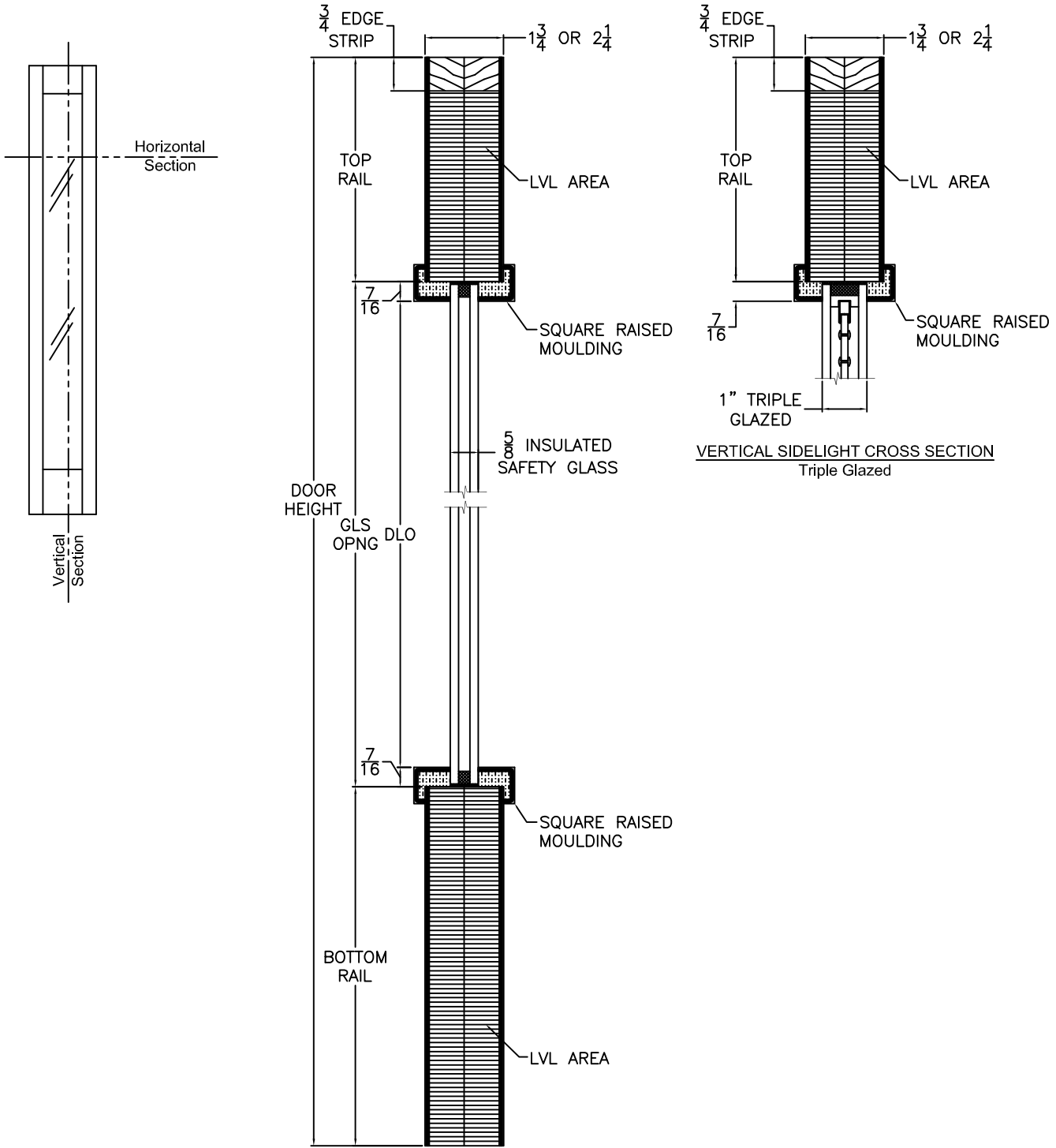
VERTICAL SIDELIGHT CROSS SECTION Insulated Glass
