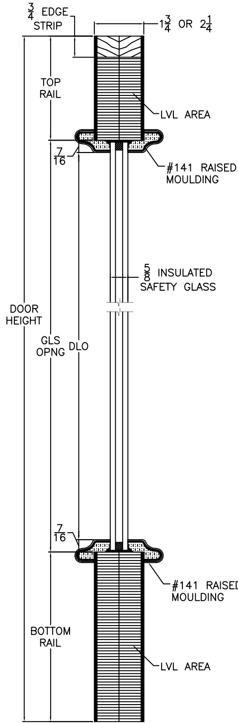
VERTICAL SIDELIGHT CROSS SECTION Insulated Glass
