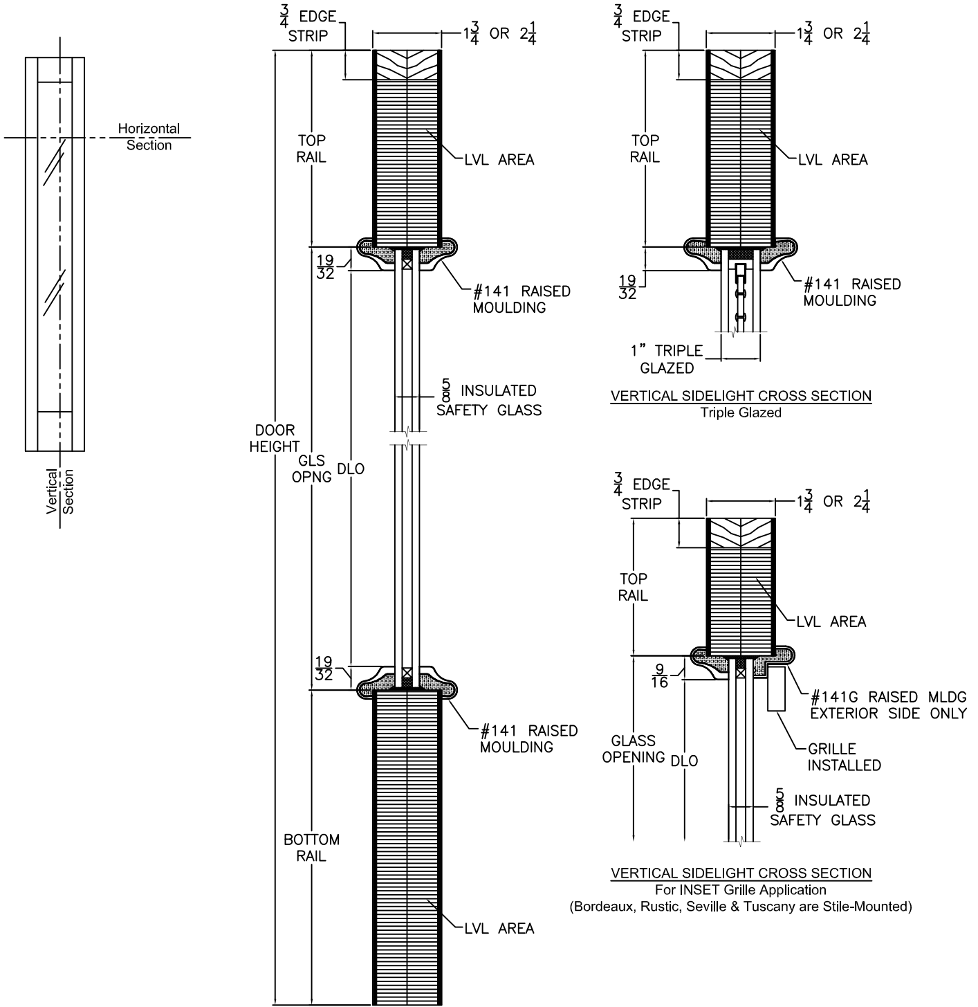
VERTICAL SIDELIGHT CROSS SECTION Insulated Glass
