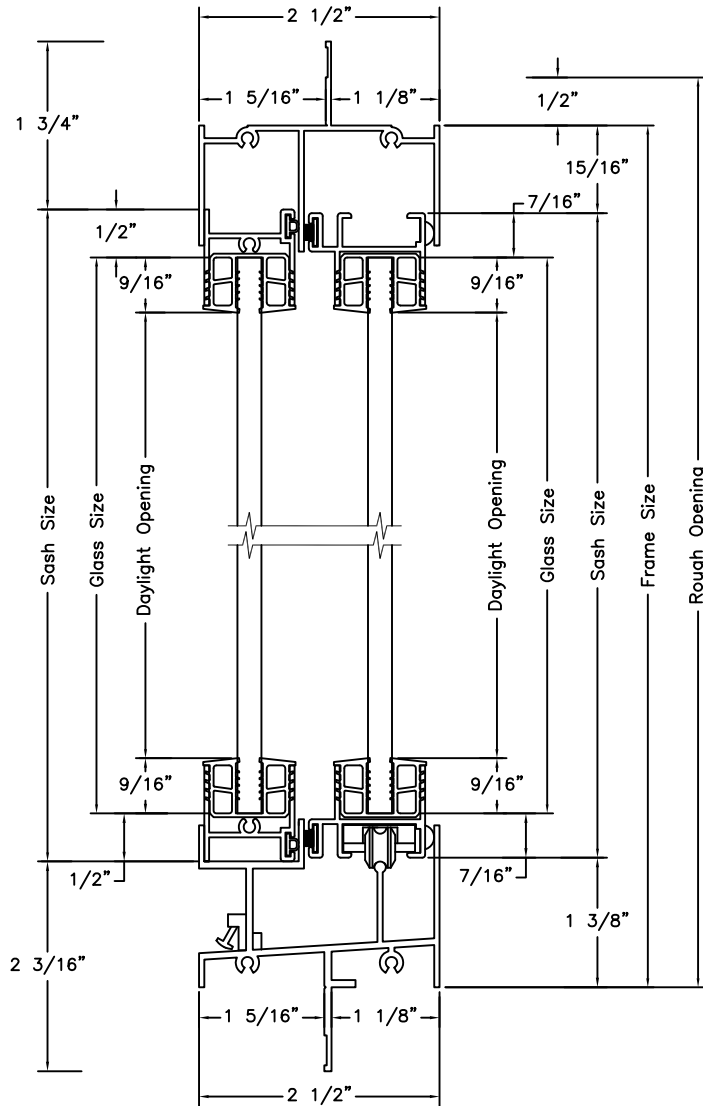
Vertical Section
