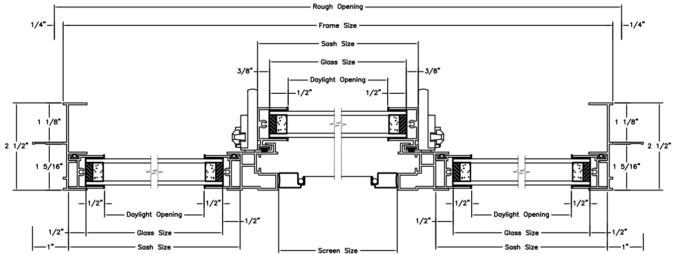
Horizontal Section
