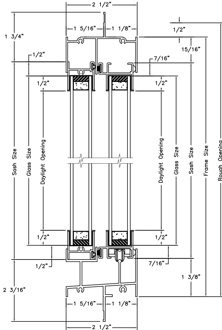
Vertical Section
