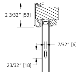
23/32" CONTOUR GBG
