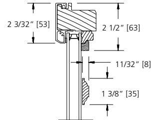
1 3/8" GRILLE BAR
