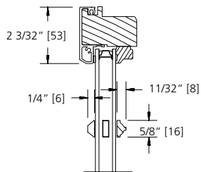
5/8" SDL BAR (PUTTY/BEAD)
