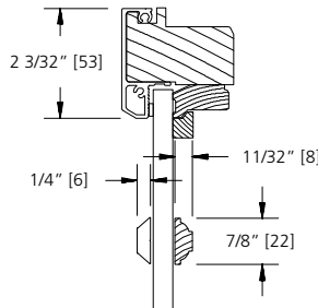
7/8" SDL (PUTTY/BEAD)
