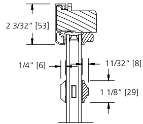
1 1/8" SDL BAR (PUTTY/BEAD)
