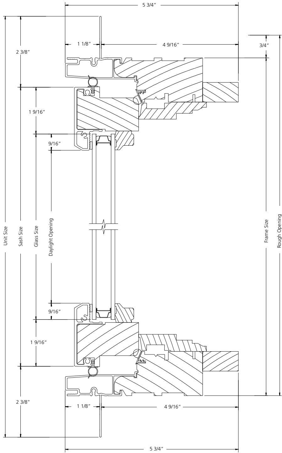
VERTICAL SECTION
