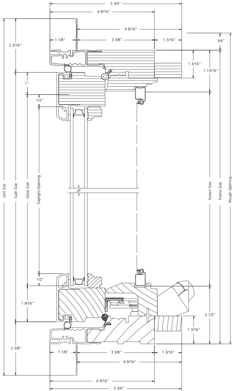
VERTICAL SECTION
