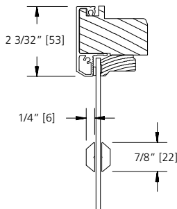
7/8" SDL (PUTTY/PUTTY)
