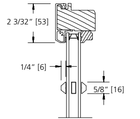
5/8" SDL BAR (PUTTY/PUTTY)
