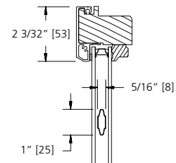
1" CONTOUR GBG
