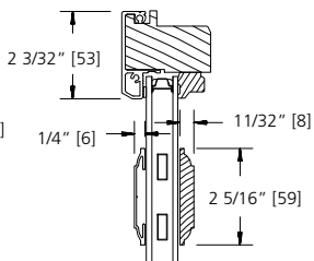
2 5/16" SDL BAR (BEAD STOP)
