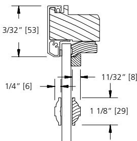
1 1/8" SDL (BEAD STOP)
