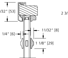
1 1/8" SDL BAR (BEAD STOP)
