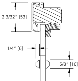
5/8" SDL (PUTTY/PUTTY)
