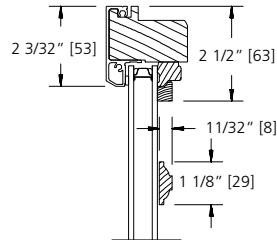
1 1/8" GRILLE BAR
