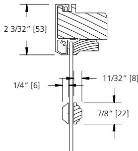
7/8" SDL (PUTTY/BEAD)
