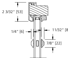
7/8" SDL BAR (BEAD STOP)
