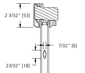
23/32" CONTOUR GBG
