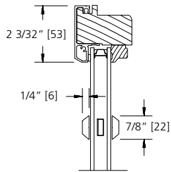
7/8" SDL BAR (PUTTY/PUTTY)
