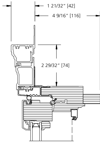
ADAMS CASING
