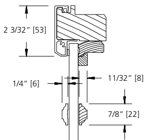
7/8" SDL (BEAD STOP)
