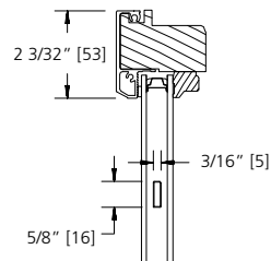
5/8" FLAT GBG
