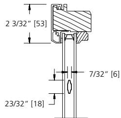
23/32" CONTOUR GBG
