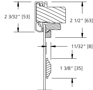
1 3/8" GRILLE BAR
