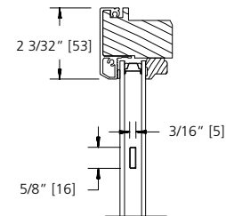
5/8" FLAT GBG
