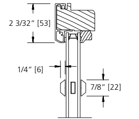
7/8" SDL BAR (PUTTY/PUTTY)
