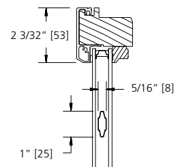
1" CONTOUR GBG
