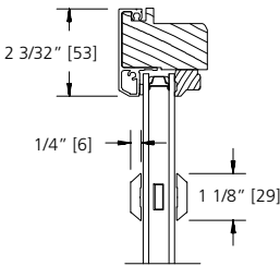
1 1/8" SDL BAR (PUTTY/PUTTY)
