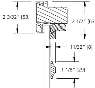
1 1/8" GRILLE BAR
