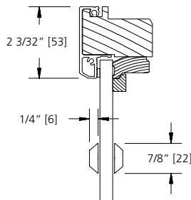
7/8" SDL (PUTTY/PUTTY)
