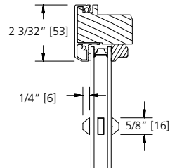
5/8" SDL BAR (PUTTY/PUTTY)
