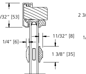
1 3/8" SDL BAR (BEAD STOP)
