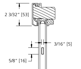
5/8" FLAT GBG
