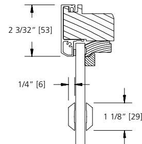
1 1/8" SDL (PUTTY/PUTTY)
