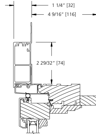
3 1/2" FLAT CASING
