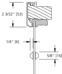
5/8" SDL (PUTTY/PUTTY)
