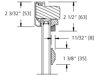
1 3/8" GRILLE BAR
