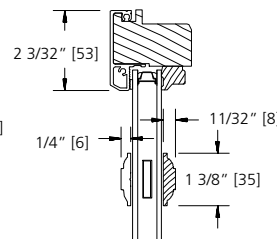
1 3/8" SDL BAR (BEAD STOP)
