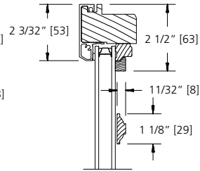
1 1/8" GRILLE BAR
