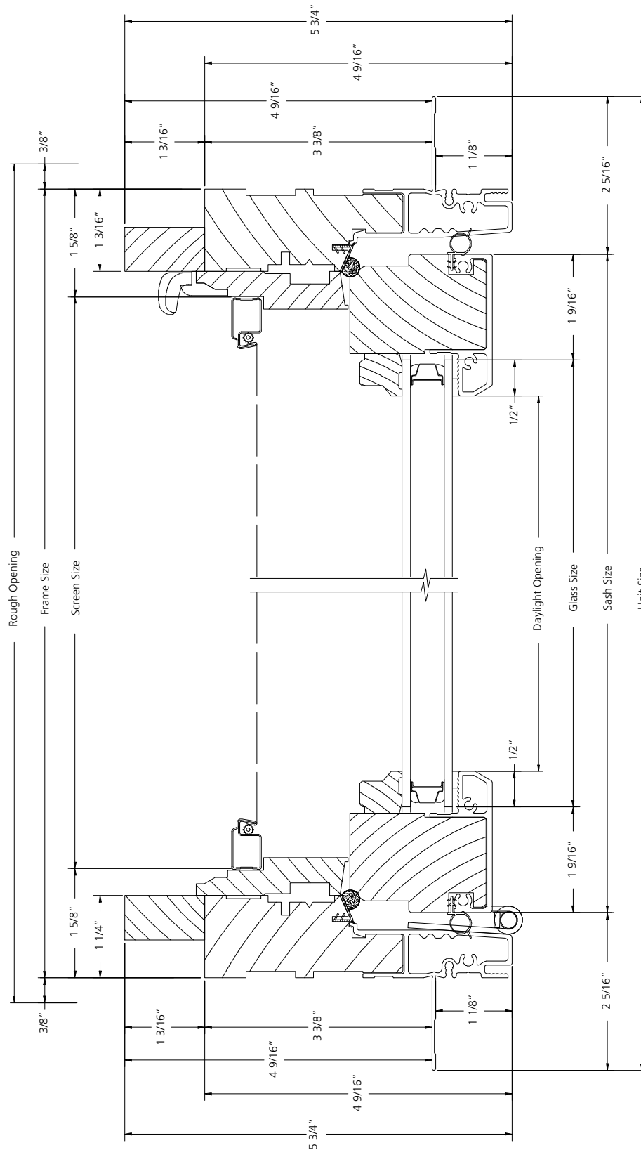
HORIZONTAL SECTION
