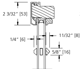
5/8" SDL BAR (PUTTY/BEAD)
