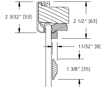
1 3/8" GRILLE BAR
