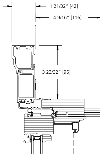
MANCHESTER CASING
