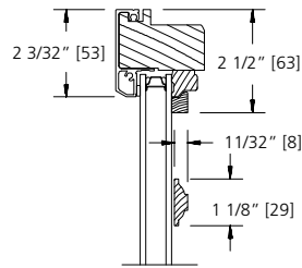
1 1/8" GRILLE BAR
