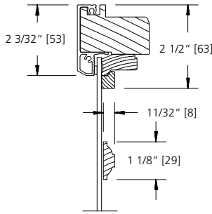
1 1/8" GRILLE BAR
