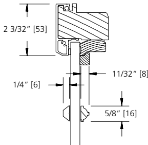
5/8" SDL (PUTTY/BEAD)
