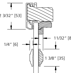
1 3/8" SDL (BEAD STOP)
