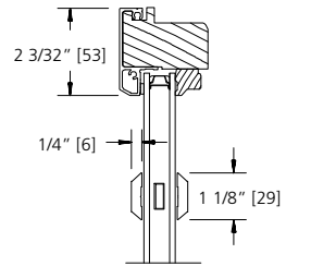
1 1/8" SDL BAR (PUTTY/PUTTY)
