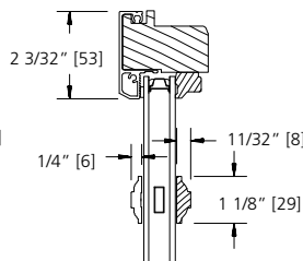
1 1/8" SDL BAR (BEAD STOP)
