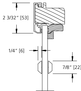
7/8" SDL (PUTTY/PUTTY)
