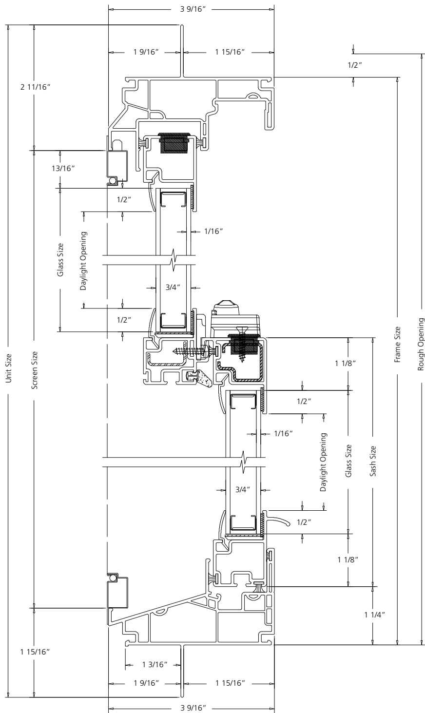
VERTICAL SECTION
