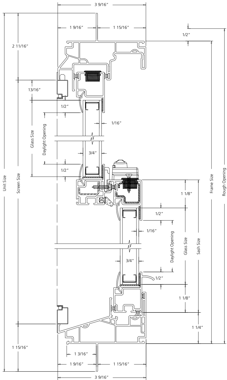
VERTICAL SECTION
