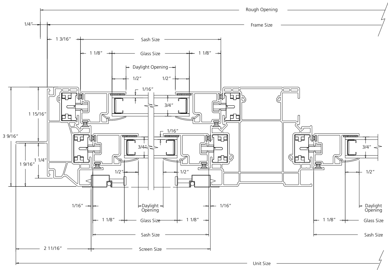
HORIZONTAL SECTION
