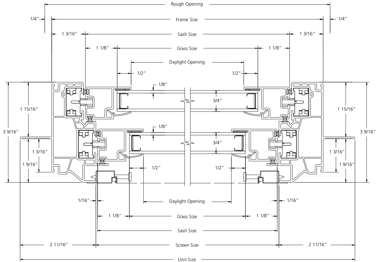
HORIZONTAL SECTION
