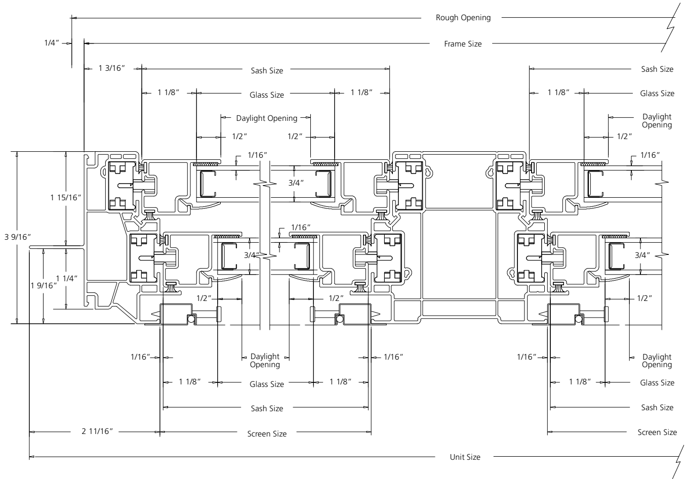
HORIZONTAL SECTION
