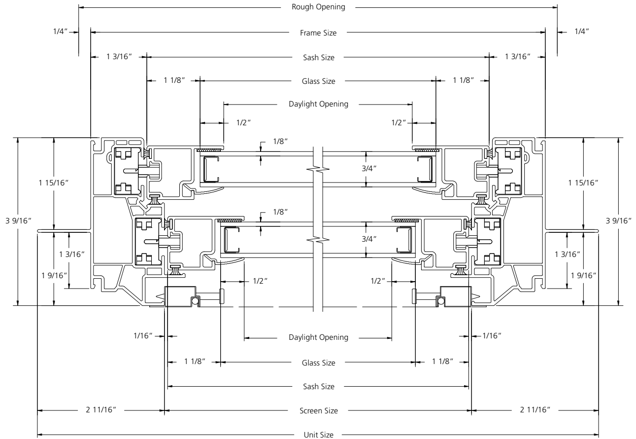
HORIZONTAL SECTION
