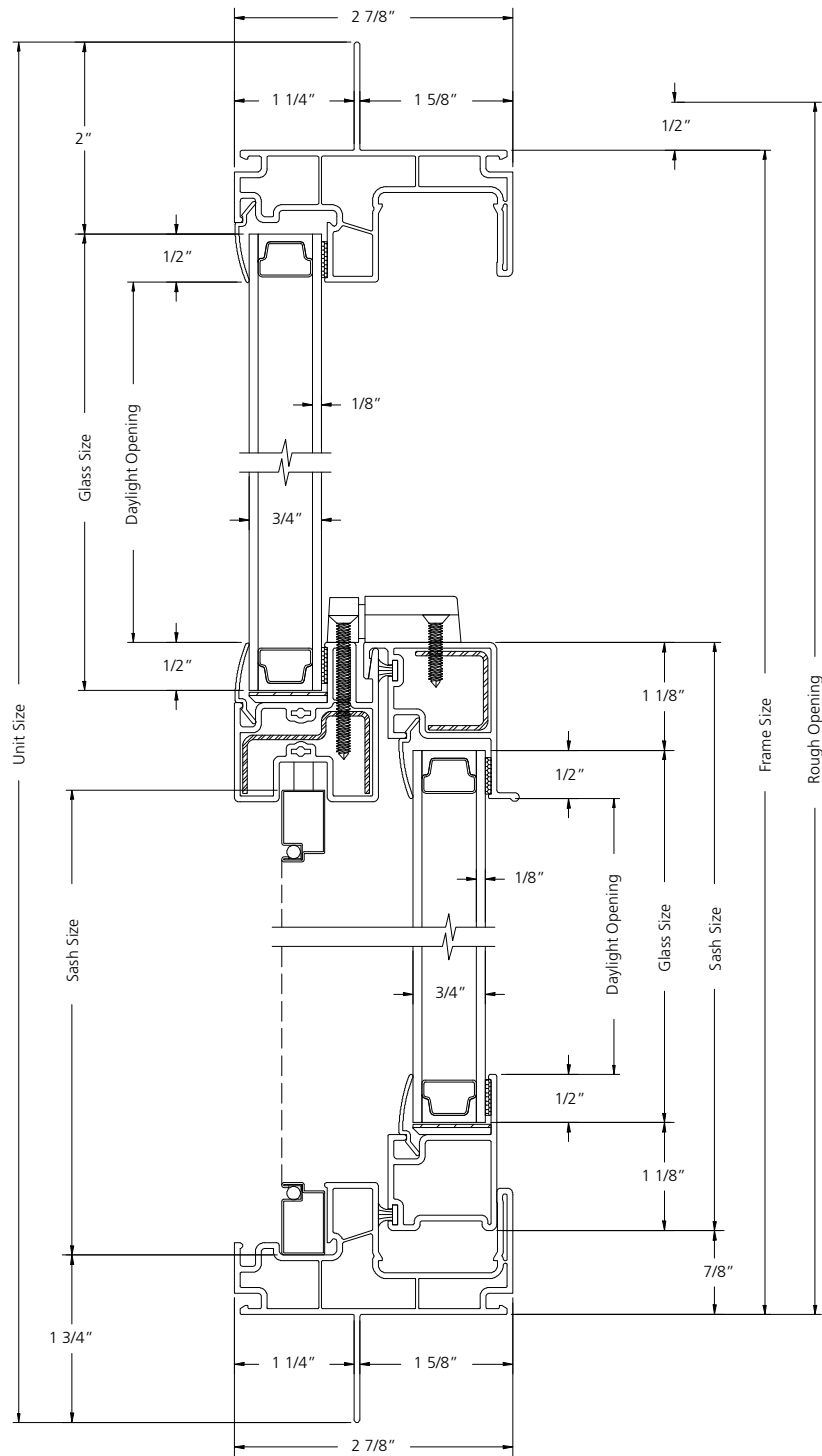
VERTICAL SECTION
