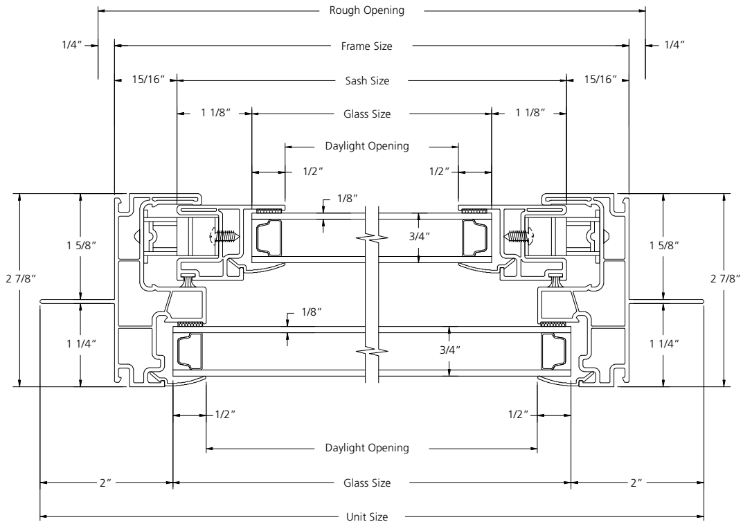
HORIZONTAL SECTION
