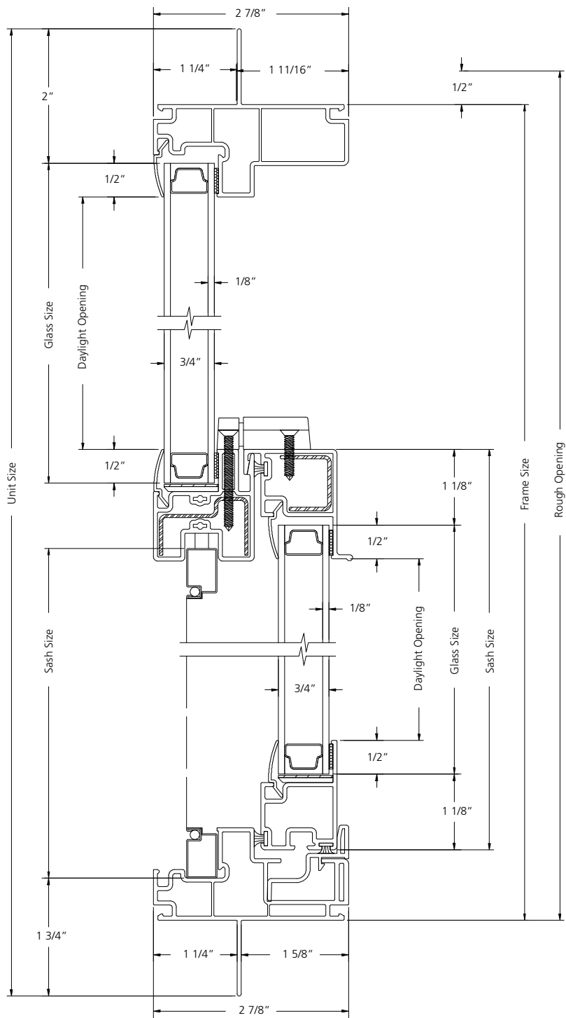
VERTICAL SECTION
