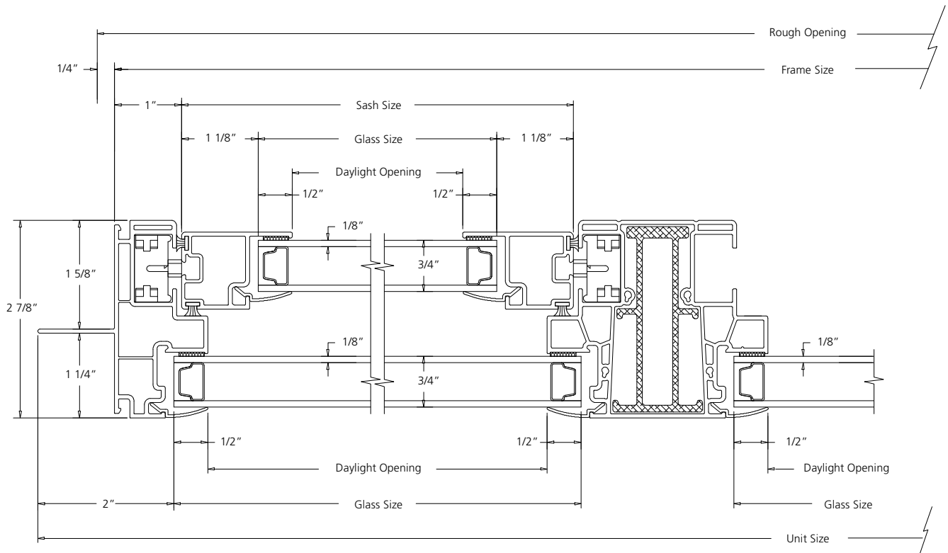
HORIZONTAL SECTION
