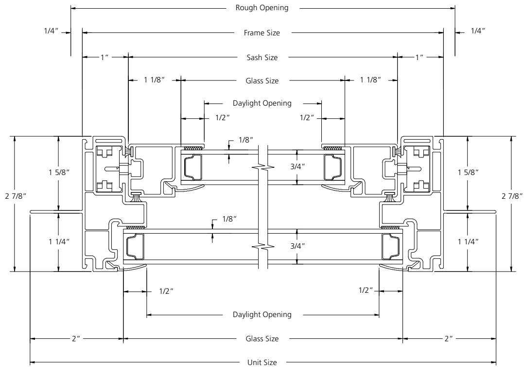
HORIZONTAL SECTION
