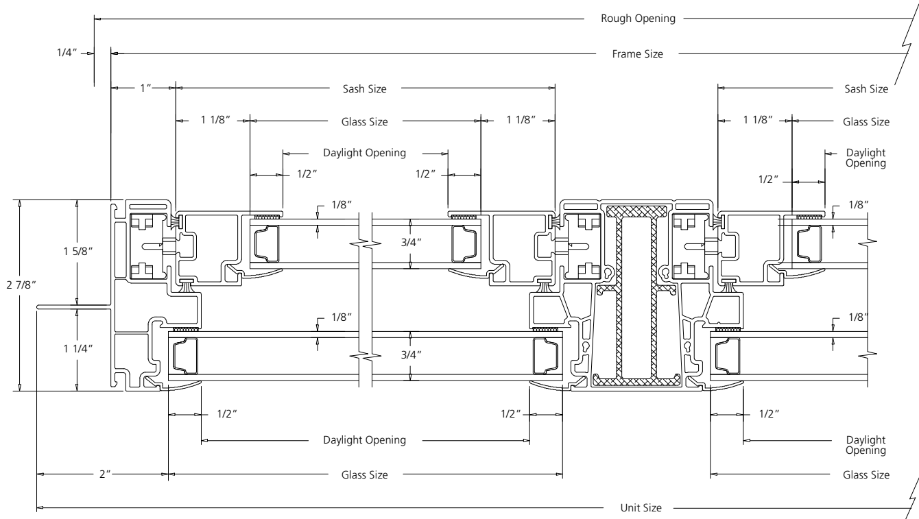
HORIZONTAL SECTION
