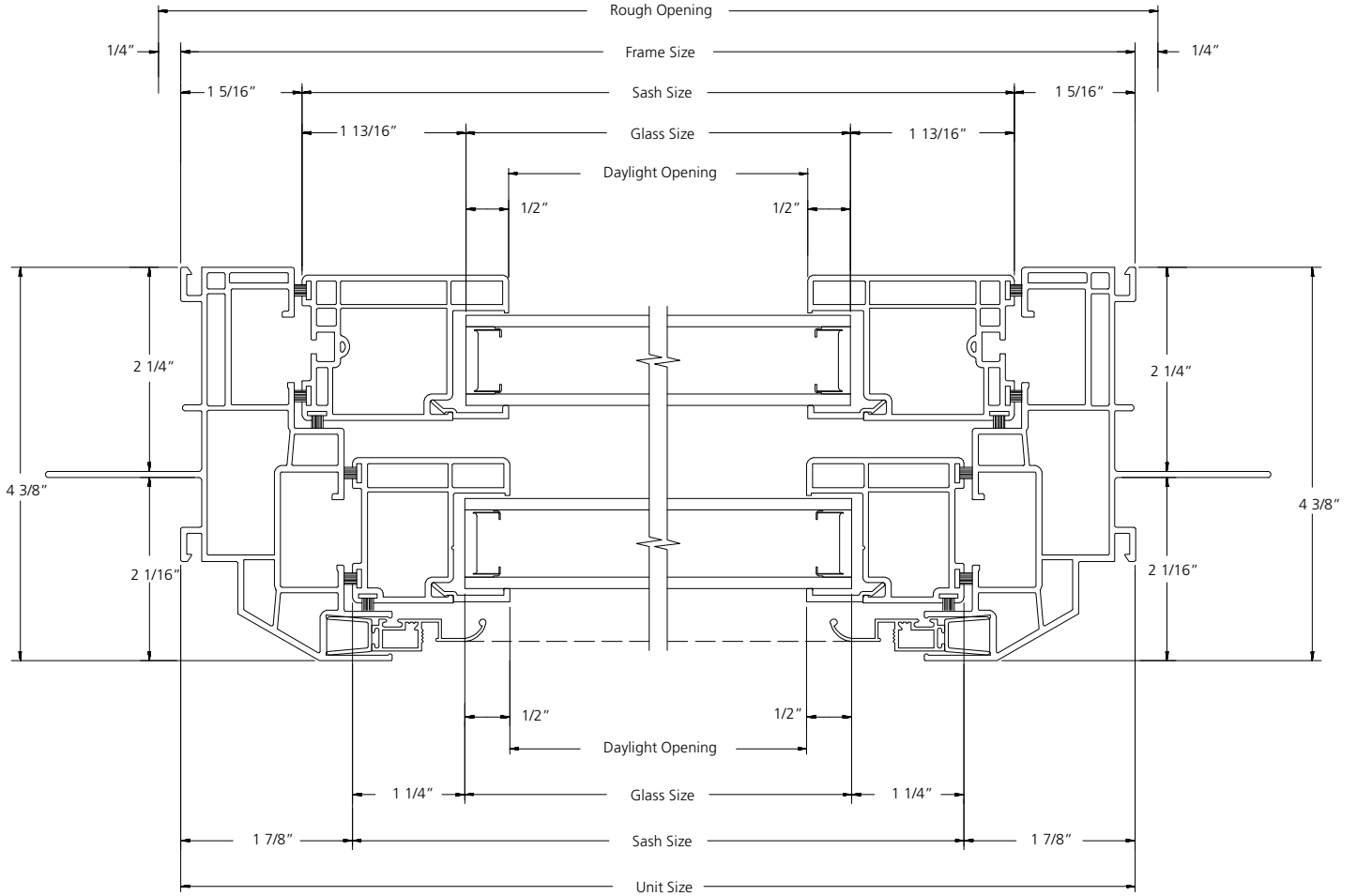
HORIZONTAL SECTION
