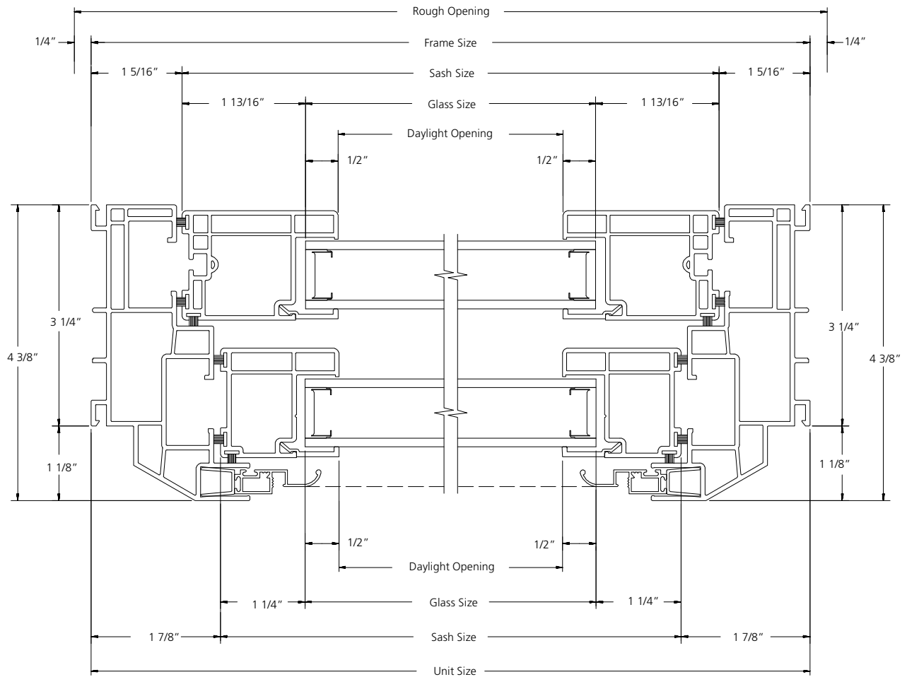
HORIZONTAL SECTION
