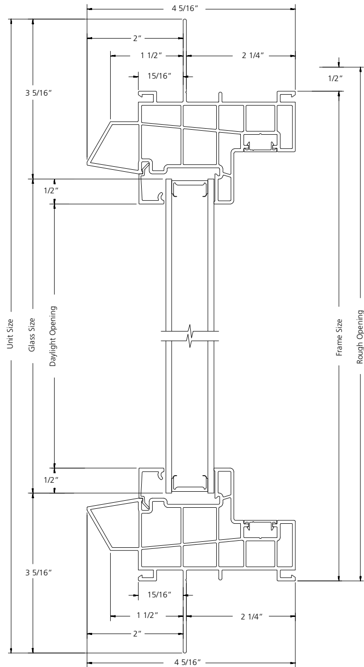
VERTICAL SECTION
