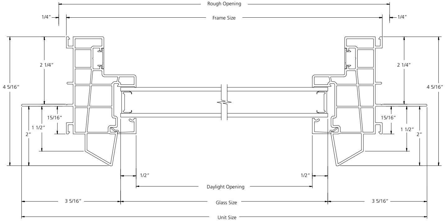
HORIZONTAL SECTION
