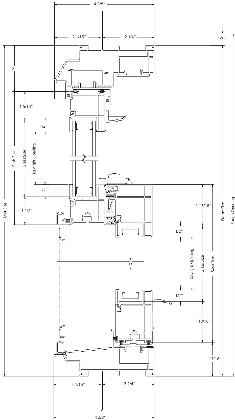
VERTICAL SECTION
