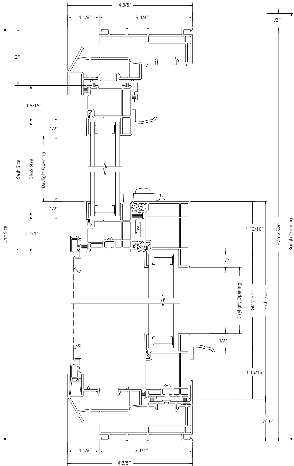
VERTICAL SECTION
