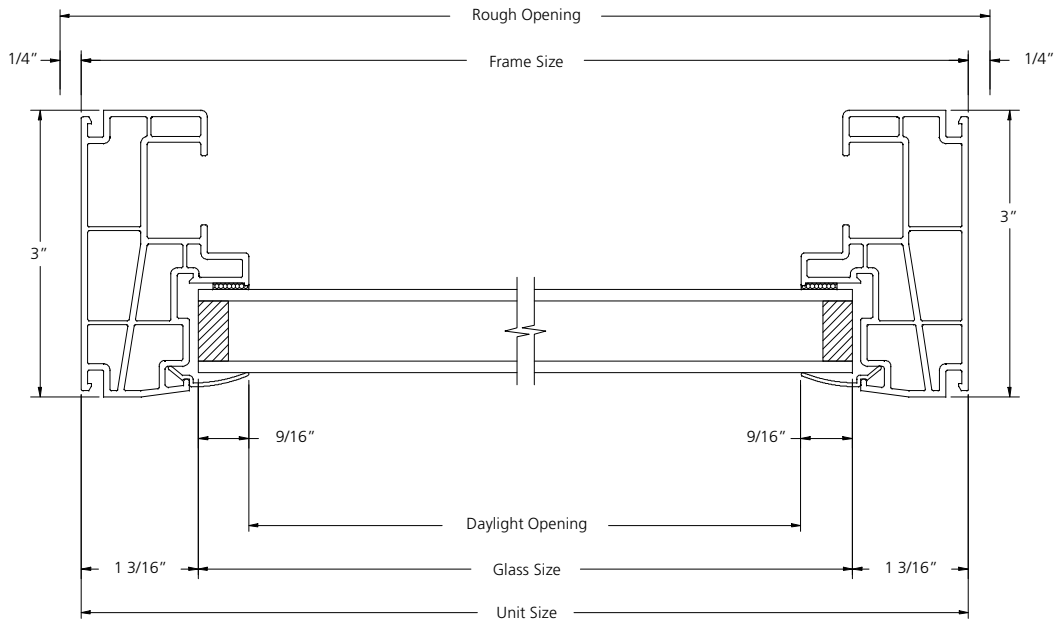
HORIZONTAL SECTION
