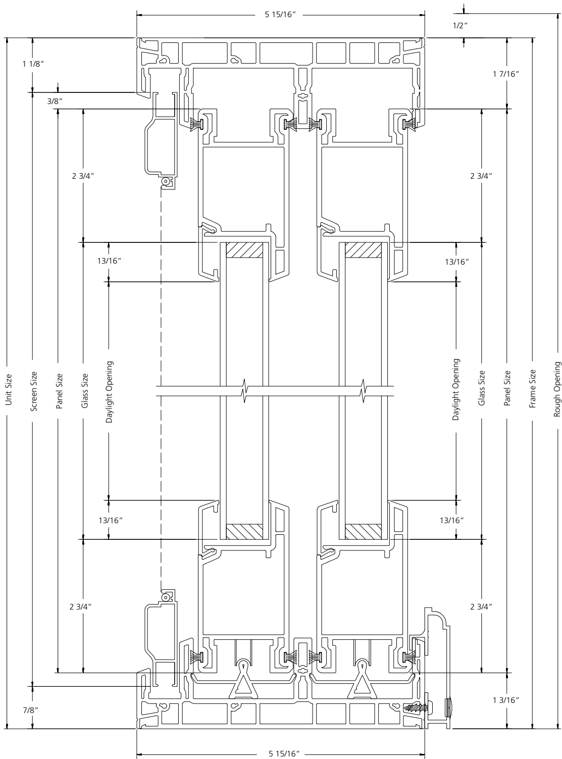
VERTICAL SECTION
