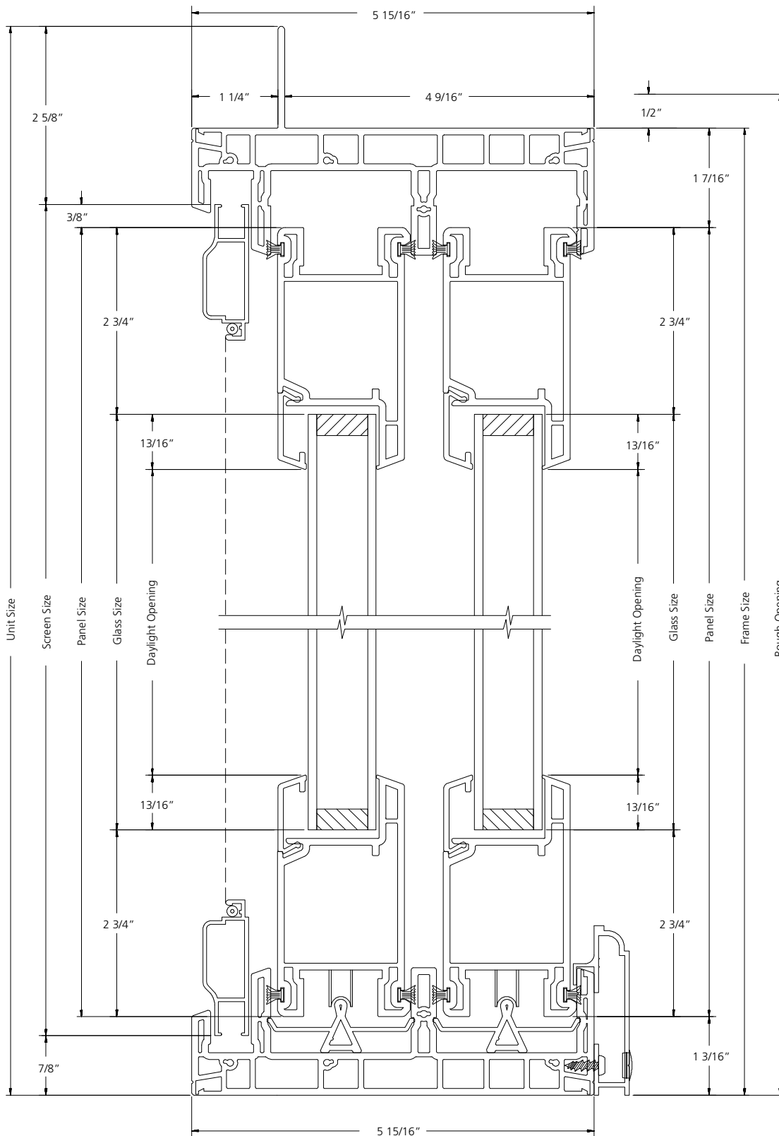
VERTICAL SECTION
