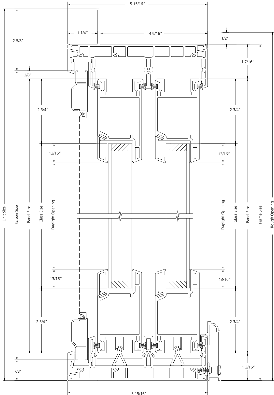
VERTICAL SECTION
