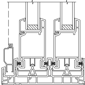
1" IG BBG ONLY
