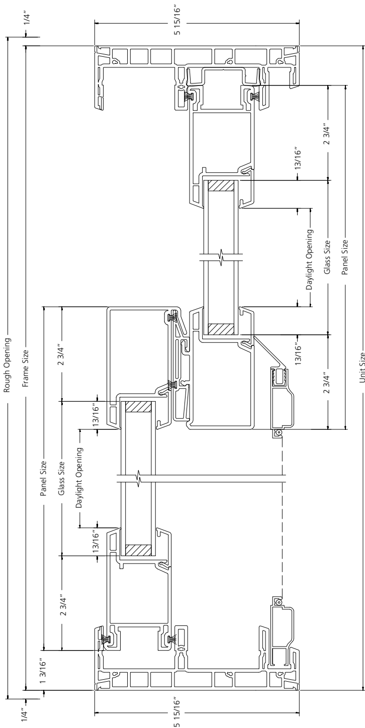
HORIZONTAL SECTION
