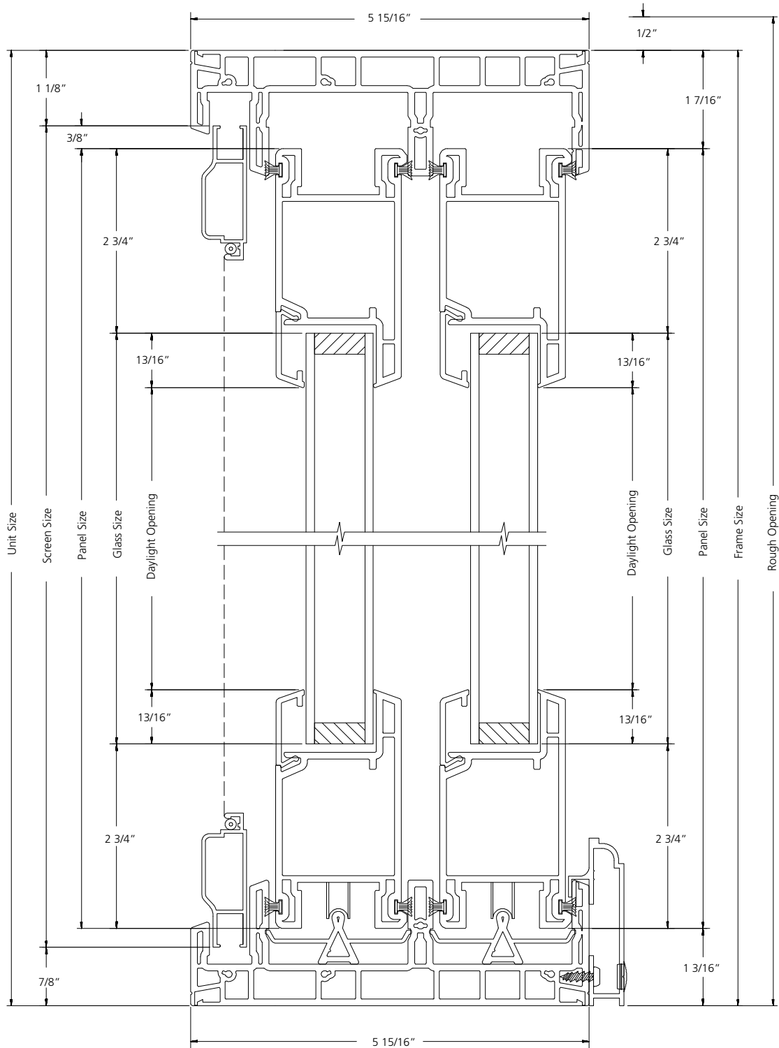
VERTICAL SECTION
