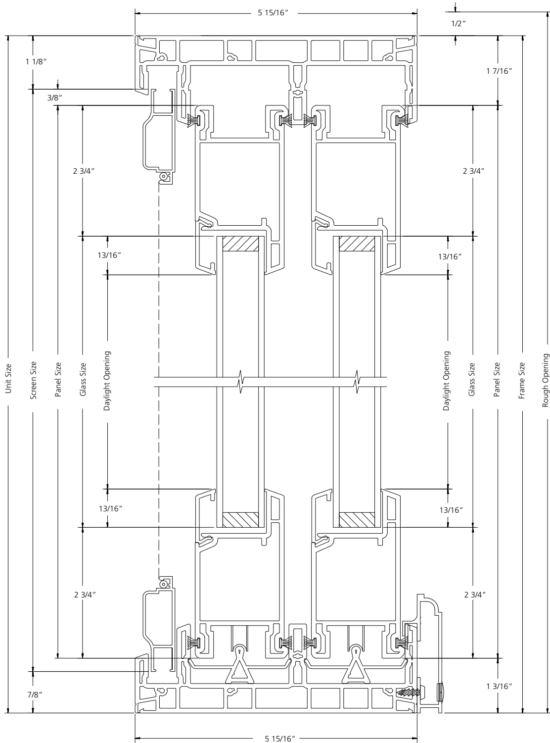
VERTICAL SECTION
