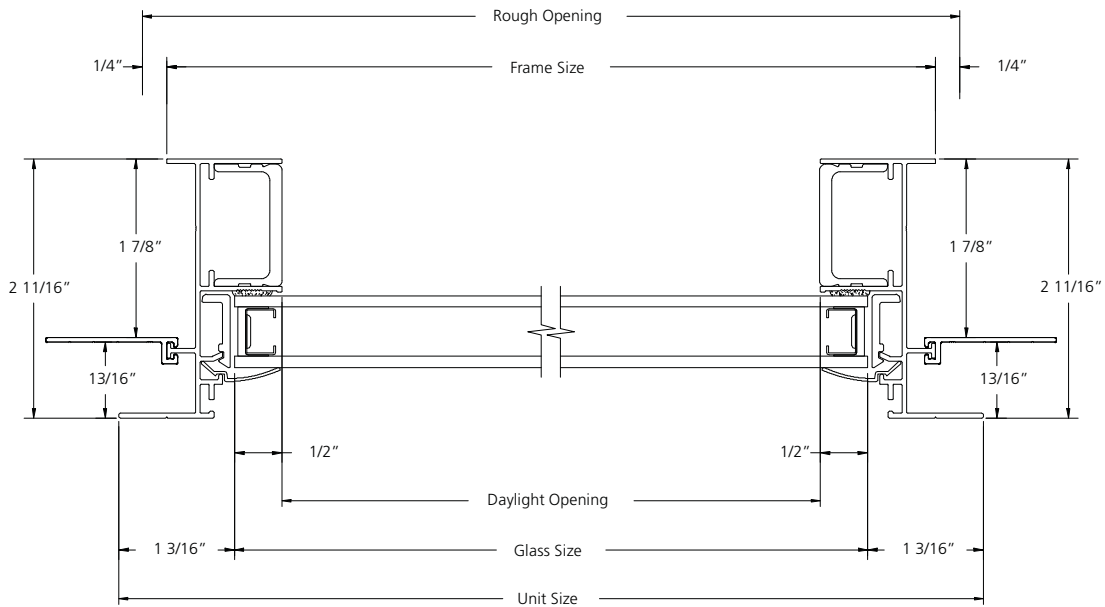
HORIZONTAL SECTION
