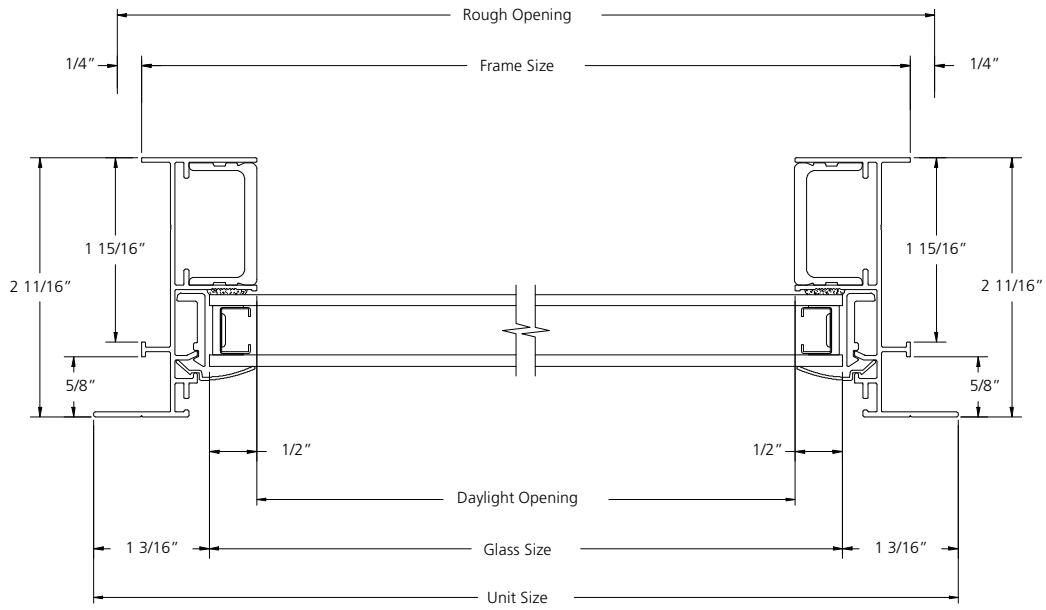
HORIZONTAL SECTION
