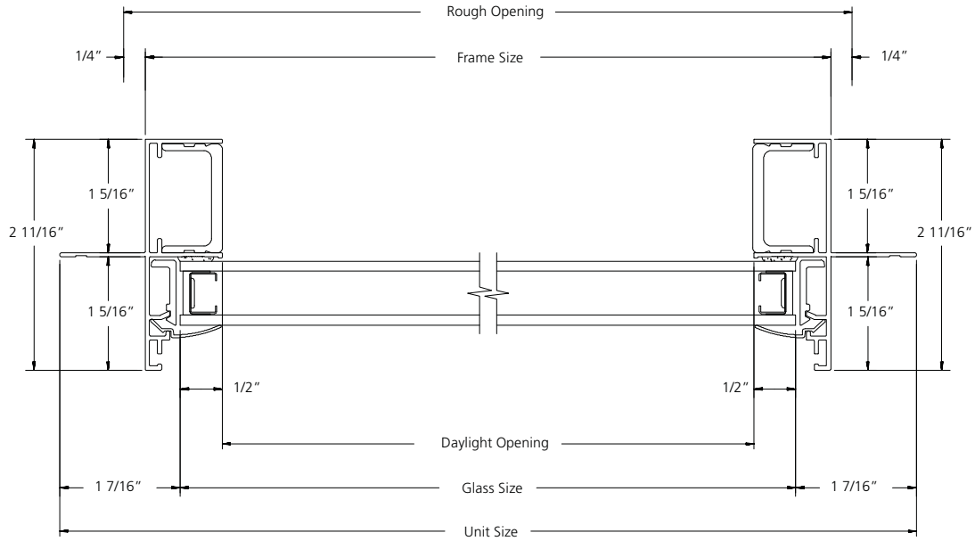
HORIZONTAL SECTION
