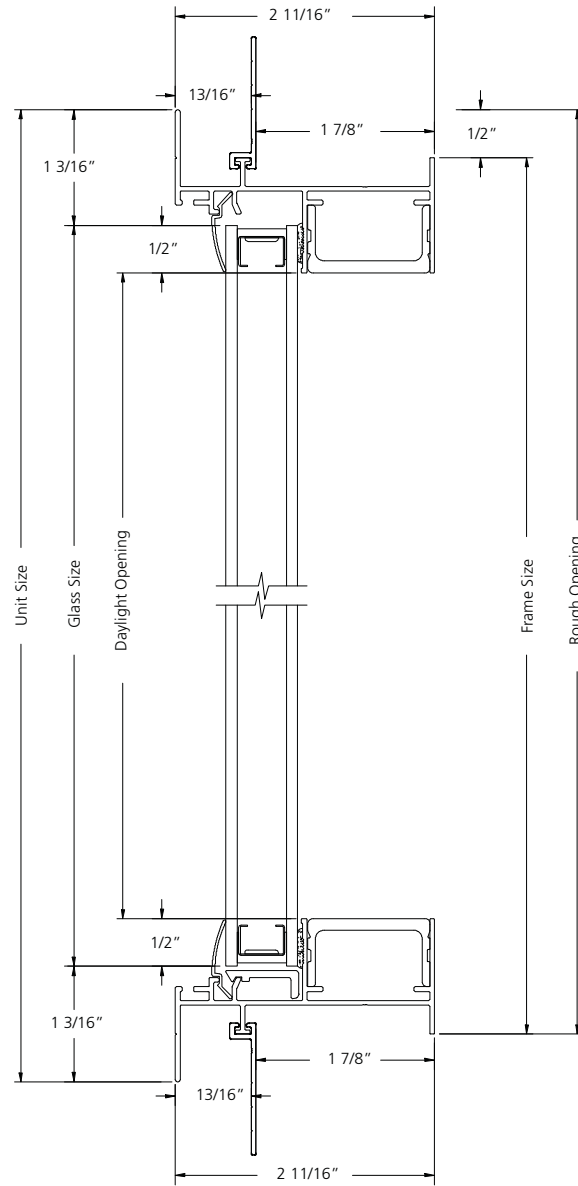
VERTICAL SECTION
