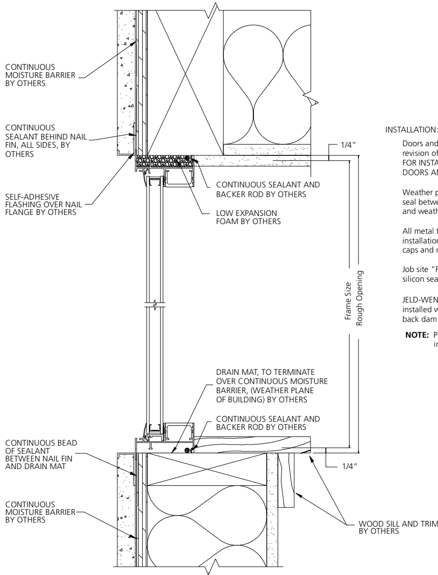
VERTICAL SECTION
