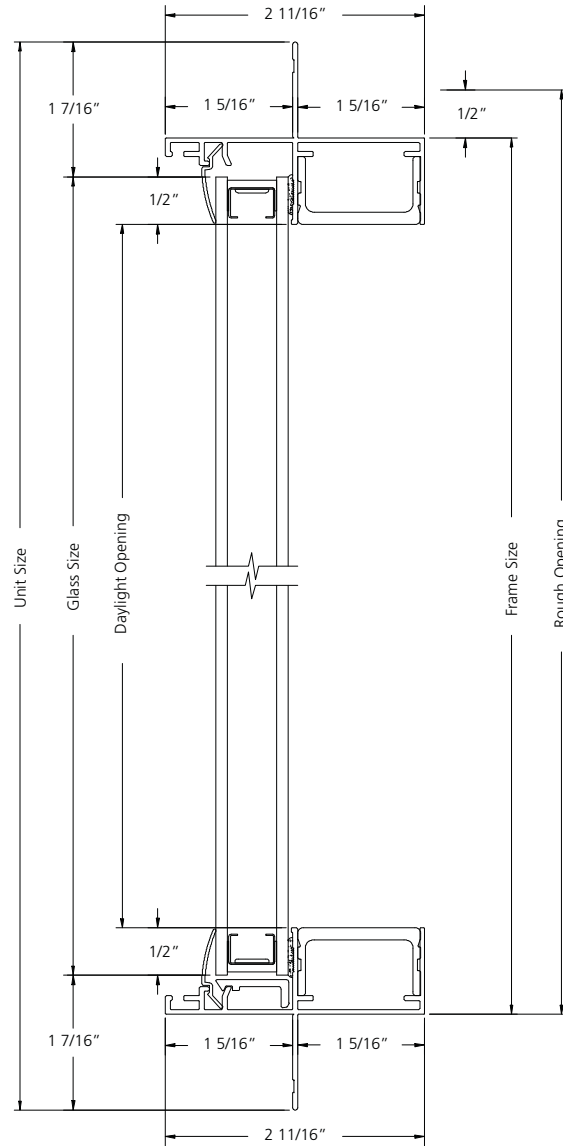
VERTICAL SECTION
