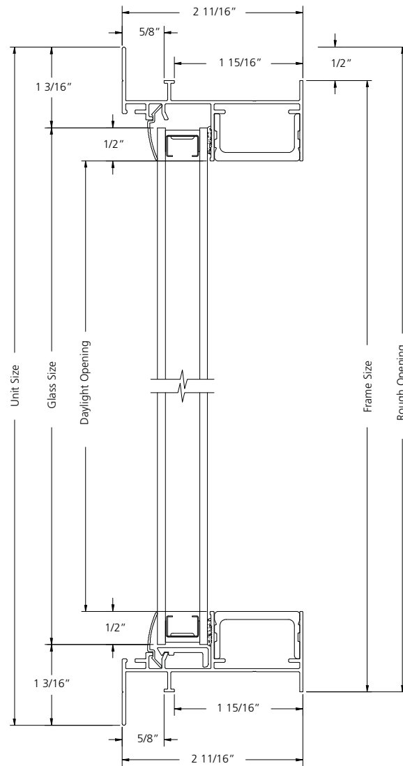
VERTICAL SECTION
