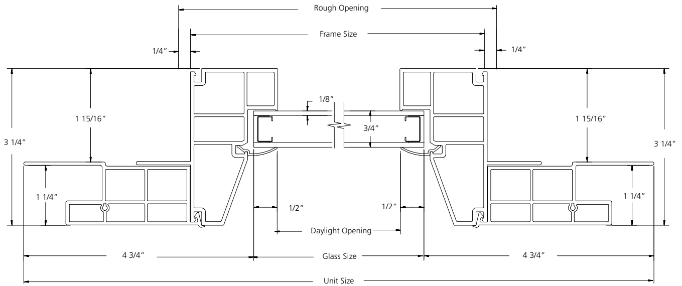
HORIZONTAL SECTION
