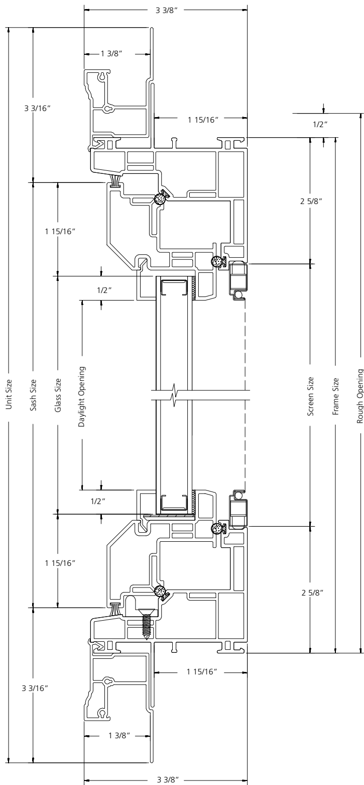
VERTICAL SECTION
