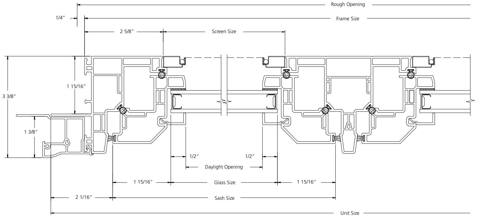
HORIZONTAL SECTION
