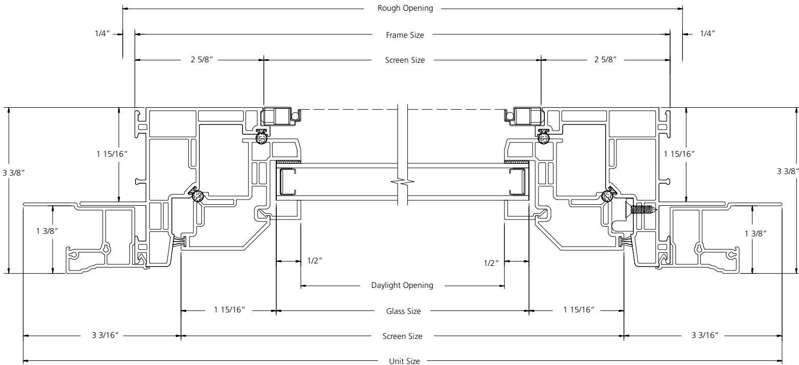
HORIZONTAL SECTION
