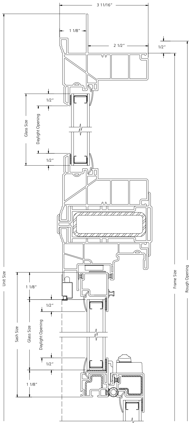
VERTICAL SECTION
