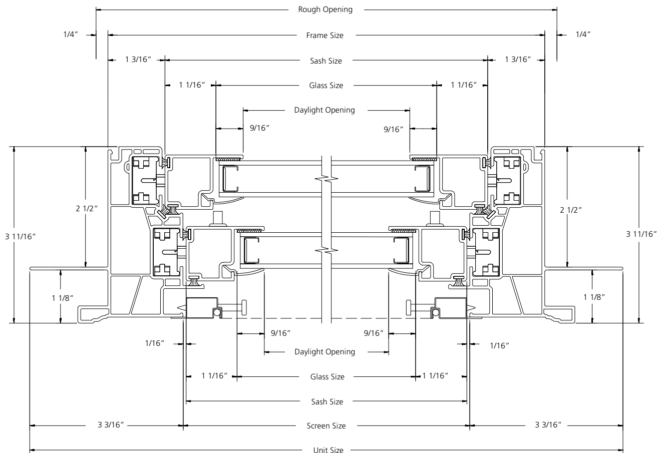
HORIZONTAL SECTION
