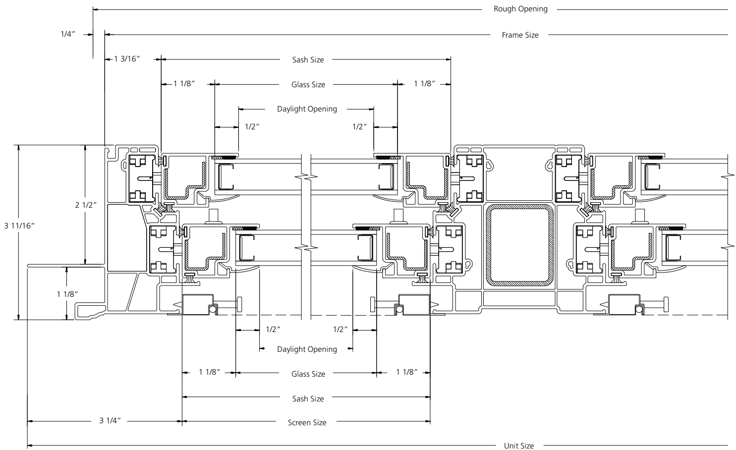
HORIZONTAL SECTION
