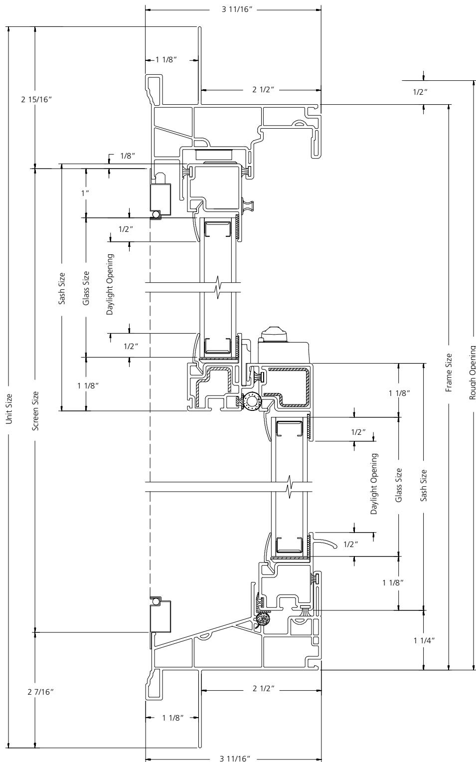
VERTICAL SECTION
