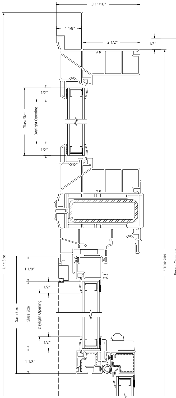
VERTICAL SECTION
