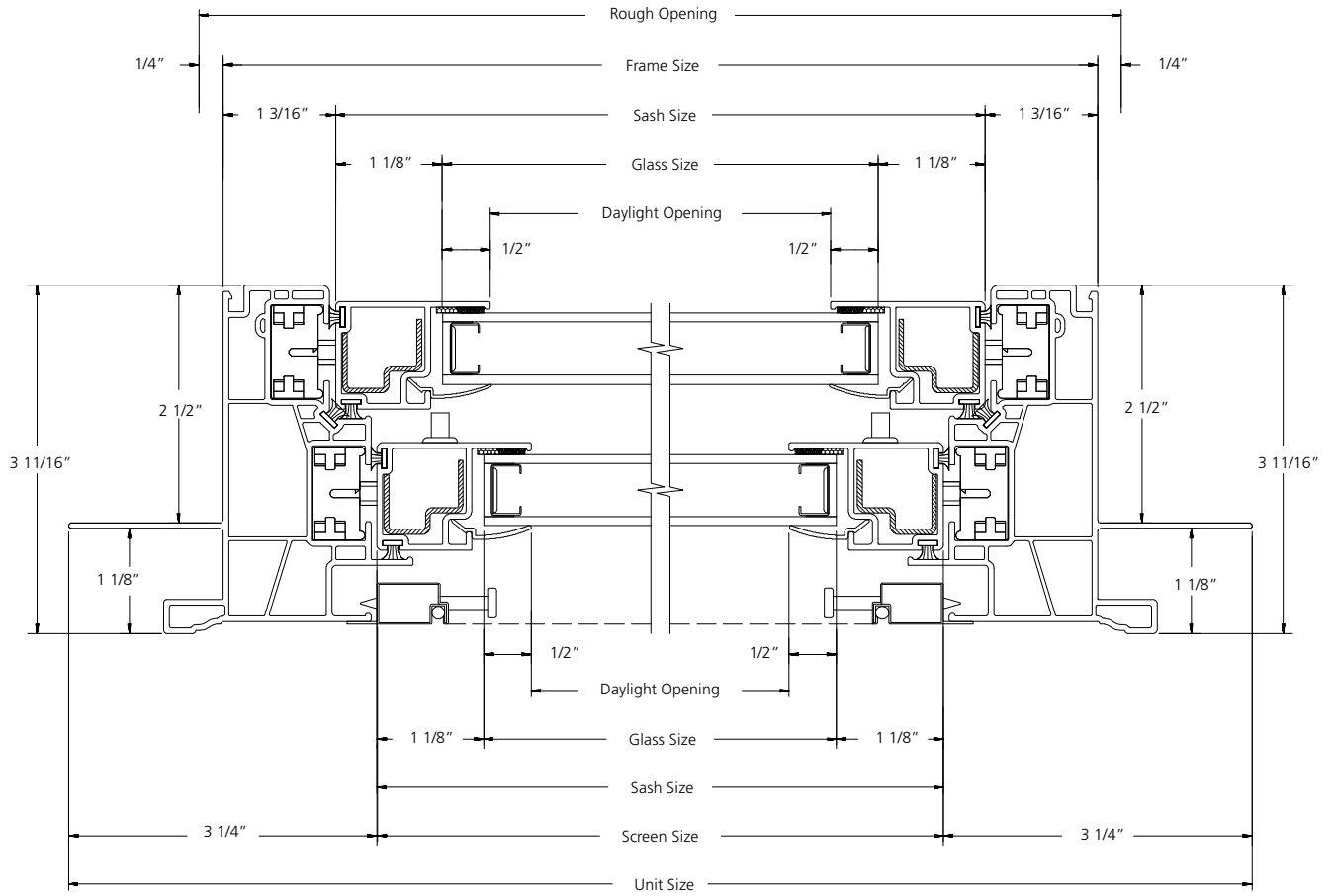
HORIZONTAL SECTION
