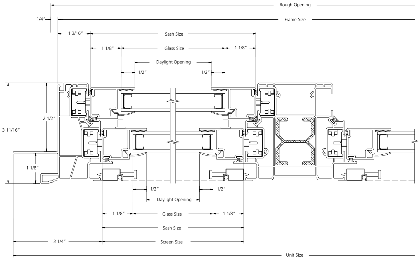
HORIZONTAL SECTION
