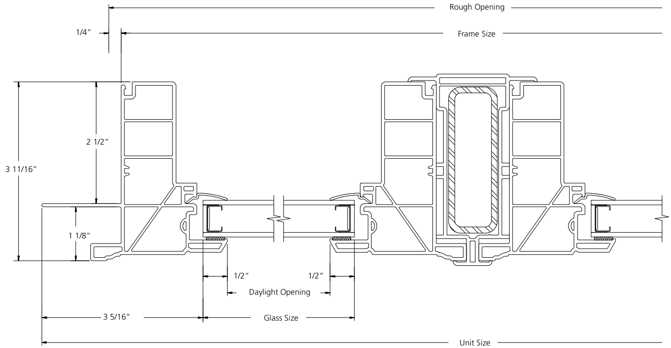
HORIZONTAL SECTION
