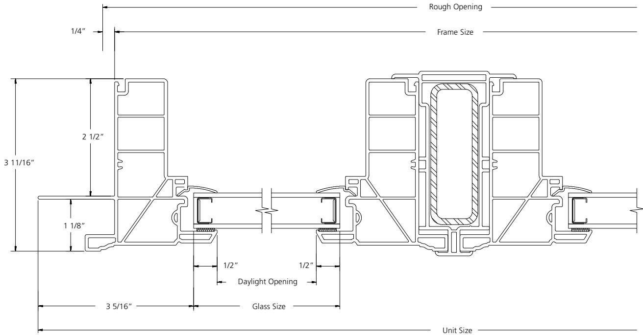
HORIZONTAL SECTION
