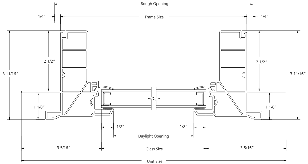
HORIZONTAL SECTION
