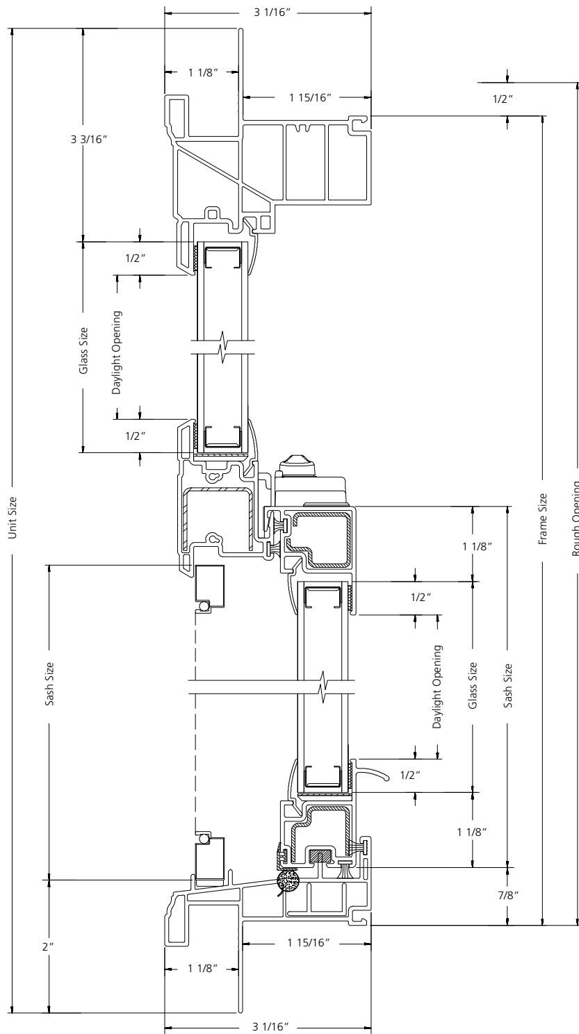
VERTICAL SECTION
