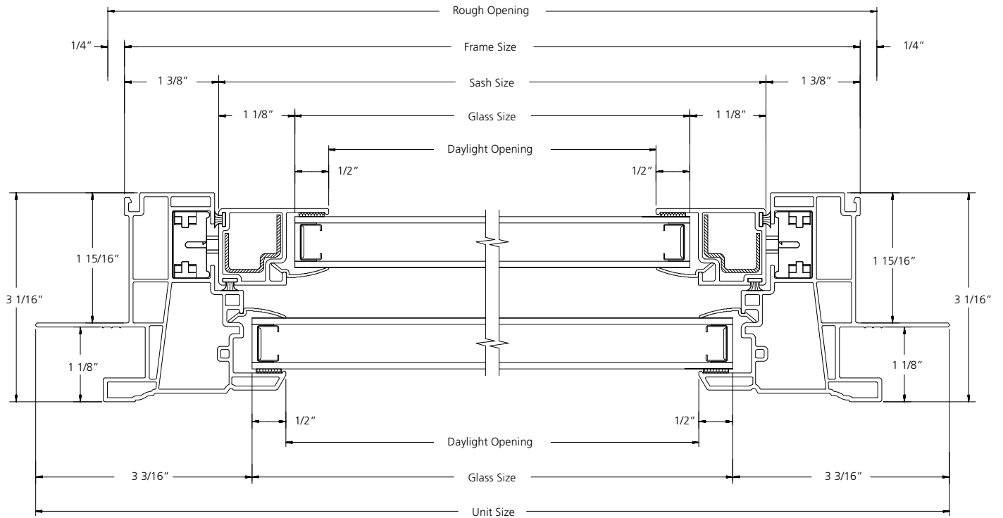
HORIZONTAL SECTION
