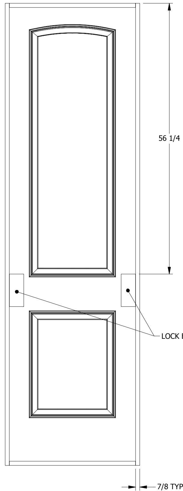
LOCK BLOCK LOCATION DOOR SKIN REMOVED
