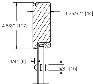
5/8" SDL BAR (PUTTY/PUTTY)
