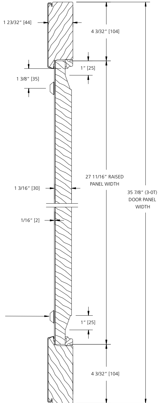
HORIZONTAL SECTION
