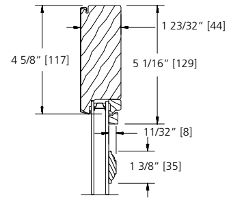
1 3/8" GRILLE BAR
