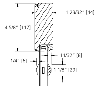
1 1/8" SDL BAR (BEAD STOP)
