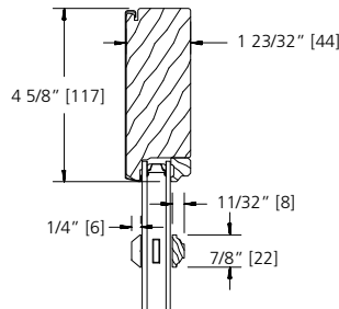
7/8" SDL BAR (PUTTY/BEAD)
