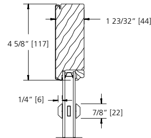
7/8" SDL BAR (PUTTY/PUTTY)
