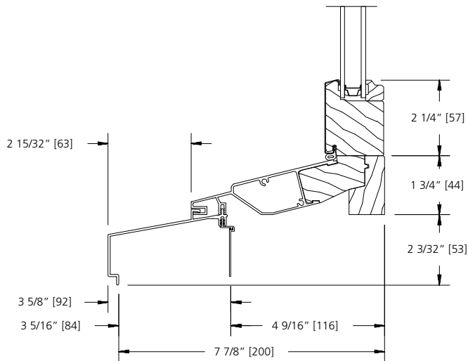
TRANSOM EXTENDED SILL NOSE (4 9/16" JAMB)
