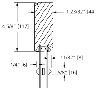
5/8" SDL BAR (PUTTY/BEAD)
