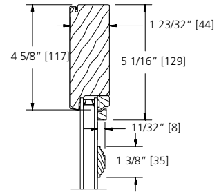
1 3/8" GRILLE BAR
