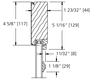
1 1/8" GRILLE BAR
