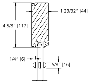
5/8" SDL BAR (PUTTY/PUTTY)
