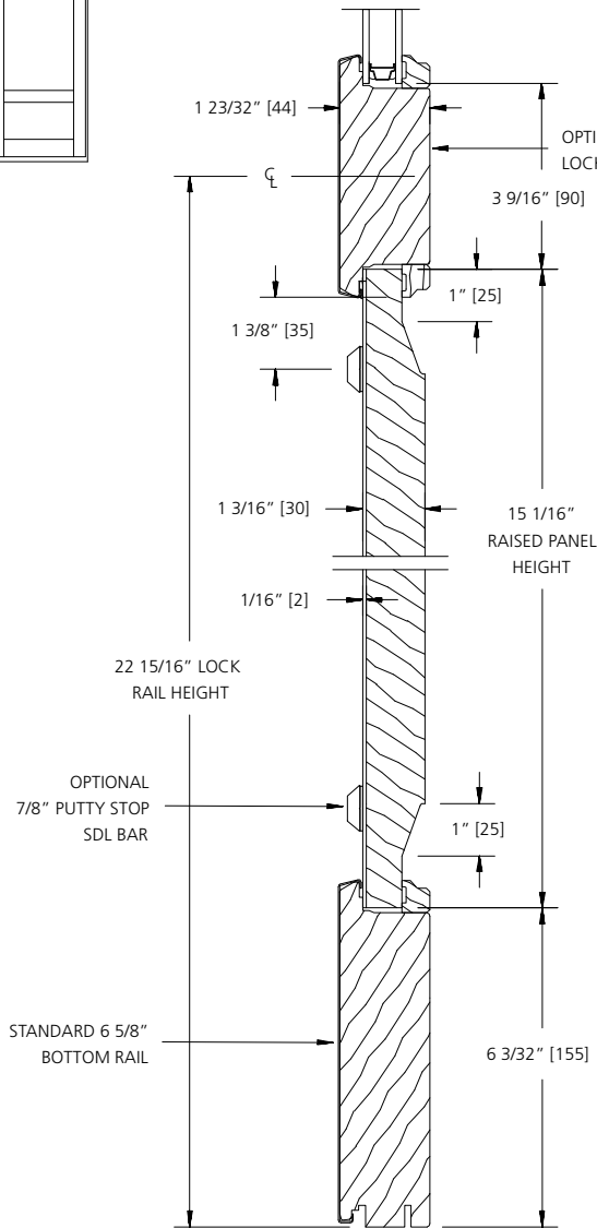
VERTICAL SECTION
