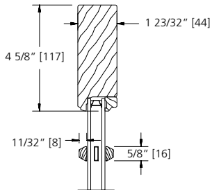
5/8" SDL BAR (PUTTY/PUTTY)
