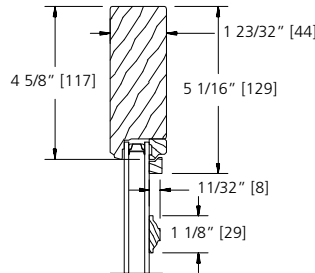
1 1/8" GRILLE BAR
