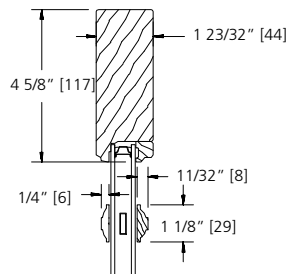
1 1/8" SDL BAR (BEAD STOP)
