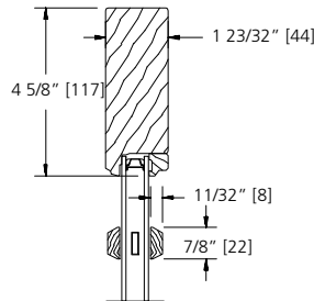
7/8" SDL BAR (PUTTY/PUTTY)
