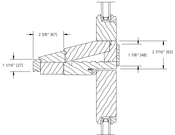
HEAD / SILL (6 9/16" JAMB)
