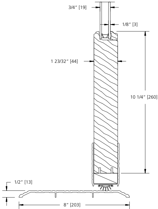
OPTIONAL 10 1/4" BOTTOM RAIL HANDICAP SILL (4 9/16 JAMB)
