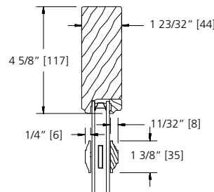
1 3/8" SDL BAR (BEAD STOP)
