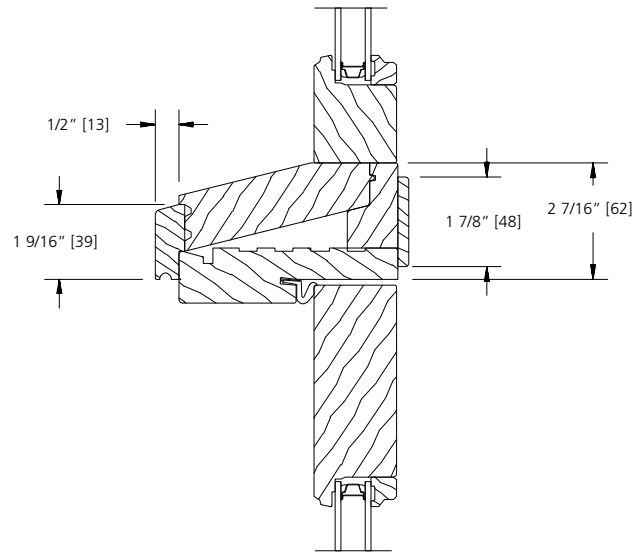
HEAD / SILL (4 9/16" JAMB)
