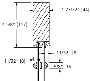
5/8" SDL BAR (PUTTY/BEAD)
