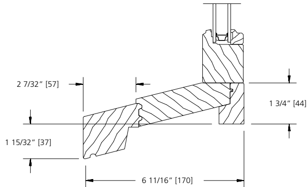
TRANSOM EXTENDED SILL NOSE (4 9/16" JAMB)
