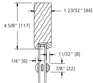
7/8" SDL BAR (BEAD STOP)
