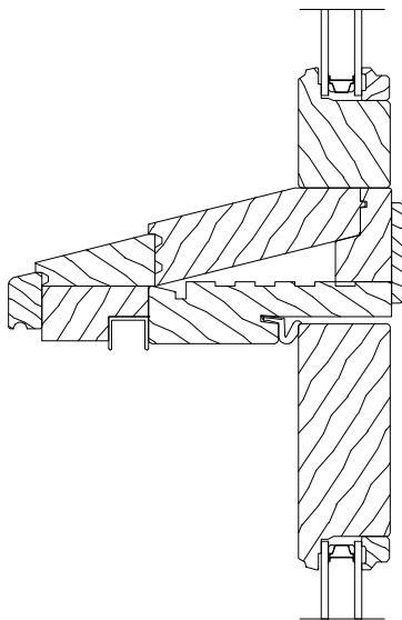
HEAD / SILL WITH SCREEN (6 9/16" JAMB)
