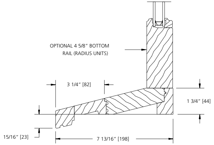
TRANSOM SILL NOSE (6 9/16" JAMB)
