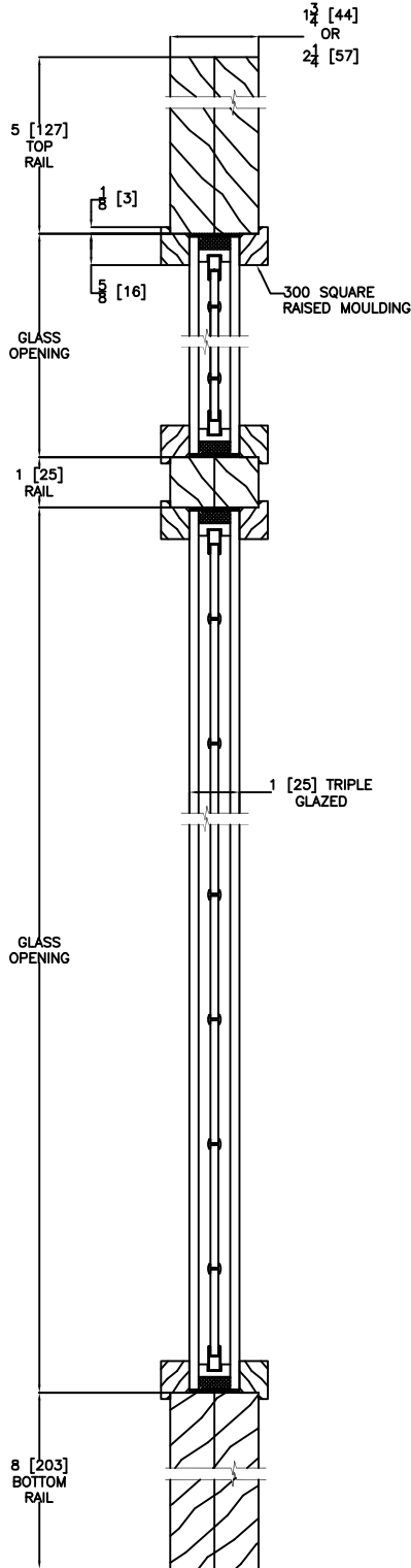
VERTICAL DOOR CROSS SECTION Triple Glazed
