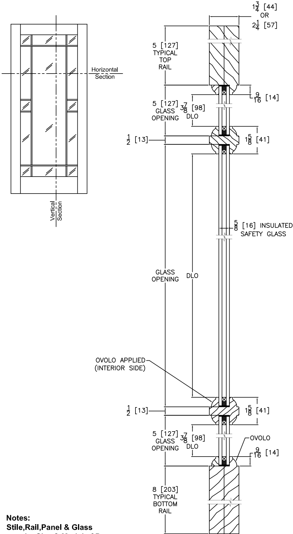
VERTICAL DOOR/SIDELIGHT CROSS SECTION Insulated Glass
