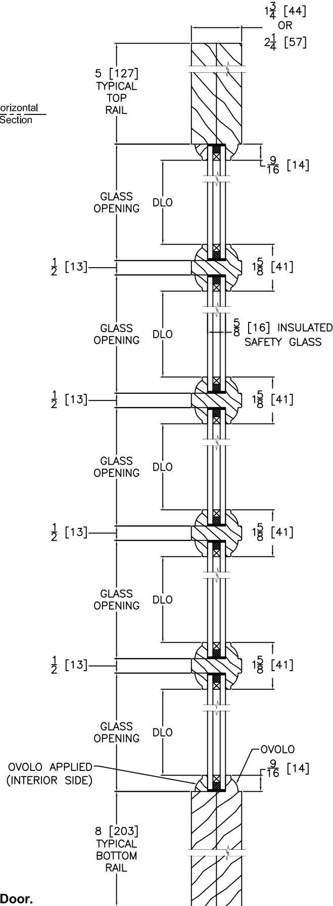
VERTICAL DOOR/SIDELIGHT CROSS SECTION Insulated Glass
