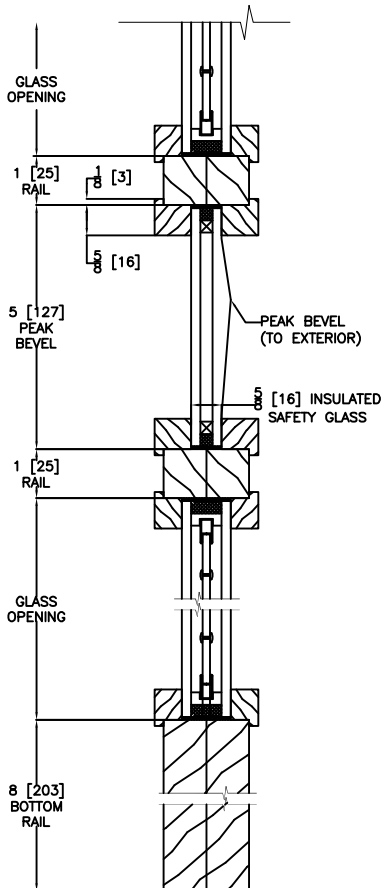
VERTICAL DOOR CROSS SECTION Insulated Glass/Triple Glazed
