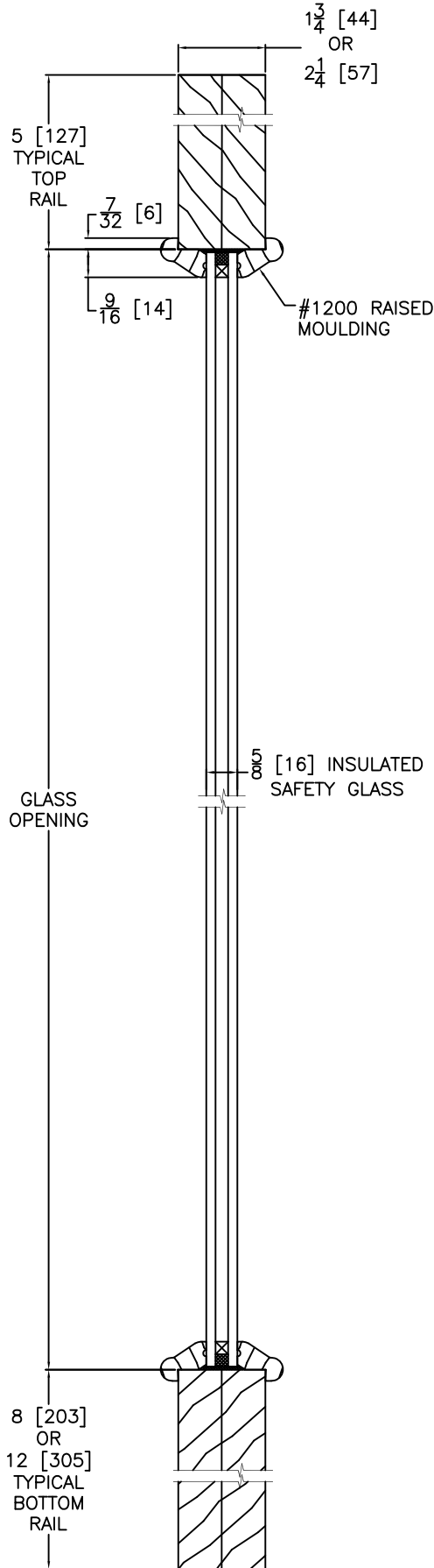
VERTICAL SIDELIGHT CROSS SECTION Insulated Glass
