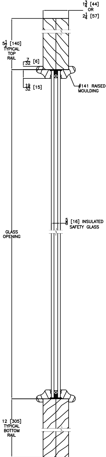
VERTICAL DOOR/SIDELIGHT CROSS SECTION Insulated Glass
