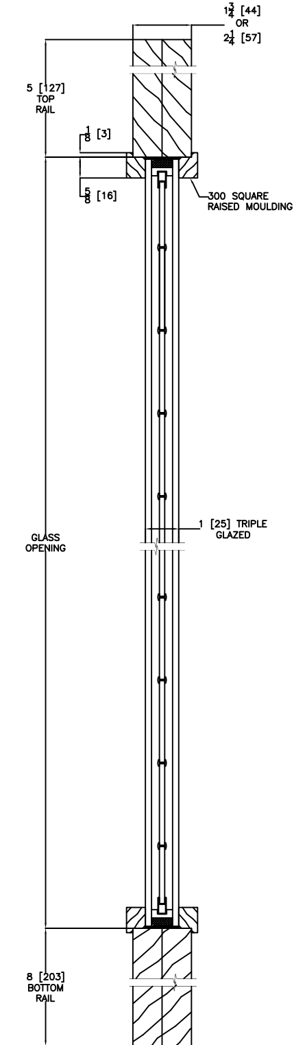
VERTICAL DOOR/SIDELIGHT CROSS SECTION Triple Glazed
