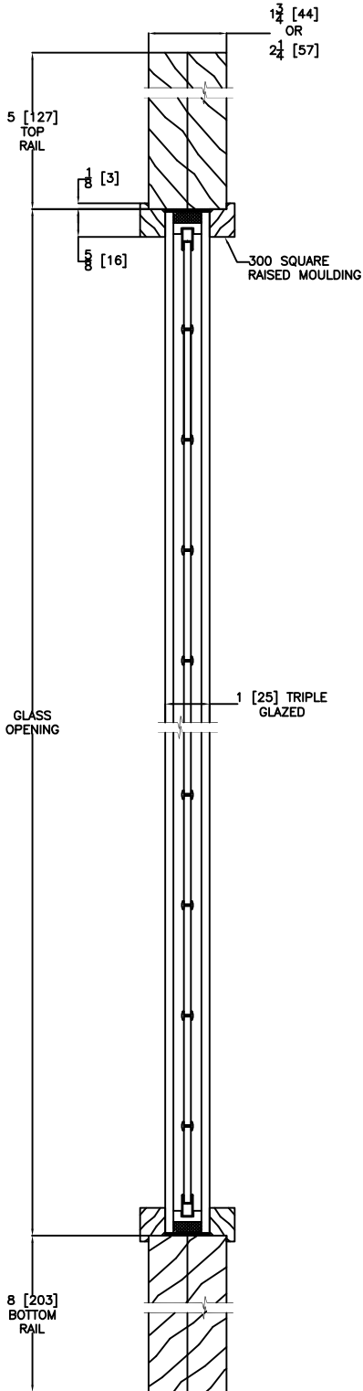
VERTICAL DOOR/SIDELIGHT CROSS SECTION Triple Glazed
