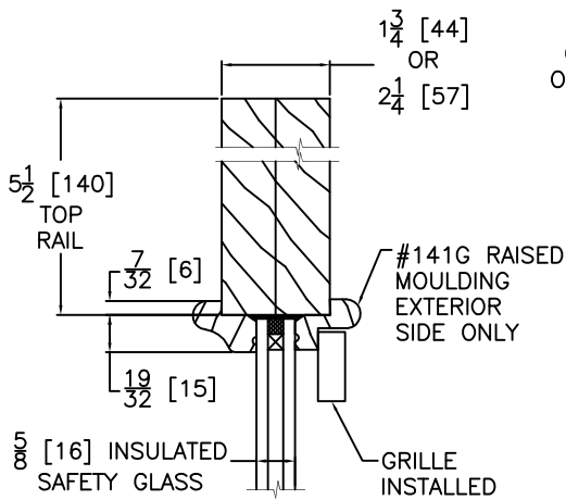
VERTICAL DOOR/SIDELIGHT CROSS SECTION For INSET Grille Application (Florence & Rustic Grilles are Stile-Mounted)
