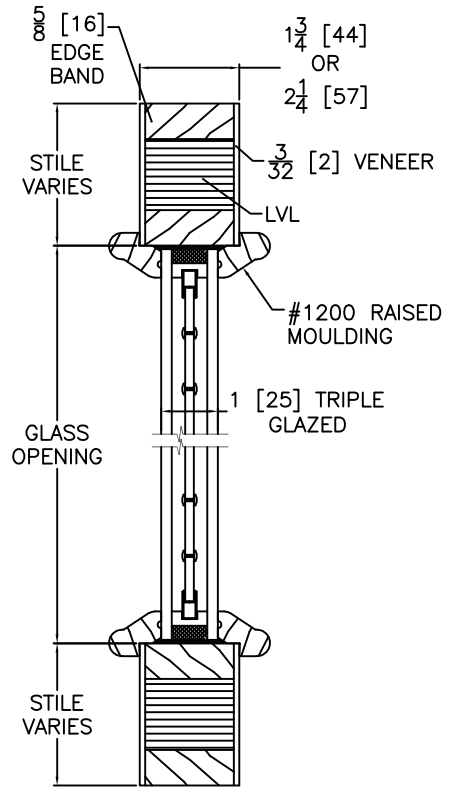
HORIZONTAL SIDELIGHT CROSS SECTION Triple Glazed Engineered Stile Option (Upon Request or Doors >3'-6" X 8'-0")
