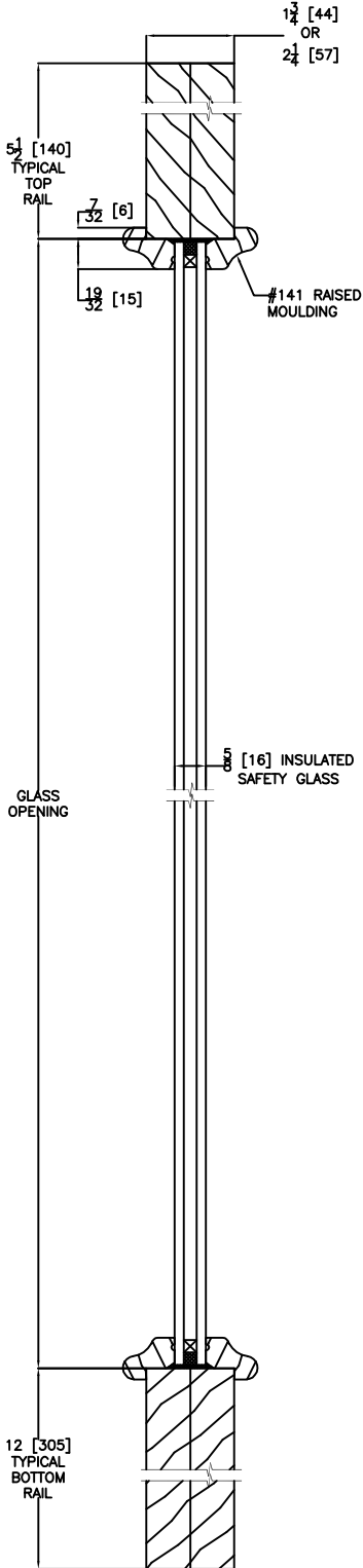
VERTICAL DOOR/SIDELIGHT CROSS SECTION Insulated Glass
