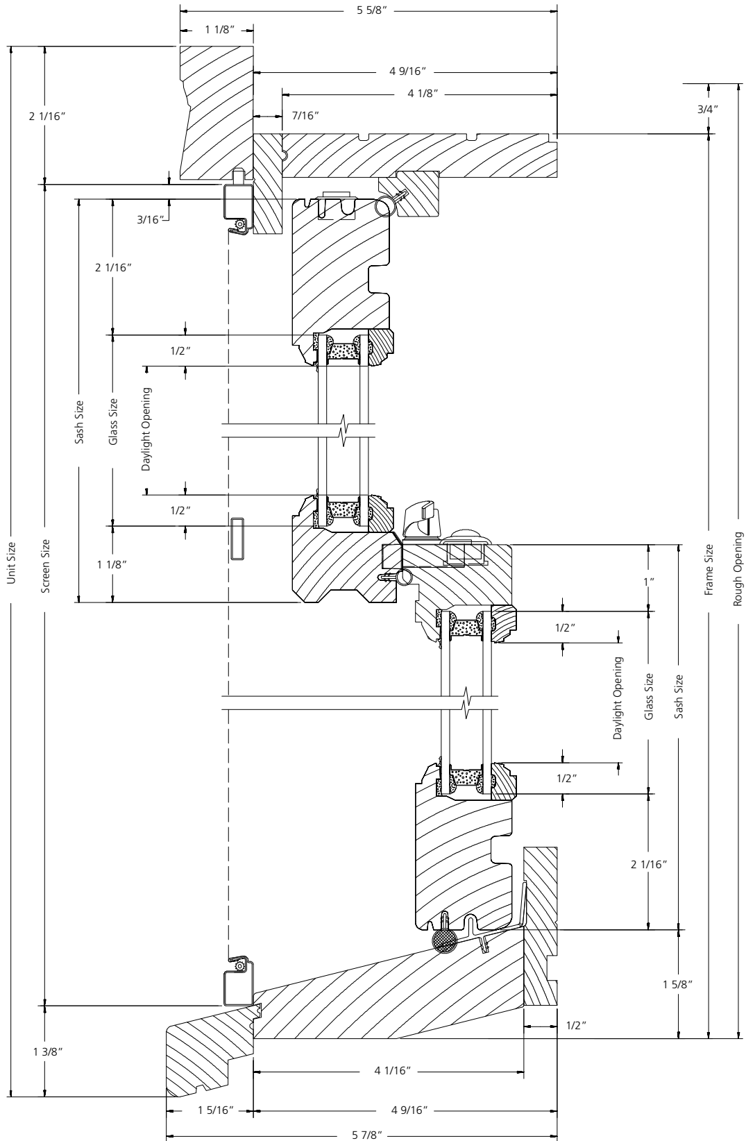
VERTICAL SECTION
