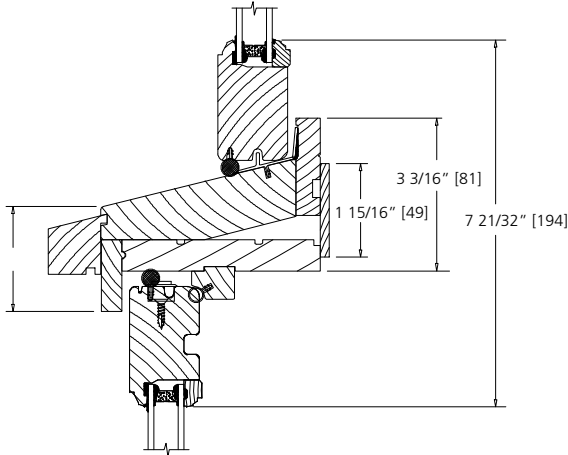
OPERATING DOUBLE-HUNG WITH FIXED TRANSOM
