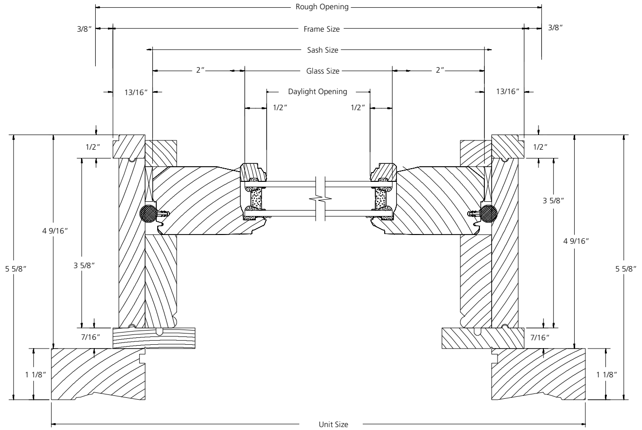
HORIZONTAL SECTION
