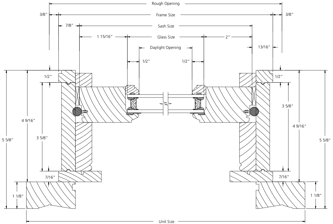
HORIZONTAL SECTION
