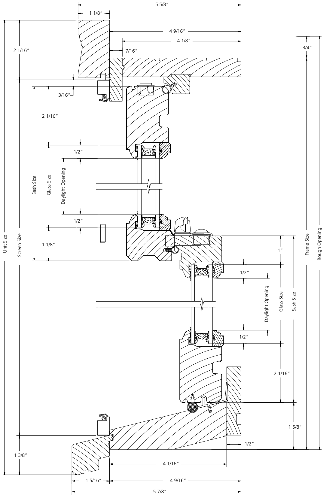
VERTICAL SECTION
