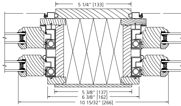
TWIN OPERATING DOUBLE-HUNG WITH 4" SOLID SPREAD MULLION
