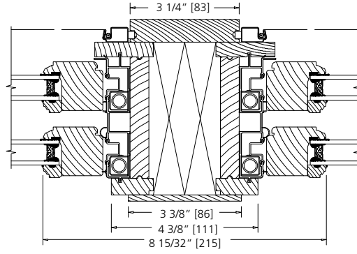
TWIN OPERATING DOUBLE-HUNG WITH 2" SOLID SPREAD MULLION
