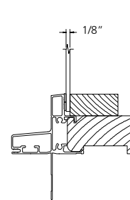
LAMINATED INSULATED SINGLE GLASS
