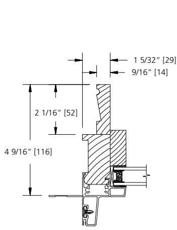
4 9/16" WALL 9/16" JAMB THICKNESS (OPTION)
