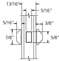
7/8" PUTTY/BEAD SDL
