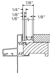
LAMINATED INSULATED TINTED GLASS
