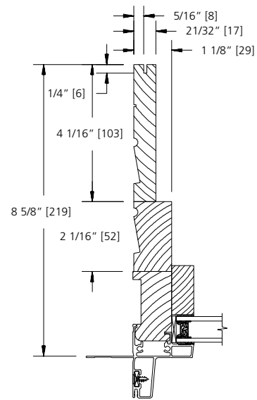
8 5/8" WALL 5/4-4/4 STACKED KERFED JAMB OPTION
