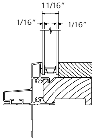
STANDARD INSULATED GLASS
