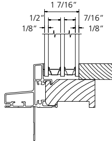
5/32" TRIPANE INSULATED GLASS
