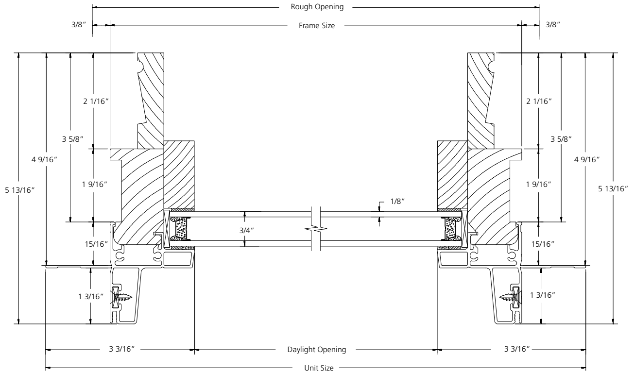
HORIZONTAL SECTION
