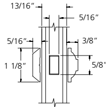
1 1/8" PUTTY/BEAD SDL
