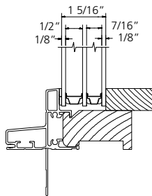
DS TRIPANE INSULATED GLASS
