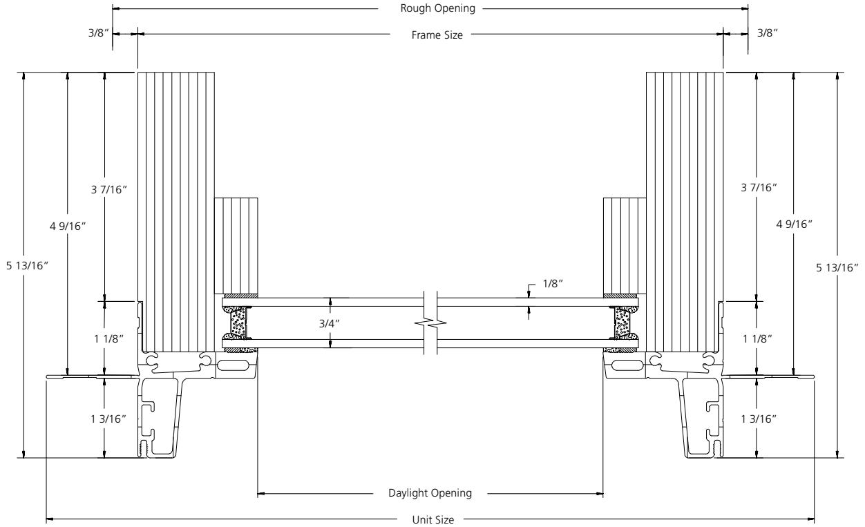
HORIZONTAL SECTION
