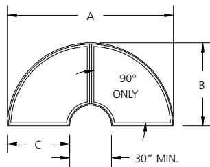
INVERTED HALF ROUND - TWIN TYPE BI - 2
