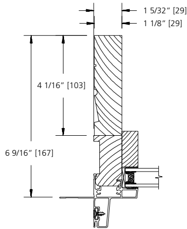
6 9/16" WALL 5/4 JAMB THICKNESS (OPTION)
