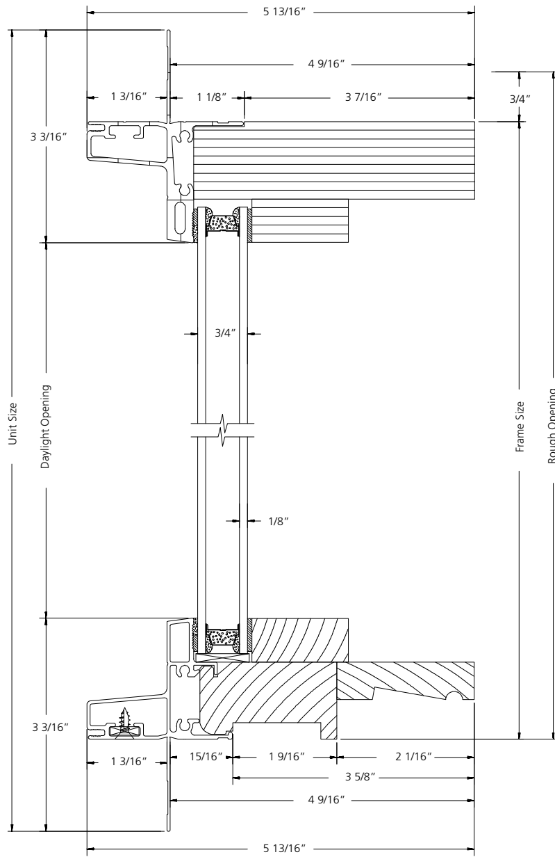
VERTICAL SECTION
