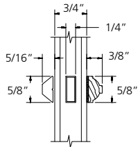
5/8" PUTTY/BEAD SDL
