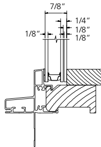
LAMINATED INSULATED CLEAR OR LOW E GLASS
