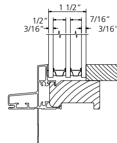
3/16" TRIPANE INSULATED GLASS
