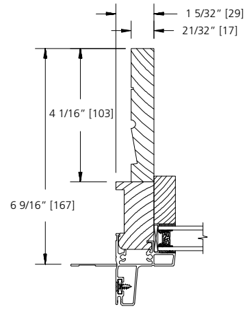
6 9/16" WALL 4/4 JAMB THICKNESS (STANDARD)
