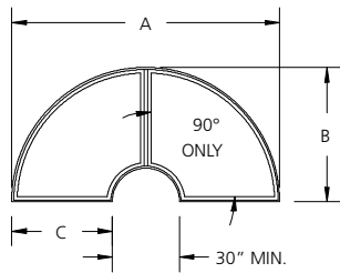
TYPE BI - 2 INVERTED HALF ROUND - TWIN
