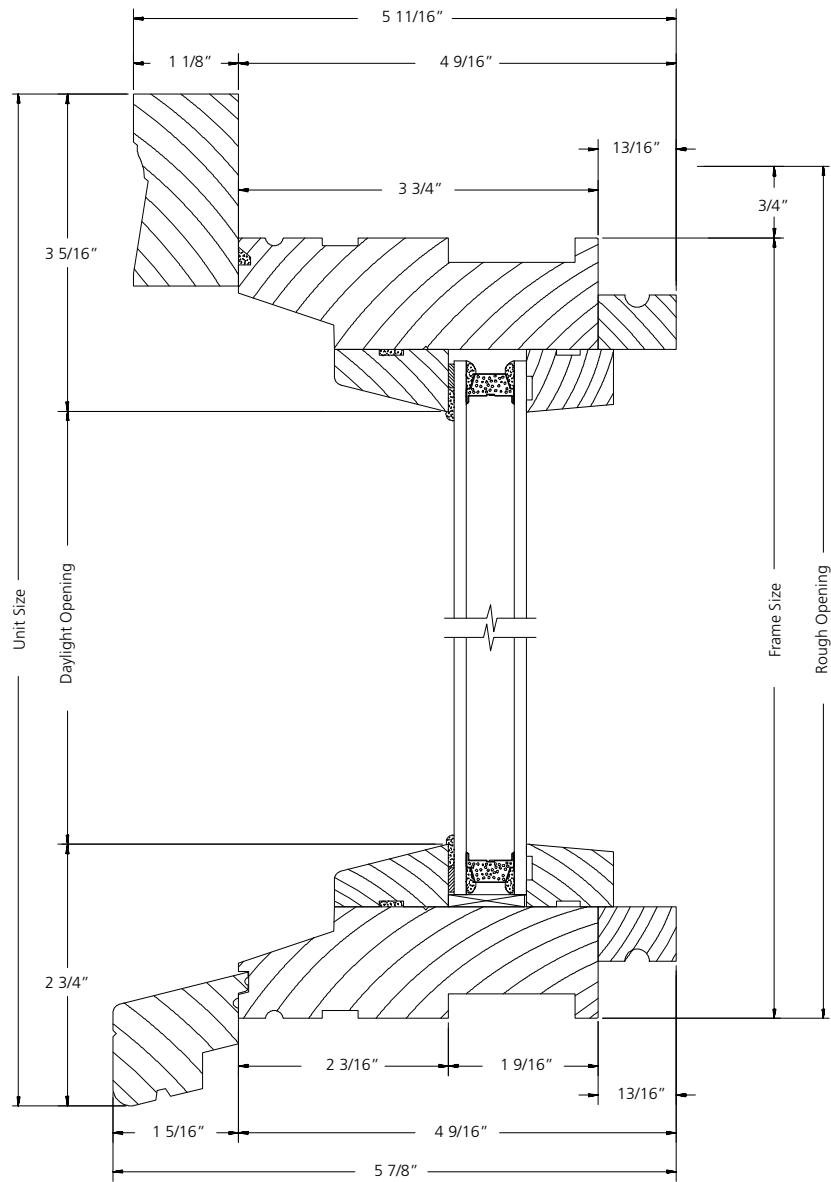
VERTICAL SECTION
