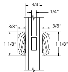
1 1/8" PUTTY/PUTTY SDL
