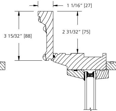
RG 3 CASING
