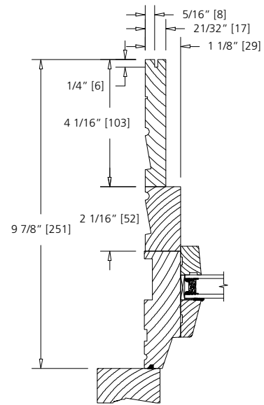
9 7/8" WALL
