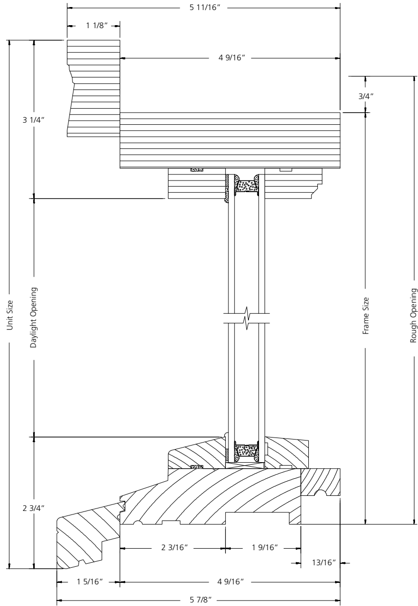
VERTICAL SECTION
