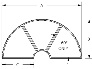
TYPE BI - 3 INVERTED HALF ROUND - TRIPLE
