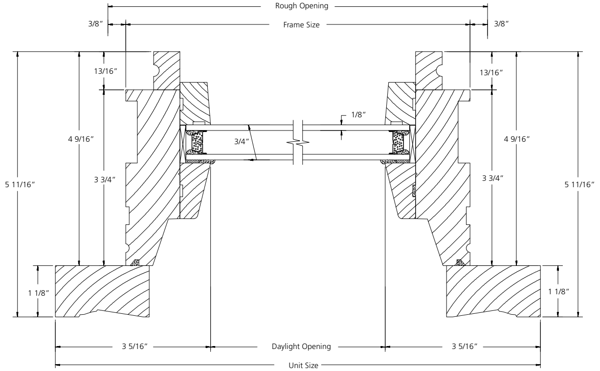
HORIZONTAL SECTION
