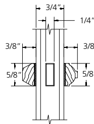
5/8" PUTTY/BEAD SDL
