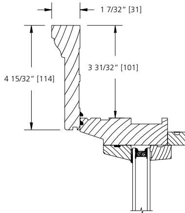
1 X 4 BACK BAND
