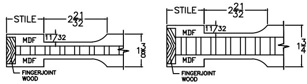
SQUARE STICKING WITH "B1" SCOOP PANEL
