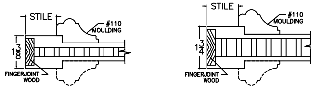
#110 MOULDING WITH "C1" FLAT PANEL
