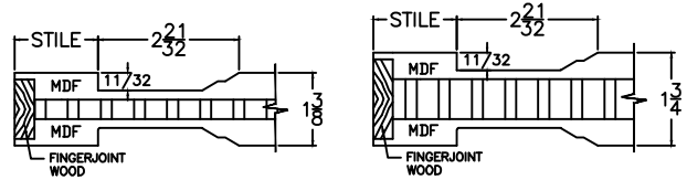
SQUARE STICKING WITH "D1" DOUBLE HIP
