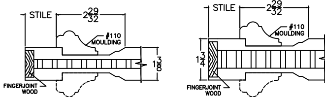
#110 MOULDING WITH "D1" DOUBLE HIP
