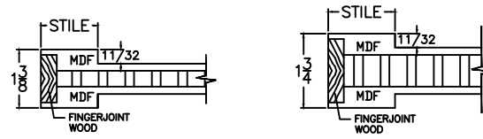
SQUARE STICKING WITH "C1" FLAT PANEL
