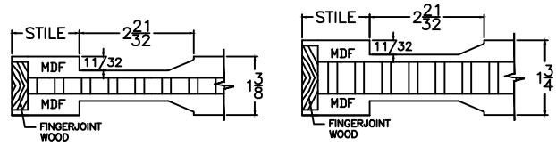
SQUARE STICKING WITH "A1" SINGLE HIP
