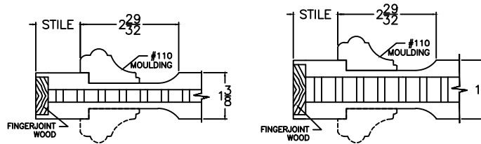
#110 MOULDING WITH "B1" SCOOP PANEL
