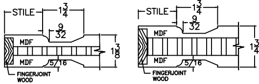
OG STICKING WITH "A1" SINGLE HIP
