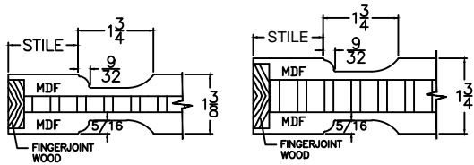
OG STICKING WITH "B1" SCOOP PANEL
