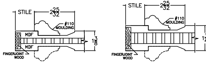
#110 MOULDING WITH "A1" SINGLE HIP
