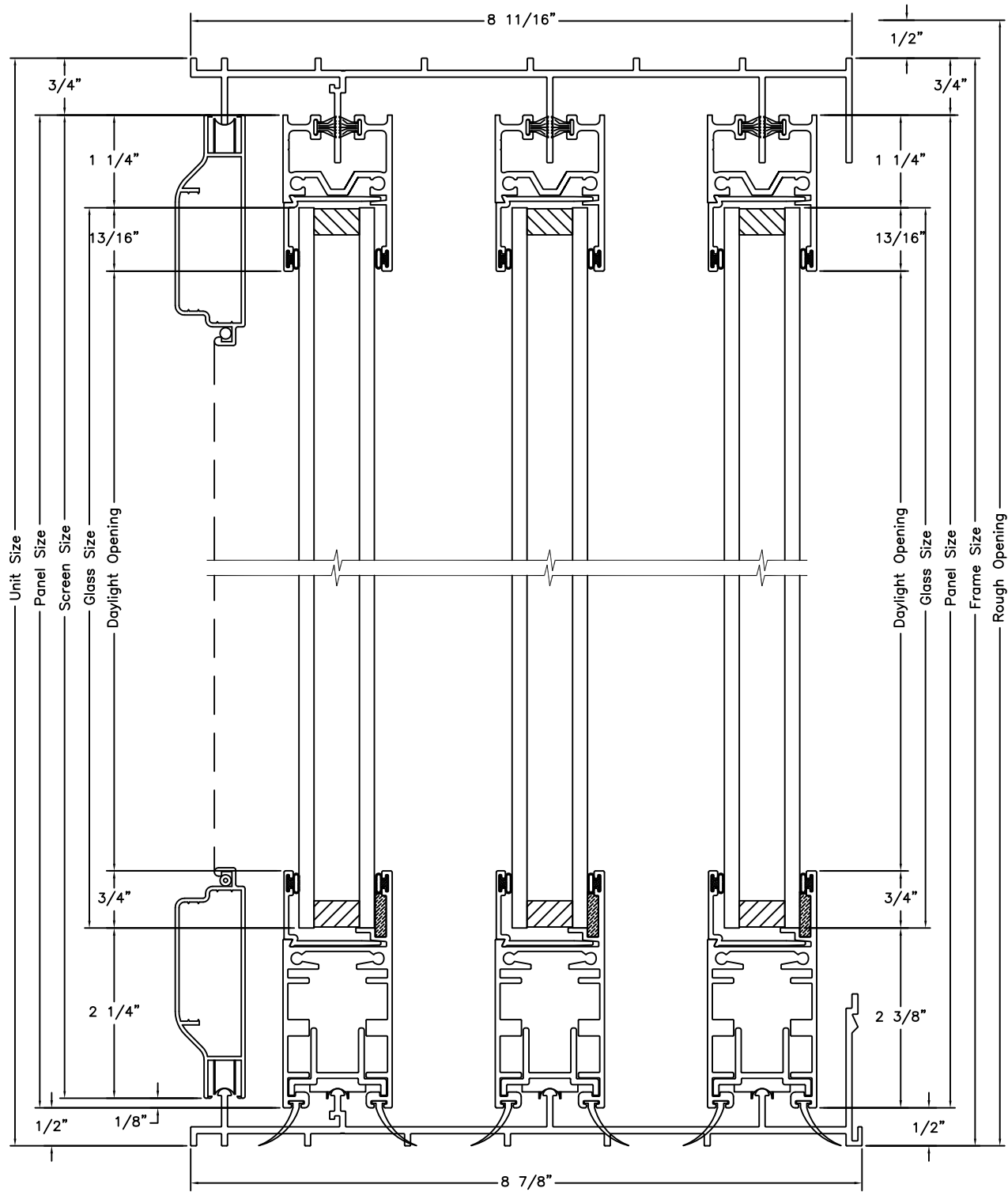
Vertical Section
