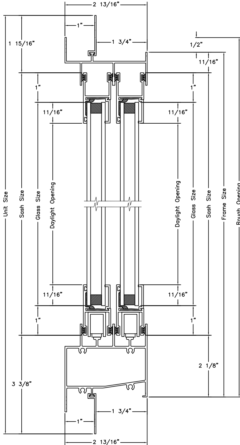
Vertical Section
