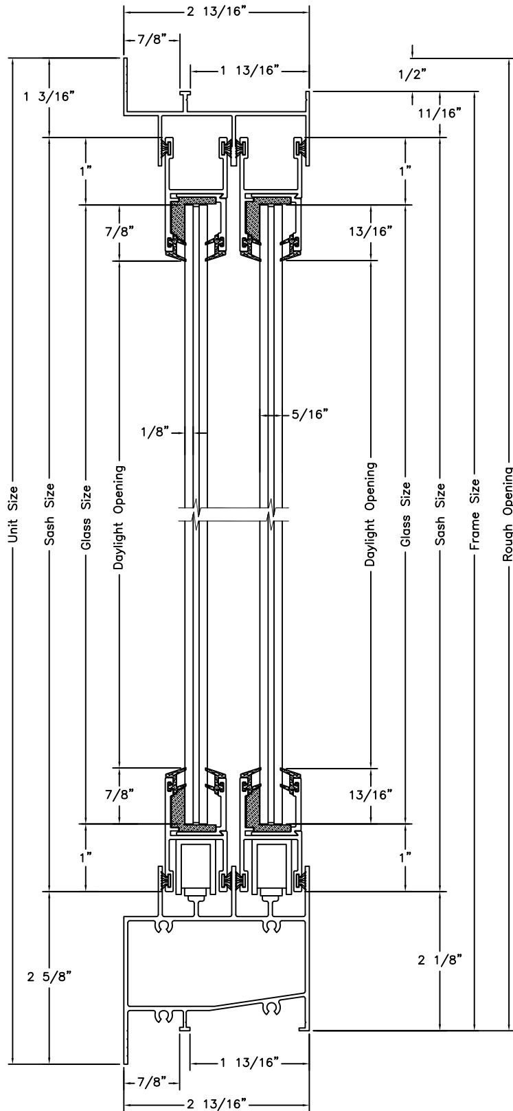
Vertical Section
