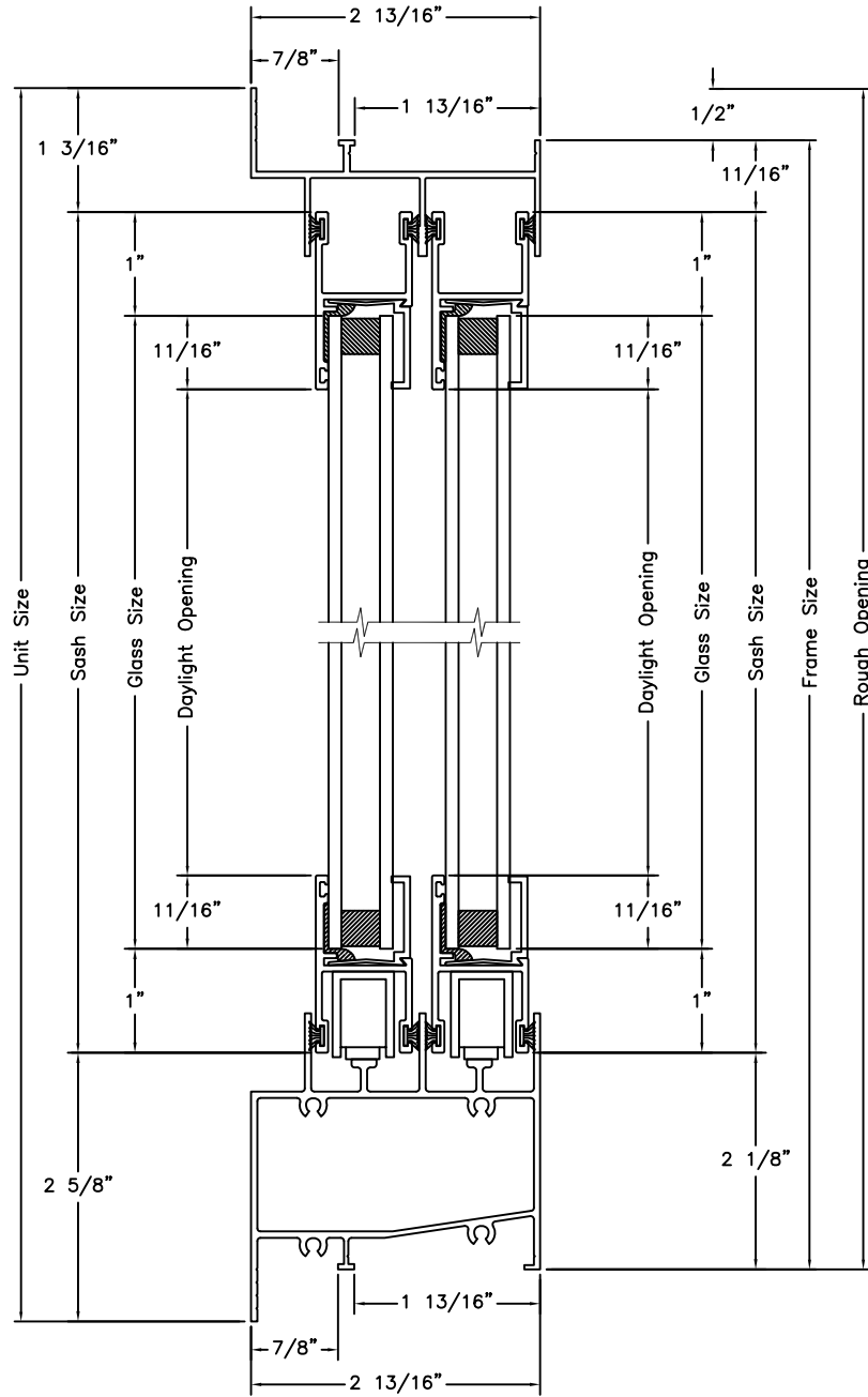
Vertical Section
