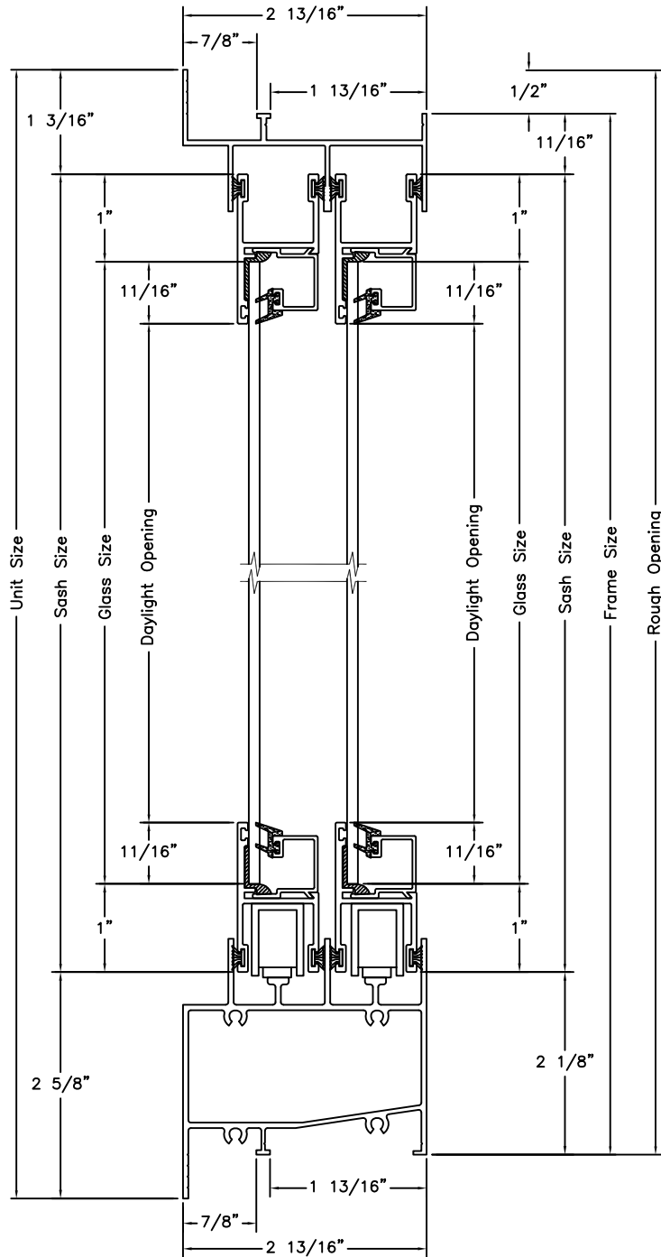
Vertical Section
