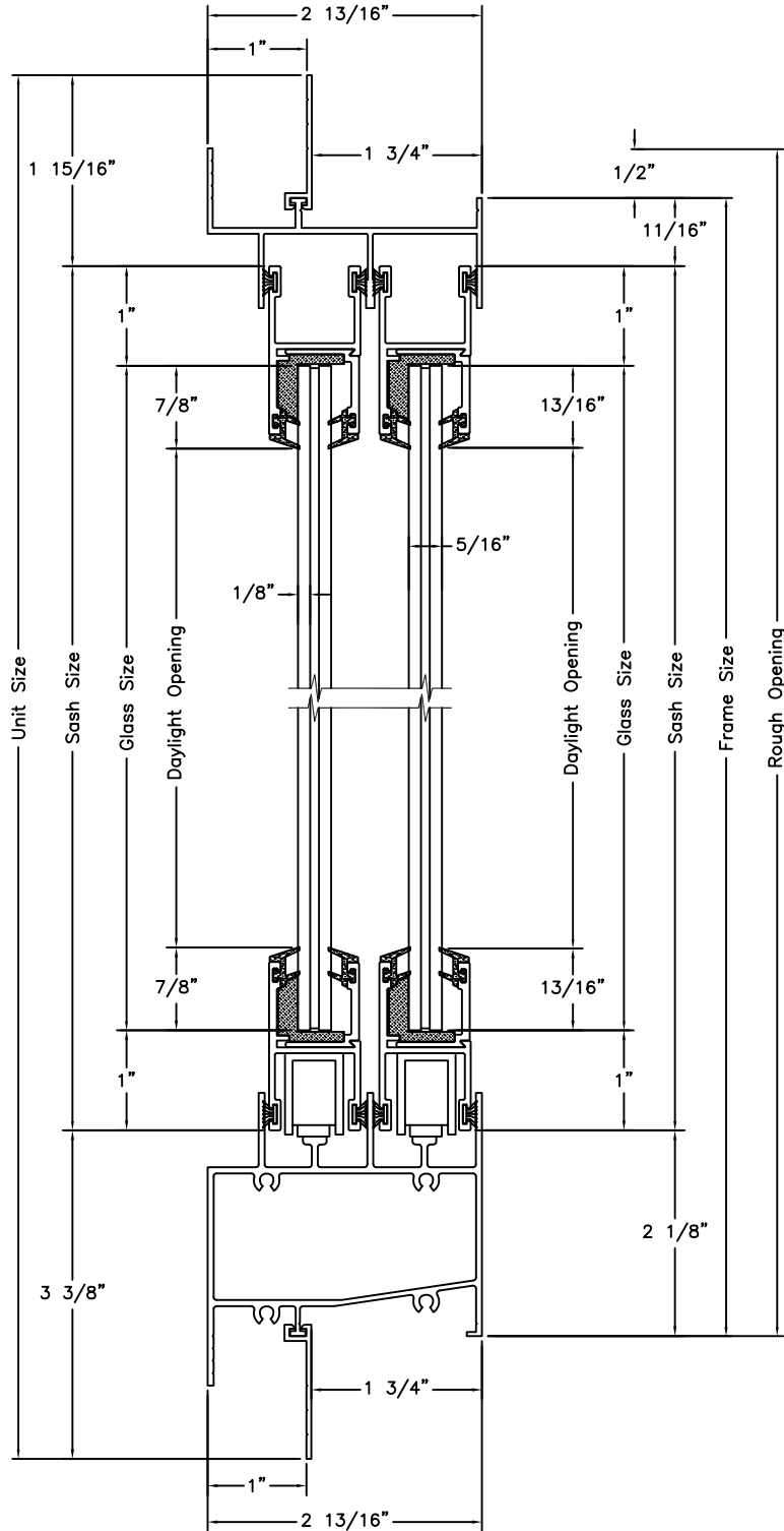
Vertical Section
