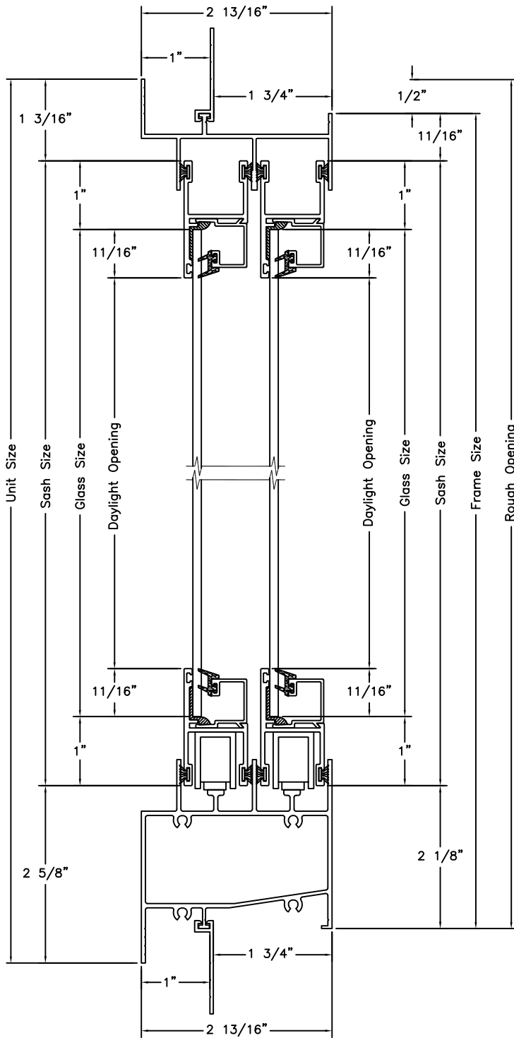
Vertical Section
